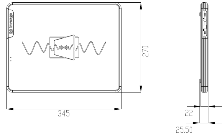
Figure 3.1 XC-RF855 reader
