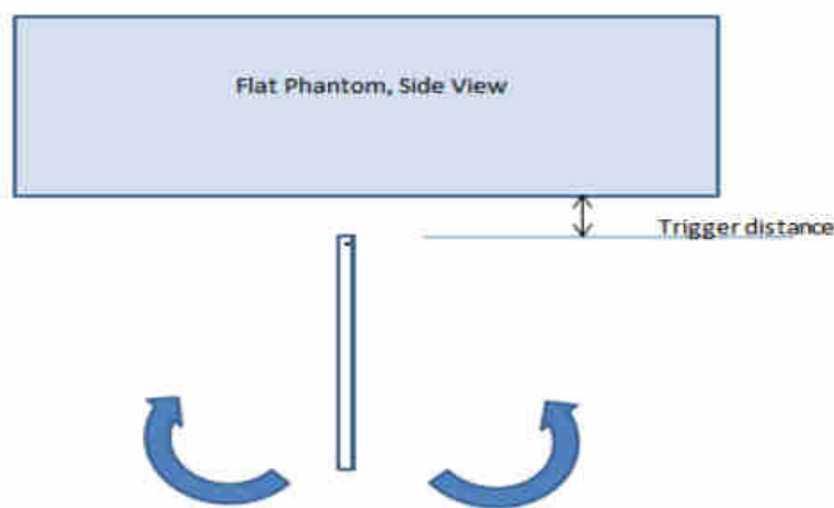
Proximity Sensor Coverage Assesment(Bottom Side)
