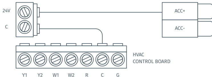
Option 2 Internally powered wiring
