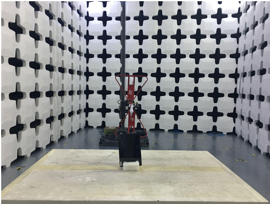
2. Radiated Emissions (Part 15C&E) (30MHz-1GHz)
