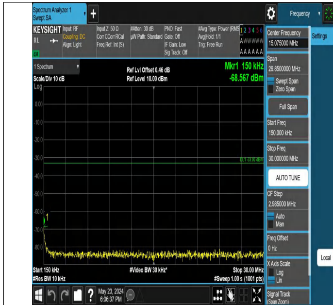
Band4_10MHz_QPSK_20000_1RB#49_0.15~30_0.15~30
