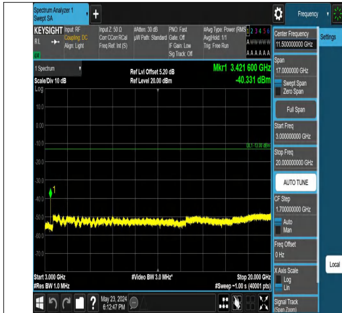
Band4_15MHz_QPSK_20025_1RB#0_3000~20000_3000~20000
