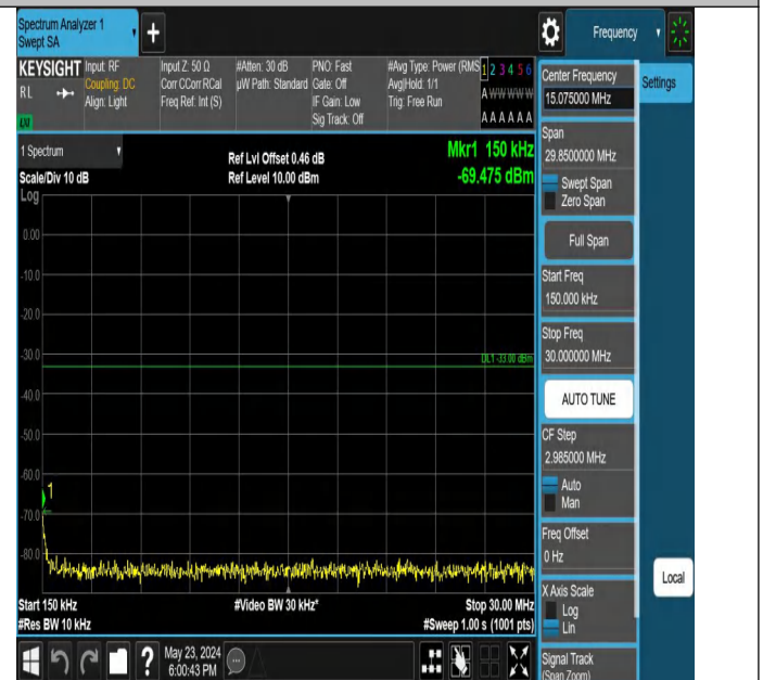
Band4_5MHz_QPSK_20175_1RB#0_0.15~30_0.15~30
