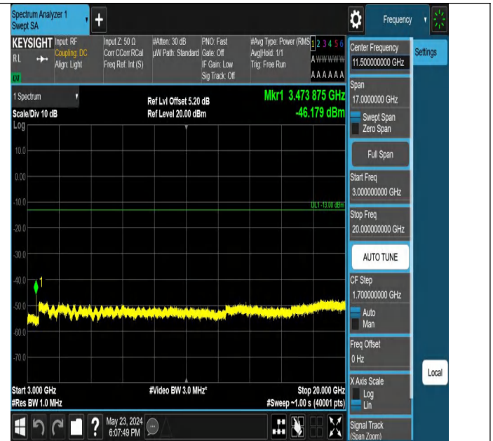
Band4_10MHz_QPSK_20175_1RB#49_3000~20000_3000~20000
