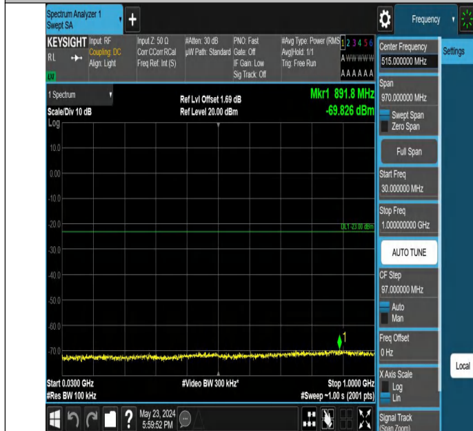
Band4_5MHz_QPSK_19975_1RB#0_30~1000_30~1000
