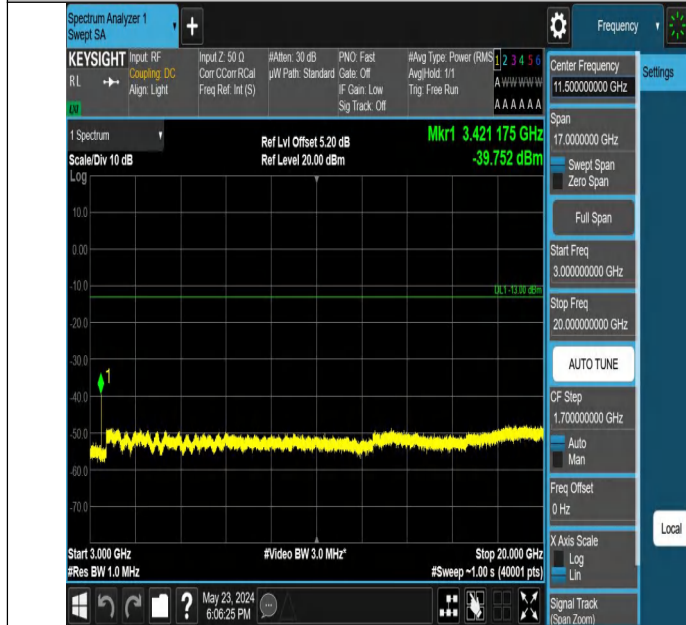
Band4_10MHz_QPSK_20000_1RB#0_3000~20000_3000~20000
