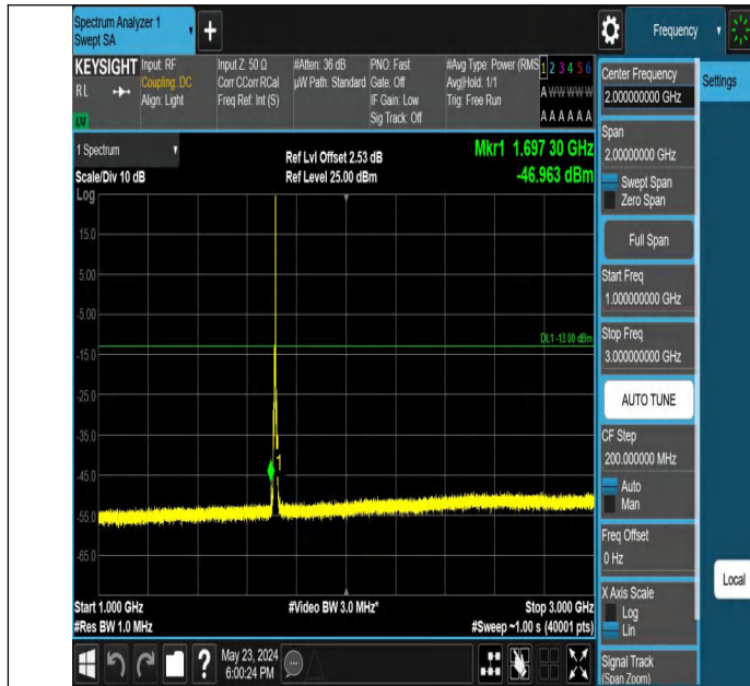
Band4_5MHz_QPSK_19975_1RB#24_1000~3000_1000~3000
