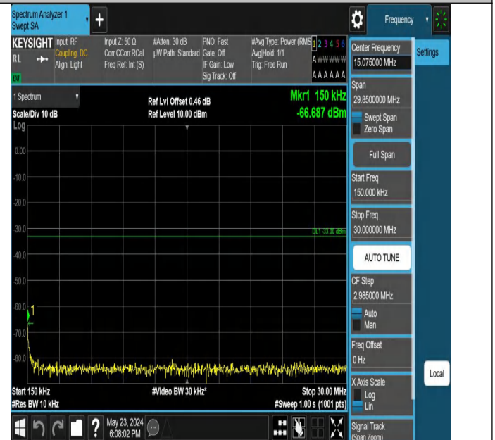
Band4_10MHz_QPSK_20350_1RB#0_0.15~30_0.15~30
