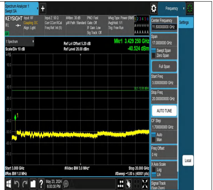
Band4_5MHz_QPSK_19975_1RB#24_3000~20000_3000~20000
