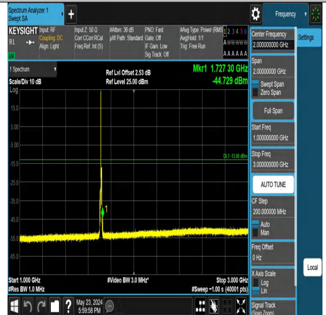
Band4_5MHz_QPSK_19975_1RB#0_1000~3000_1000~3000
