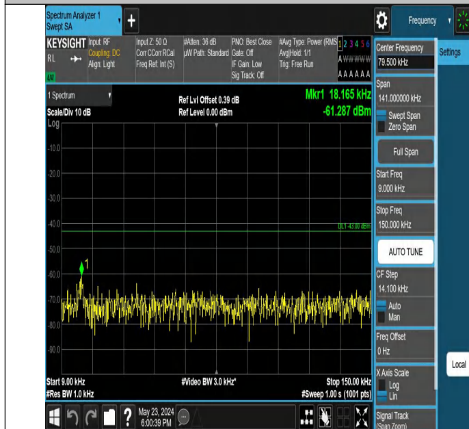
Band4_5MHz_QPSK_20175_1RB#0_0.009~0.15_0.009~0.15
