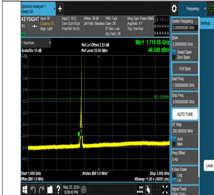
Band4_10MHz_QPSK_20350_1RB#49_1000~3000_1000~3000
