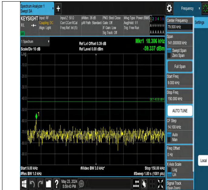
Band4_5MHz_QPSK_19975_1RB#0_0.009~0.15_0.009~0.15
