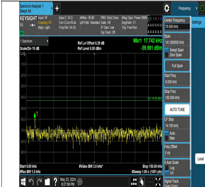
Band4_10MHz_QPSK_20350_1RB#0_0.009~0.15_0.009~0.15
