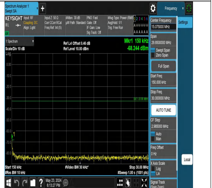
Band4_15MHz_QPSK_20175_1RB#0_0.15~30_0.15~30
