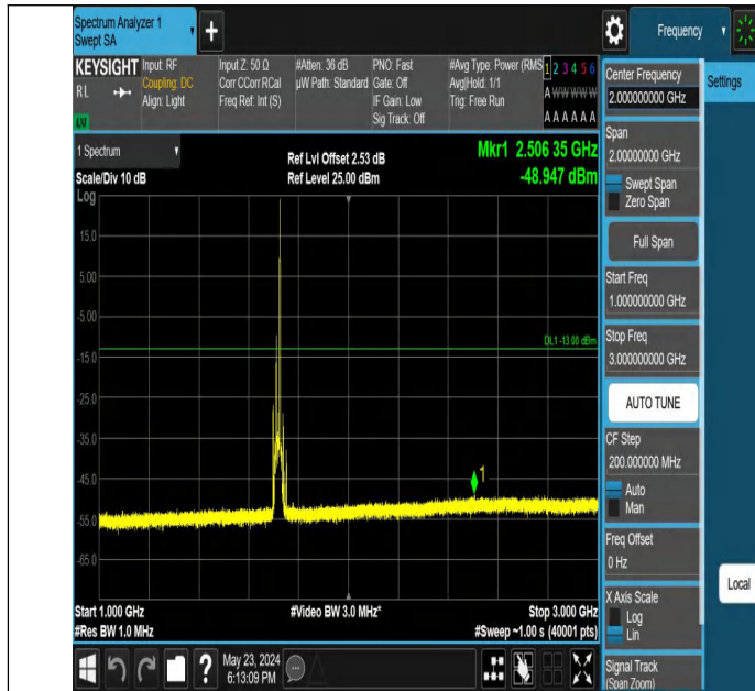
Band4_15MHz_QPSK_20025_1RB#74_1000~3000_1000~3000
