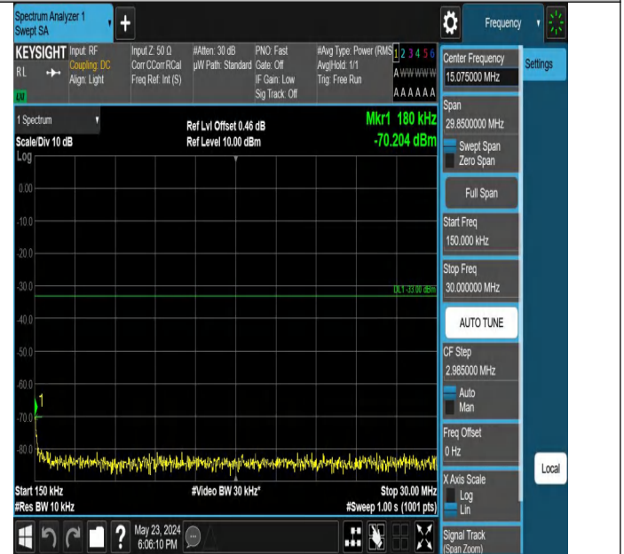
Band4_10MHz_QPSK_20000_1RB#0_0.15~30_0.15~30
