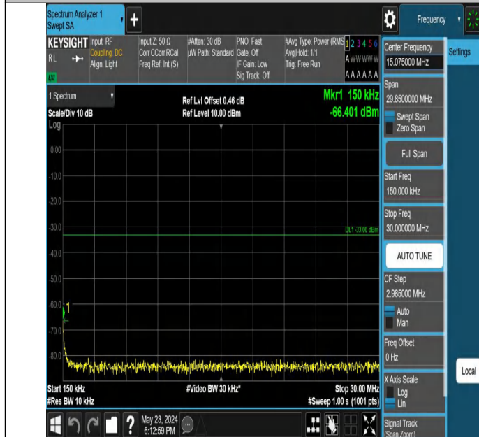
Band4_15MHz_QPSK_20025_1RB#74_0.15~30_0.15~30
