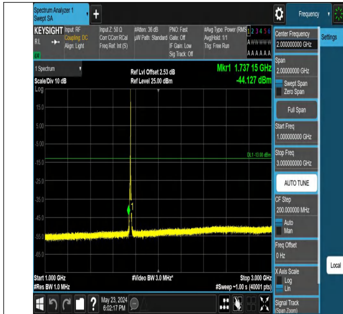
Band4_5MHz_QPSK_20375_1RB#24_1000~3000_1000~3000
