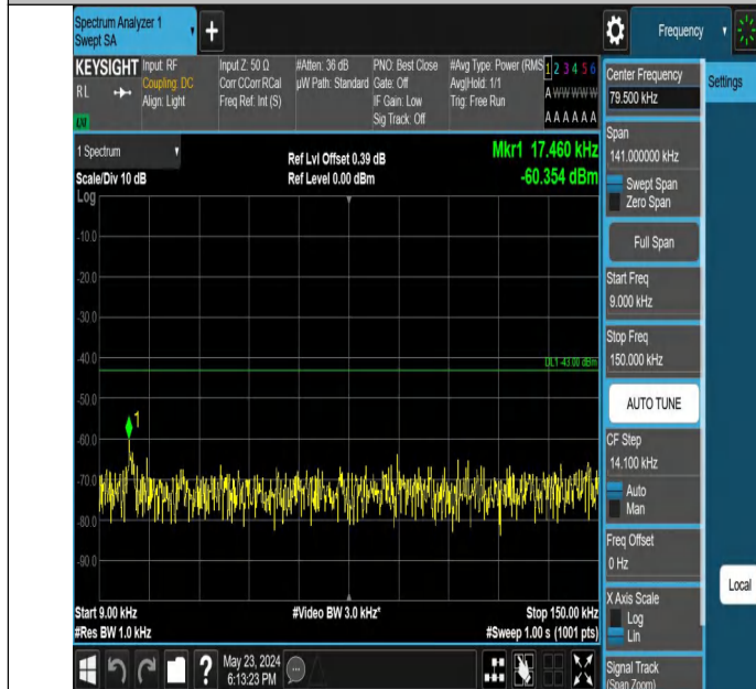
Band4_15MHz_QPSK_20175_1RB#0_0.009~0.15_0.009~0.15
