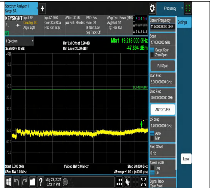
Band4_15MHz_QPSK_20025_1RB#74_3000~20000_3000~20000
