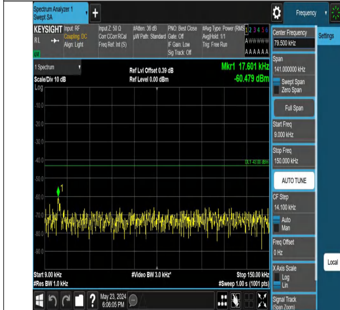
Band4_10MHz_QPSK_20000_1RB#0_0.009~0.15_0.009~0.15
