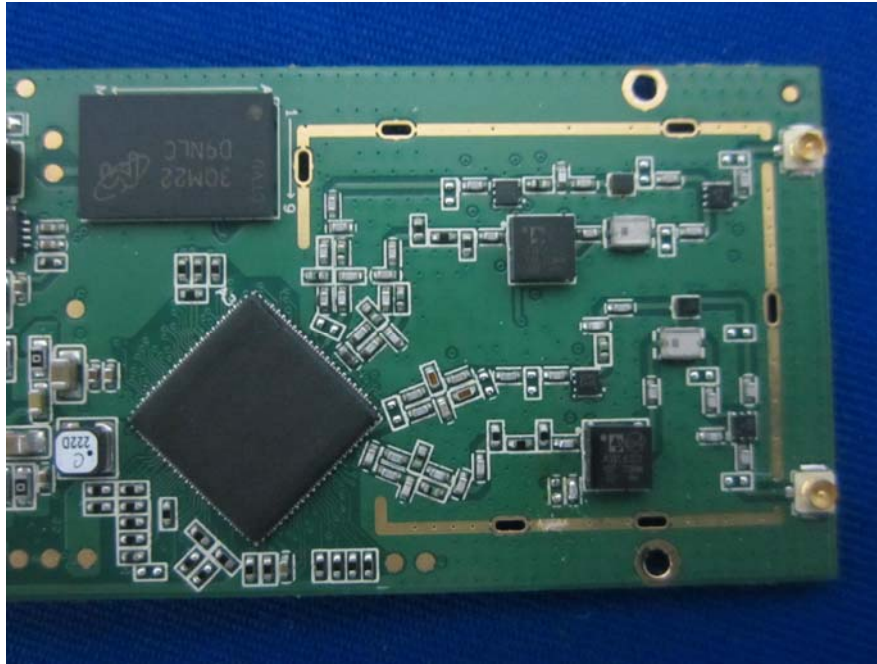
EUT- RF Part View
