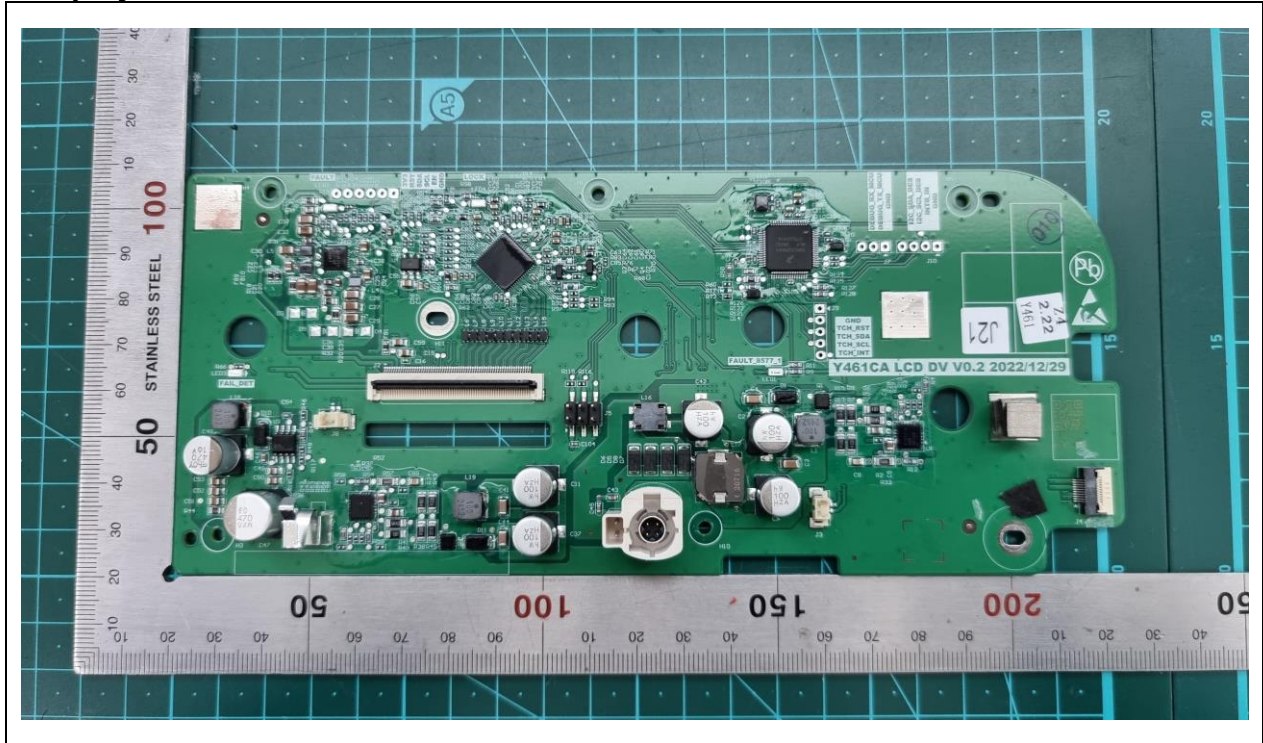
Display PCB Front
