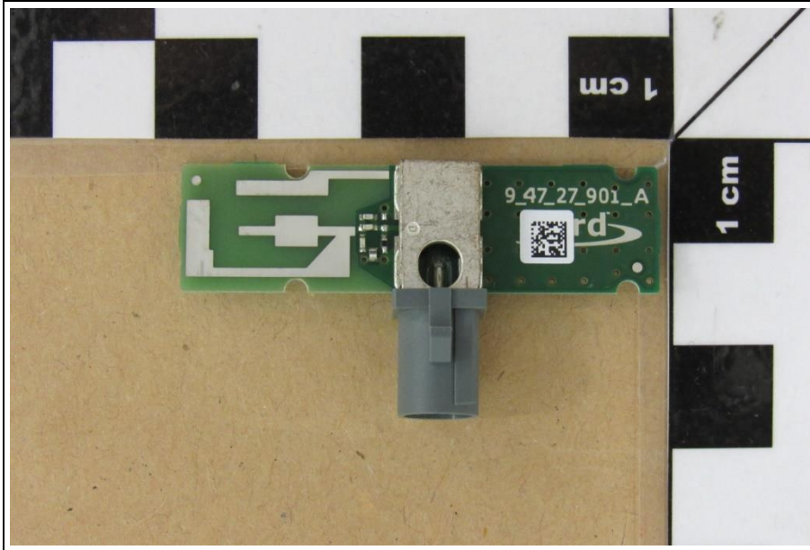
Wifi antenna 5B4.035.510 PCB top
