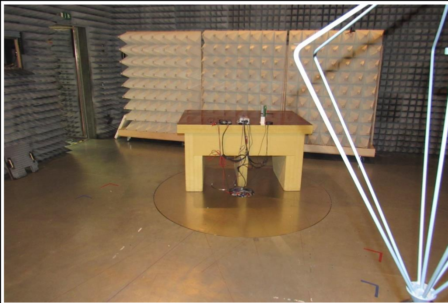
Testsetup view from measurement-antenna
