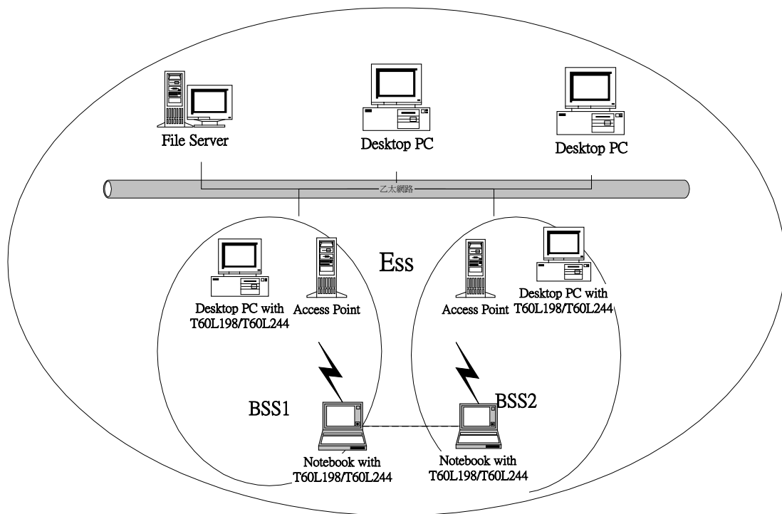
Fig.4 Roaming in an Extended Service Set (ESS)
