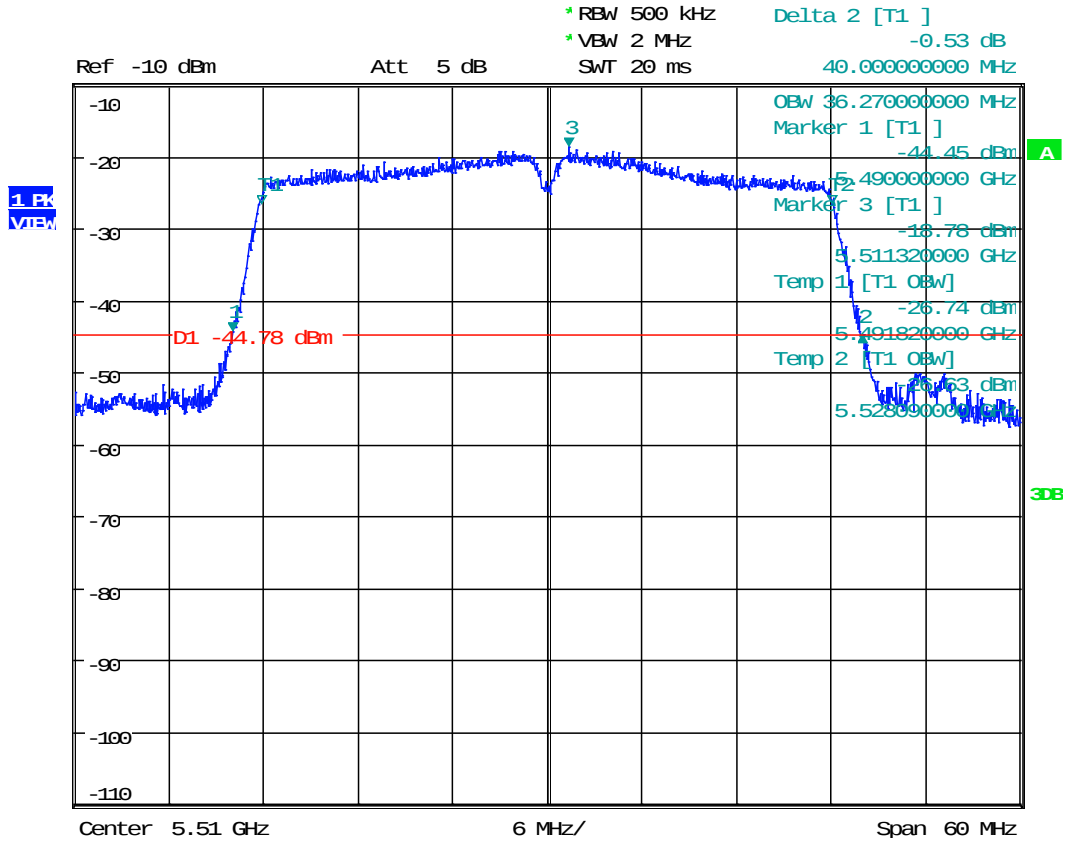
Plot 1.7 802.11n 40MHz, 5510MHz
