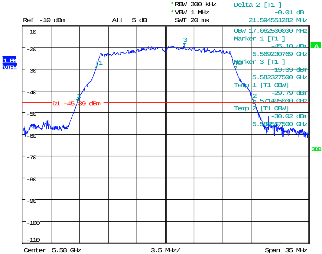
Plot 1.2 802.11a 5580MHz
