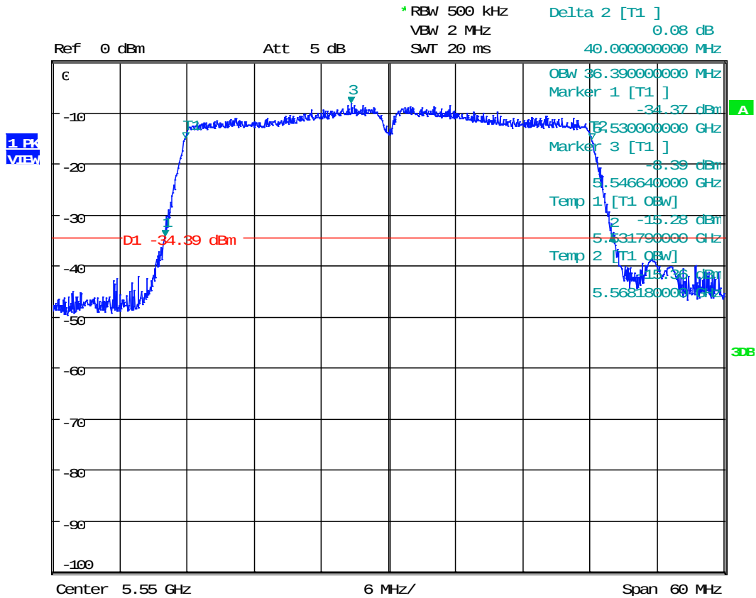
Plot 1. 8 802.11n 40MHz, 5550MHz
