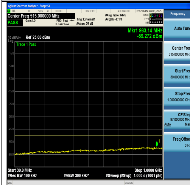
NTNV-n48-PC3-30-40-M-DFT-BPSK-Edge_1RB_Left-30- 1000-PASS
