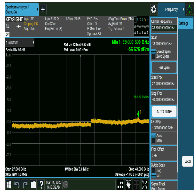
NTNV-n48-PC3-30-40-L-DFT-BPSK-Edge_1RB_Left- 27000-40000-PASS
