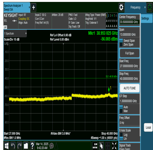
NTNV-n48-PC3-30-40-L-CP-QPSK-Edge_1RB_Left-27000-40000-PASS
