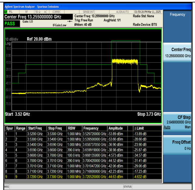
NTNV-n48-PC3-30-40-H-DFT-BPSK-Outer_Full-PASS
