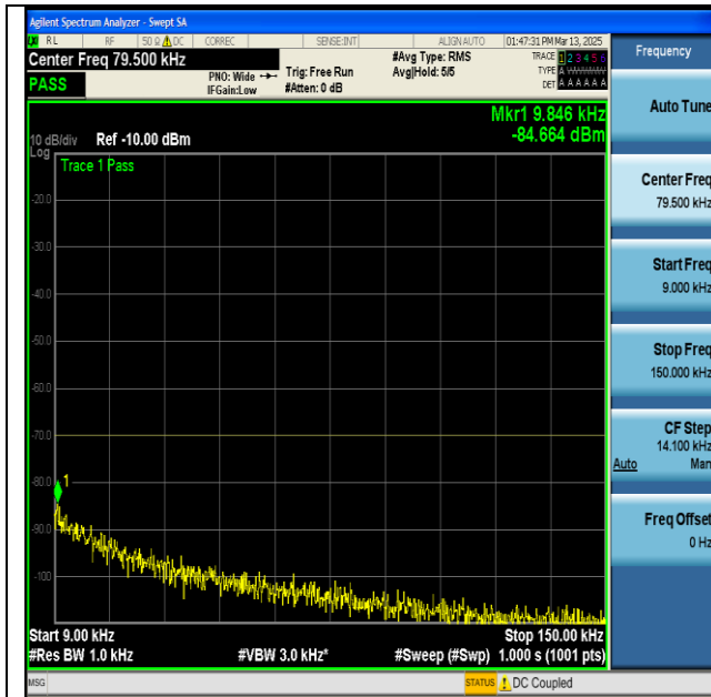
NTNV-n48-PC3-30-40-H-DFT-BPSK-Edge_1RB_Left- 0.009-0.15-PASS
