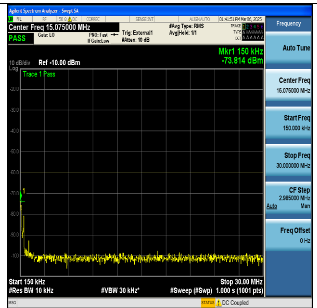
NTNV-n48-PC3-30-40-M-DFT-BPSK-Edge_1RB_Left- 0.15-30-PASS
