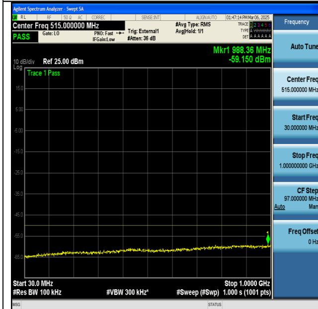
NTNV-n48-PC3-30-40-H-DFT-BPSK-Edge_1RB_Left-30- 1000-PASS
