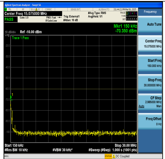
NTNV-n48-PC3-30-40-M-CP-QPSK-Edge_1RB_Left-0.15- 30-PASS
