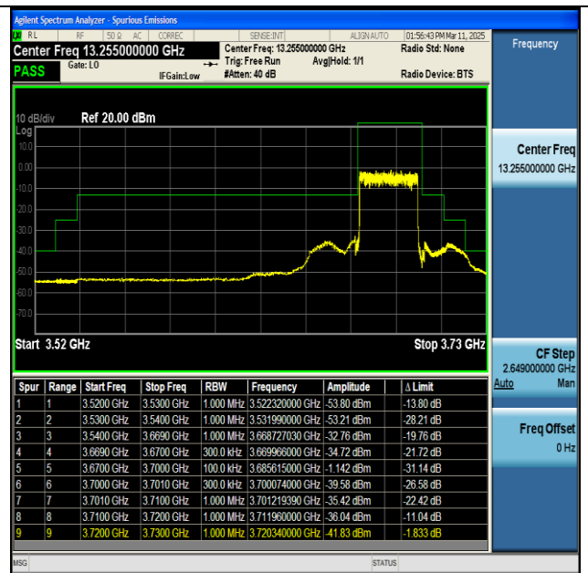
NTNV-n48-PC3-30-30-H-DFT-BPSK-Outer_Full-PASS
