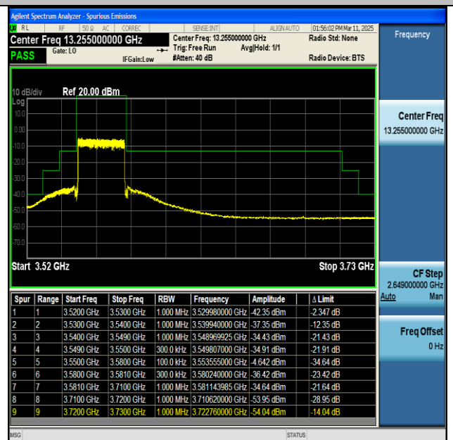
NTNV-n48-PC3-30-30-L-CP-QPSK-Outer_Full-PASS
