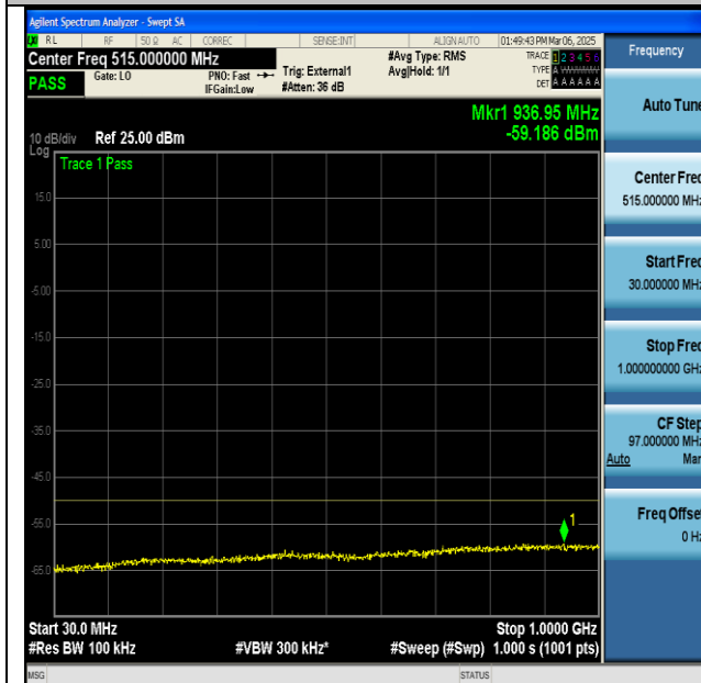
NTNV-n48-PC3-30-40-H-CP-QPSK-Edge_1RB_Left-30- 1000-PASS
