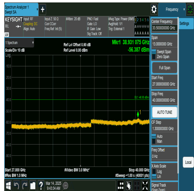
NTNV-n48-PC3-30-40-H-DFT-BPSK-Edge_1RB_Left- 27000-40000-PASS
