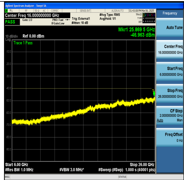
NTNV-n48-PC3-30-40-M-DFT-BPSK-Edge_1RB_Left- 6000-26000-PASS
