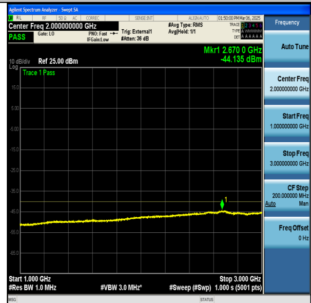
NTNV-n48-PC3-30-40-H-CP-QPSK-Edge_1RB_Left-1000- 3000-PASS
