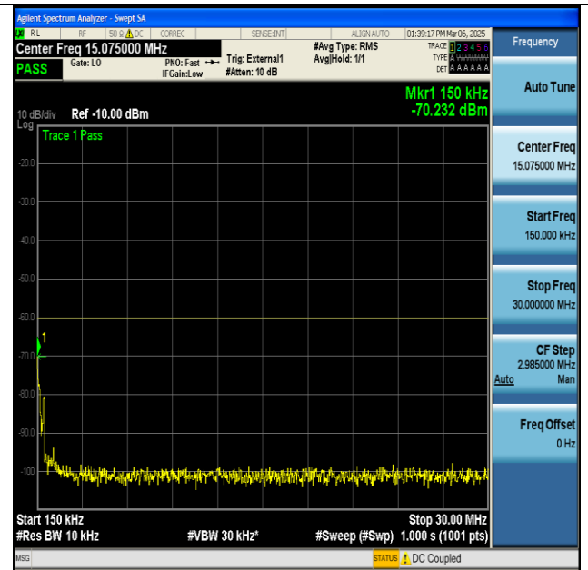
NTNV-n48-PC3-30-40-L-CP-QPSK-Edge_1RB_Left-0.15-30-PASS
