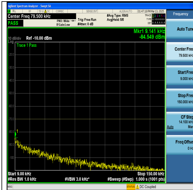
NTNV-n48-PC3-30-40-M-CP-QPSK-Edge_1RB_Left- 0.009-0.15-PASS
