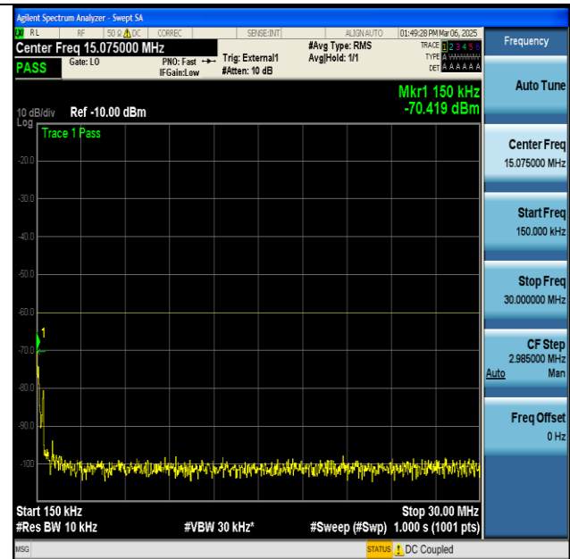
NTNV-n48-PC3-30-40-H-CP-QPSK-Edge_1RB_Left-0.15- 30-PASS
