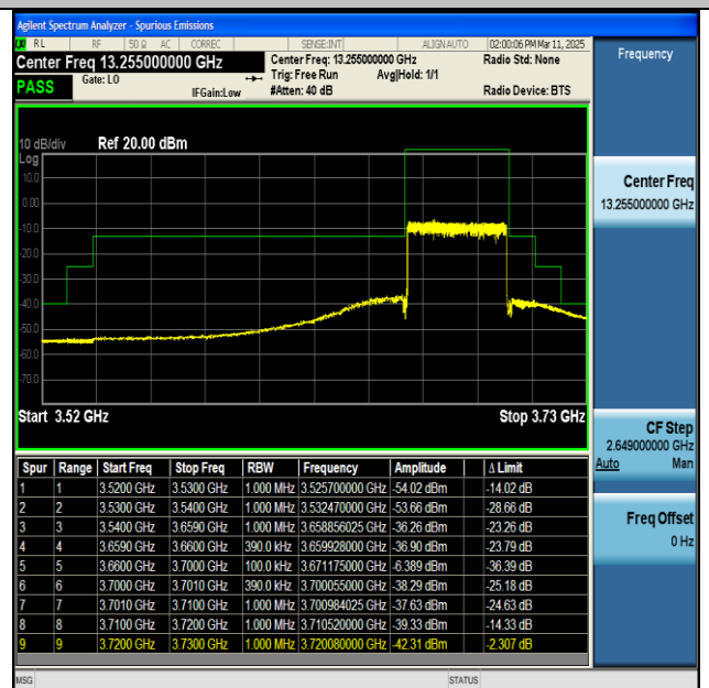
NTNV-n48-PC3-30-40-H-CP-QPSK-Outer_Full-PASS
