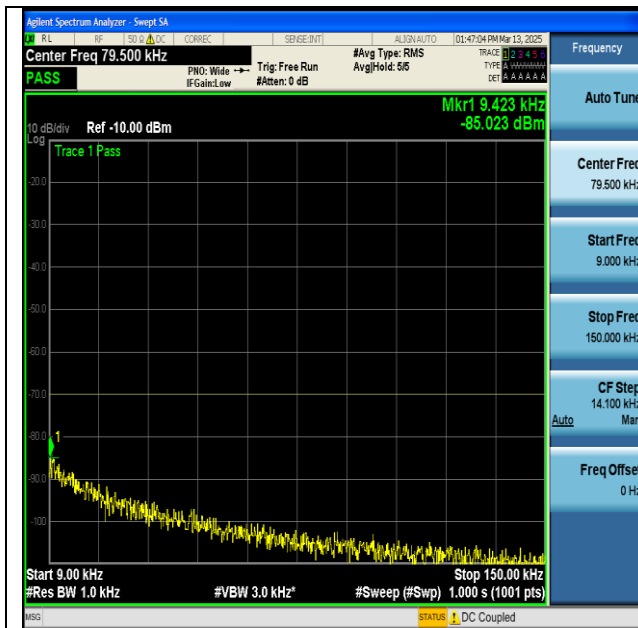
NTNV-n48-PC3-30-40-M-DFT-BPSK-Edge_1RB_Left- 0.009-0.15-PASS
