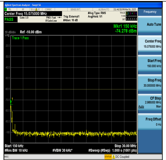
NTNV-n48-PC3-30-40-H-DFT-BPSK-Edge_1RB_Left-0.15- 30-PASS
