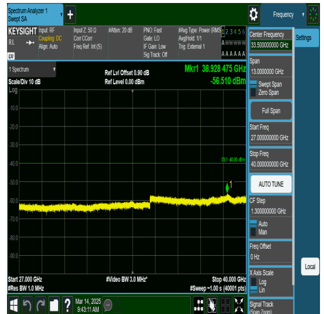
NTNV-n48-PC3-30-40-M-CP-QPSK-Edge_1RB_Left-27000-40000-PASS
