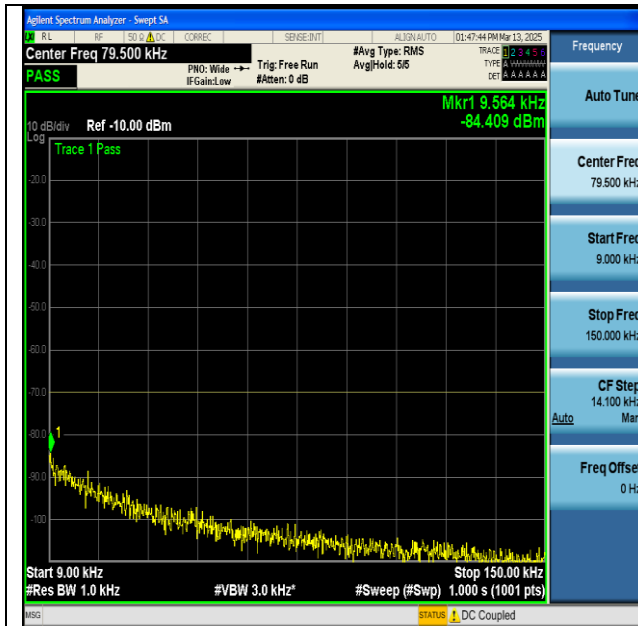
NTNV-n48-PC3-30-40-H-CP-QPSK-Edge_1RB_Left- 0.009-0.15-PASS
