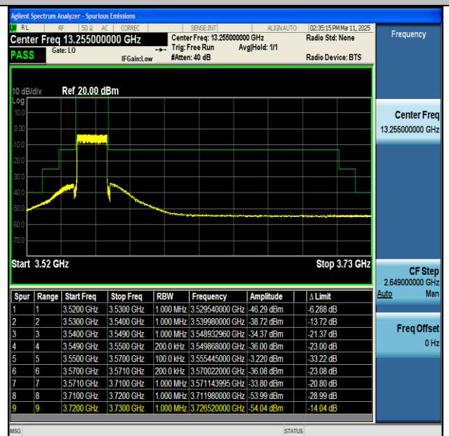
NTNV-n48-PC3-30-20-L-CP-QPSK-Outer_Full-PASS
