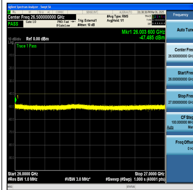
NTNV-n48-PC3-30-40-L-DFT-BPSK-Edge_1RB_Left- 26000-27000-PASS
