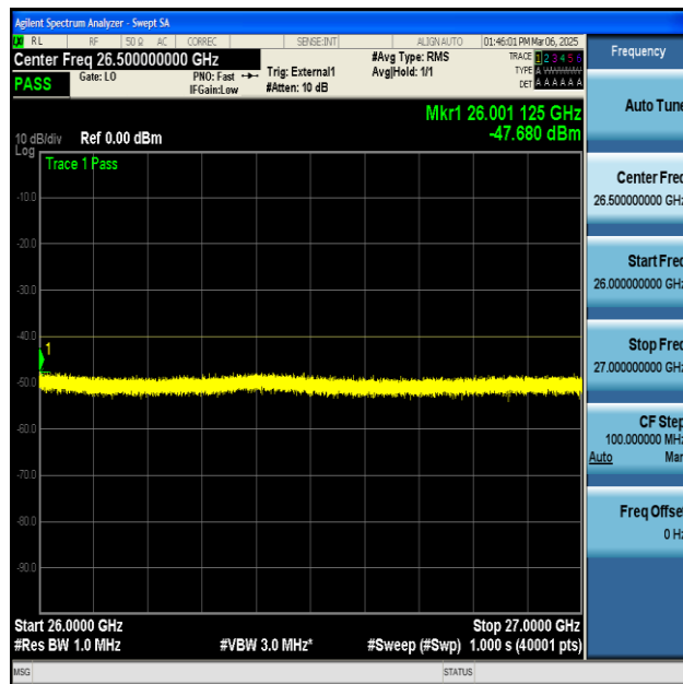
NTNV-n48-PC3-30-40-M-CP-QPSK-Edge_1RB_Left-26000-27000-PASS
