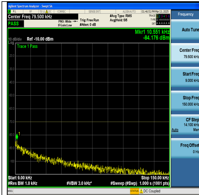
NTNV-n48-PC3-30-40-L-CP-QPSK-Edge_1RB_Left-0.009-0.15-PASS
