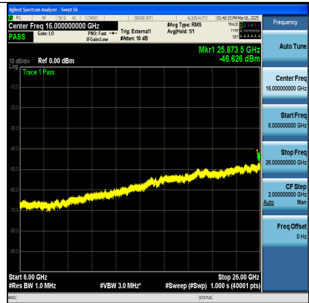
NTNV-n48-PC3-30-40-H-DFT-BPSK-Edge_1RB_Left- 6000-26000-PASS
