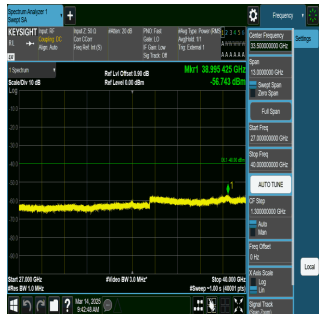
NTNV-n48-PC3-30-40-M-DFT-BPSK-Edge_1RB_Left- 27000-40000-PASS
