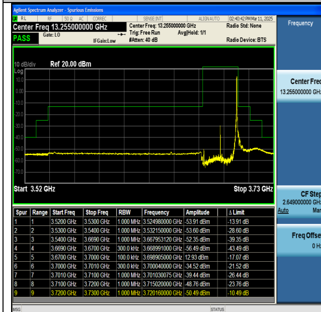
NTNV-n48-PC3-30-30-H-CP-QPSK-Edge_1RB_Right-PASS
