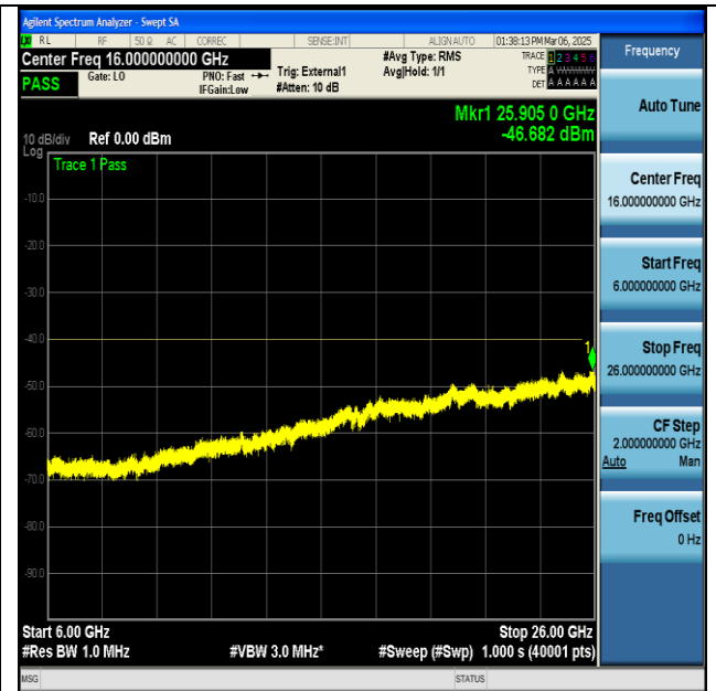
NTNV-n48-PC3-30-40-L-DFT-BPSK-Edge_1RB_Left- 6000-26000-PASS
