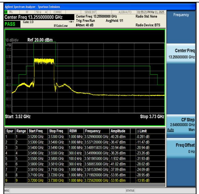
NTNV-n48-PC3-30-30-L-DFT-BPSK-Outer_Full-PASS
