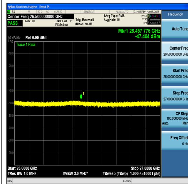
NTNV-n48-PC3-30-40-L-CP-QPSK-Edge_1RB_Left-26000-27000-PASS
