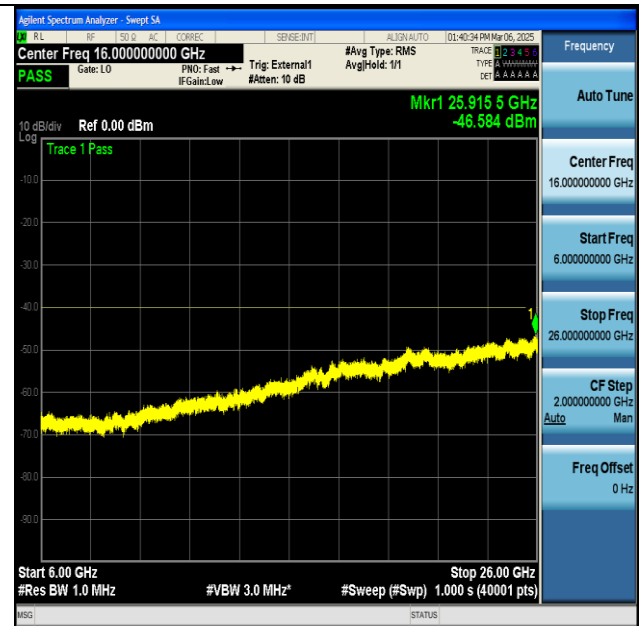
NTNV-n48-PC3-30-40-L-CP-QPSK-Edge_1RB_Left-6000-26000-PASS
