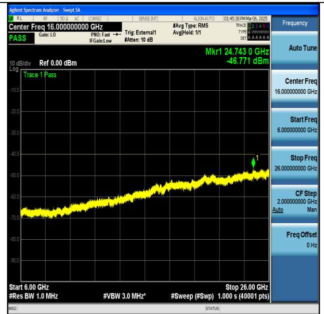
NTNV-n48-PC3-30-40-M-CP-QPSK-Edge_1RB_Left-6000-26000-PASS
