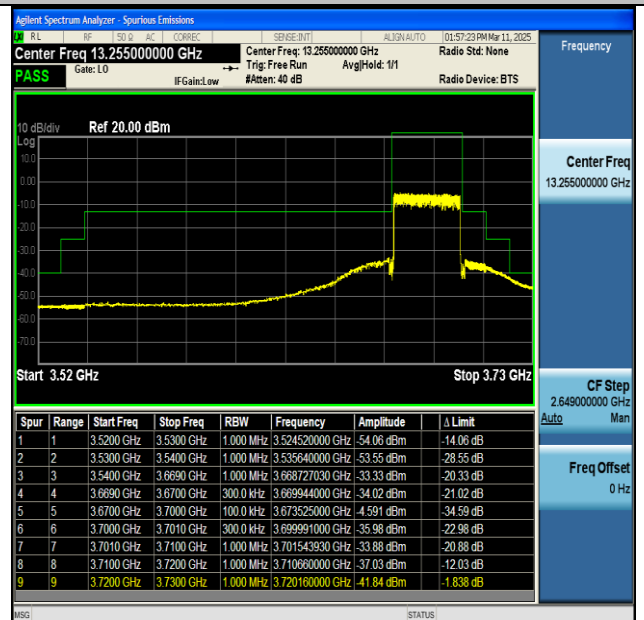
NTNV-n48-PC3-30-30-H-CP-QPSK-Outer_Full-PASS
