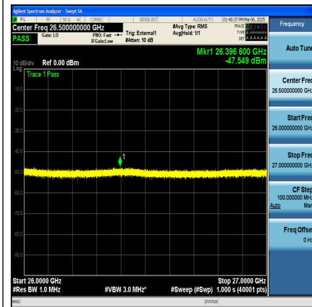
NTNV-n48-PC3-30-40-H-DFT-BPSK-Edge_1RB_Left- 26000-27000-PASS
