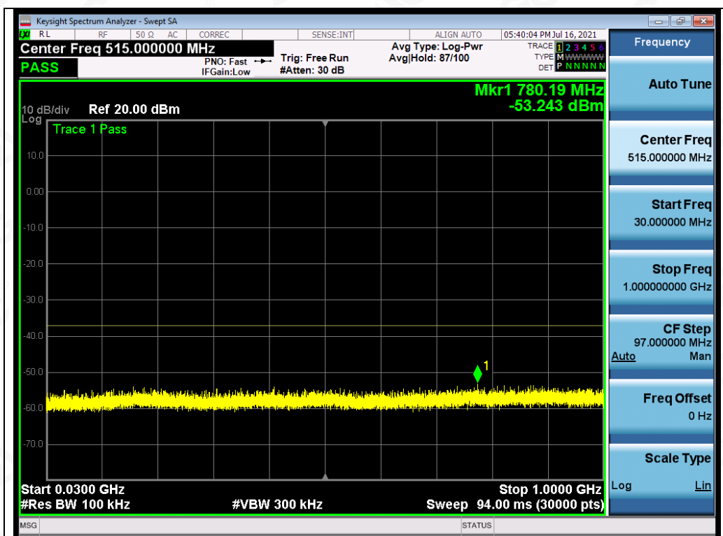
Test_Graph_802.11a_ANT1_5180_6Mbps_Frequency Band 1
