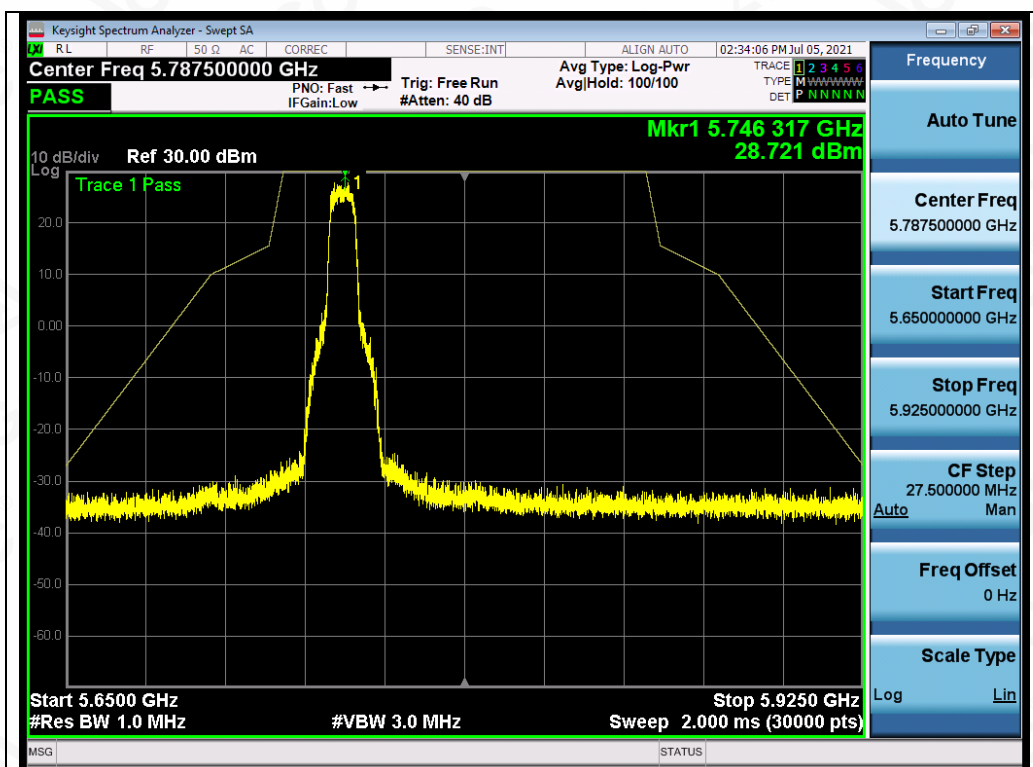
Test_Graph_OFDM_ANT1_5745_MCS0_Frequency Band3
