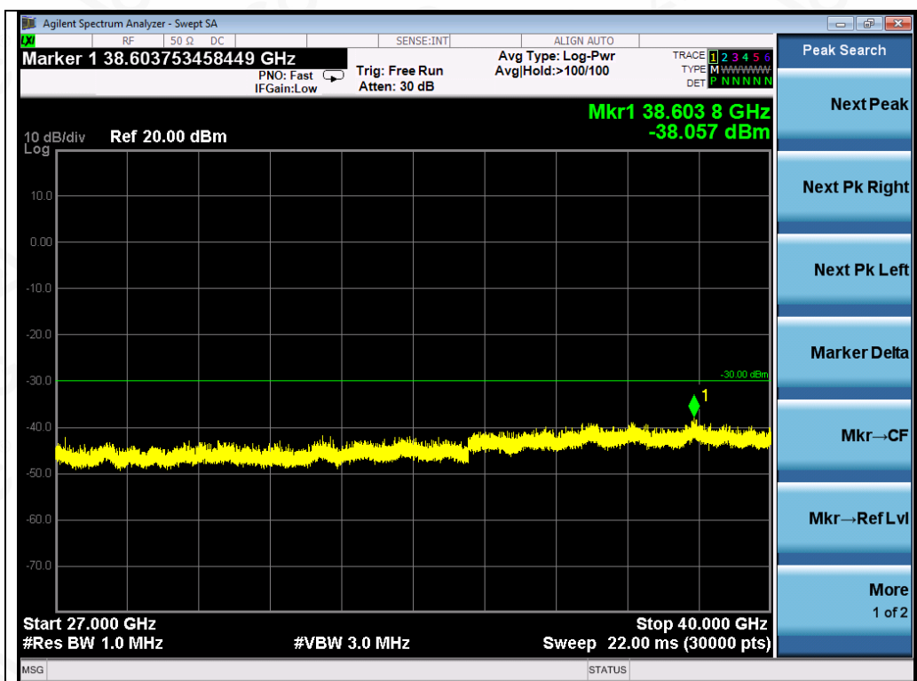
Test_Graph_OFDM_ANT1_5745_6Mbps_Frequency Band5
