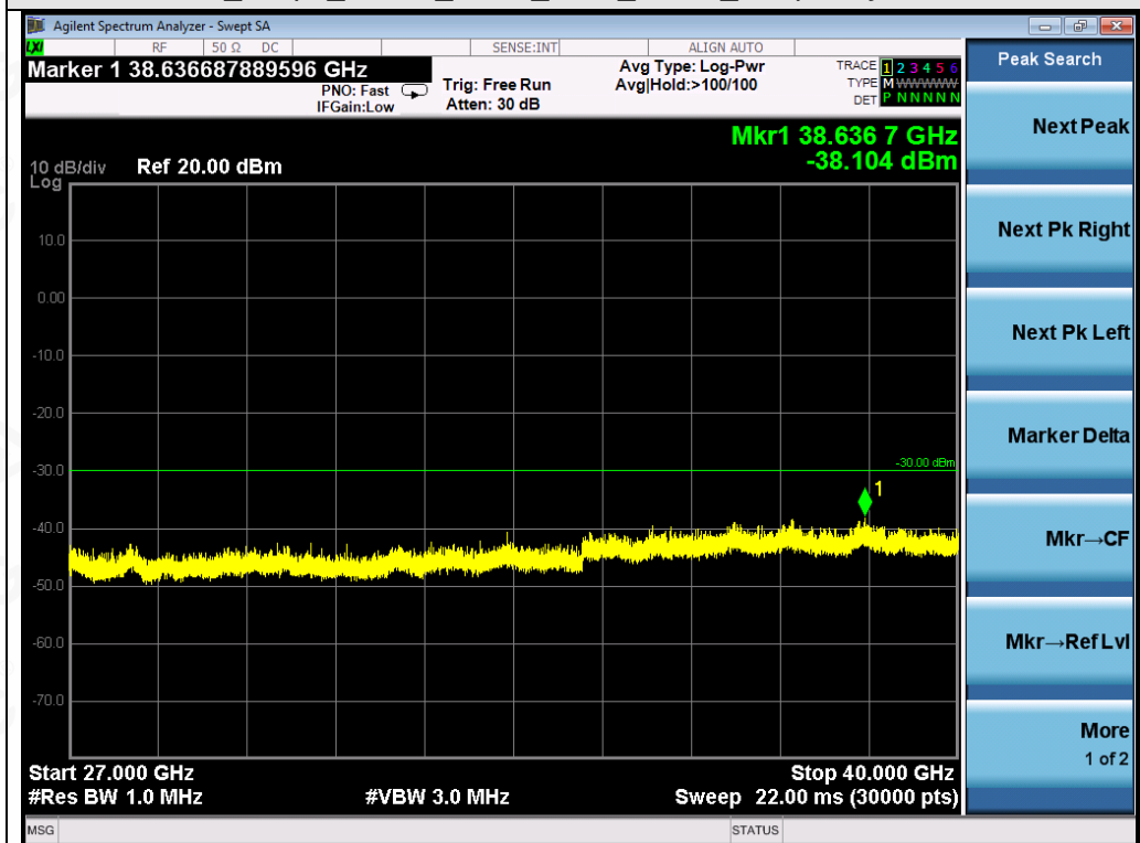
Test_Graph_OFDM_ANT1_5240_MCS0_Frequency Band 5
