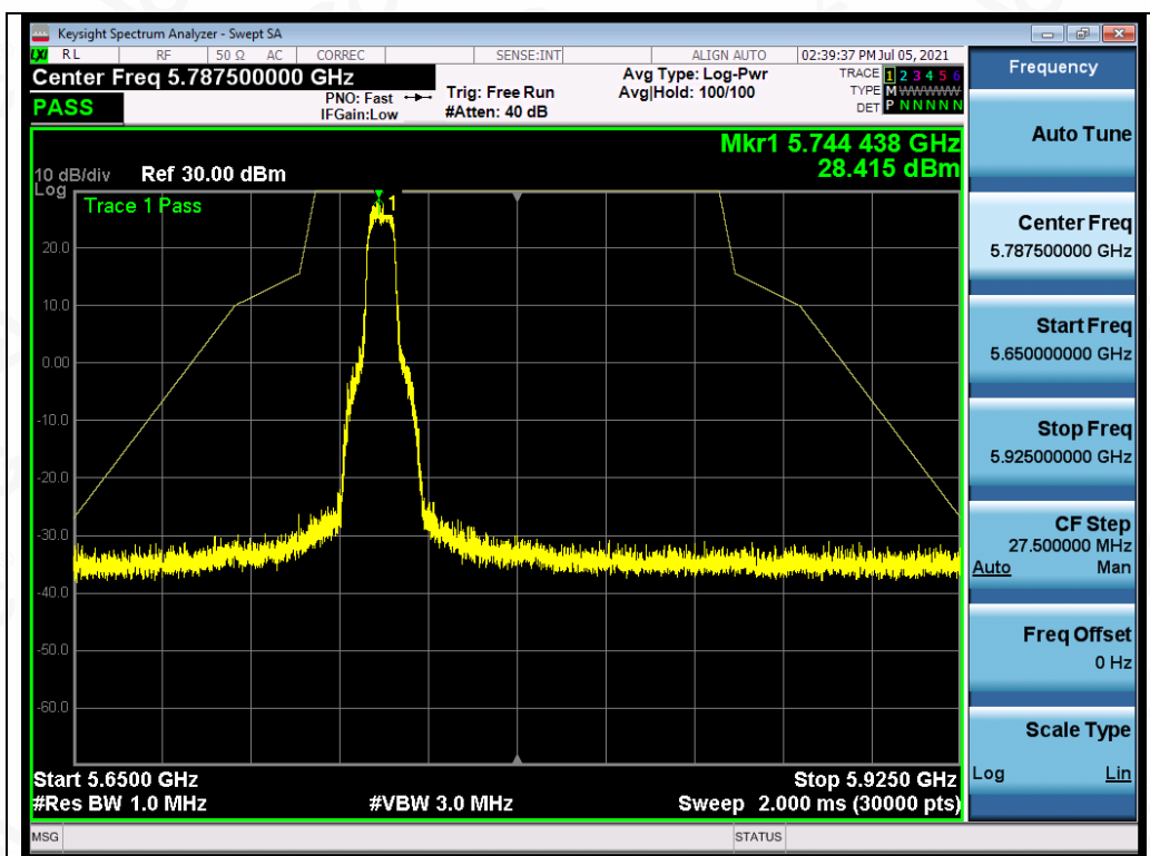
Test_Graph_OFDM_ANT1_5745_6Mbps_Frequency Band3
