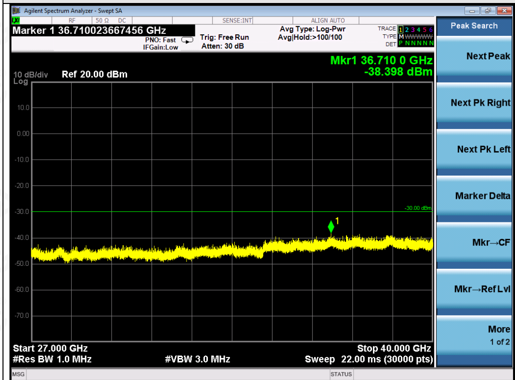
Test_Graph_OFDM_ANT1_5825_6Mbps_Frequency Band5
