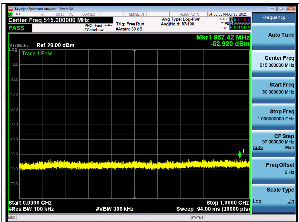
Test_Graph_OFDM_ANT1_5180_6Mbps_Frequency Band 1
