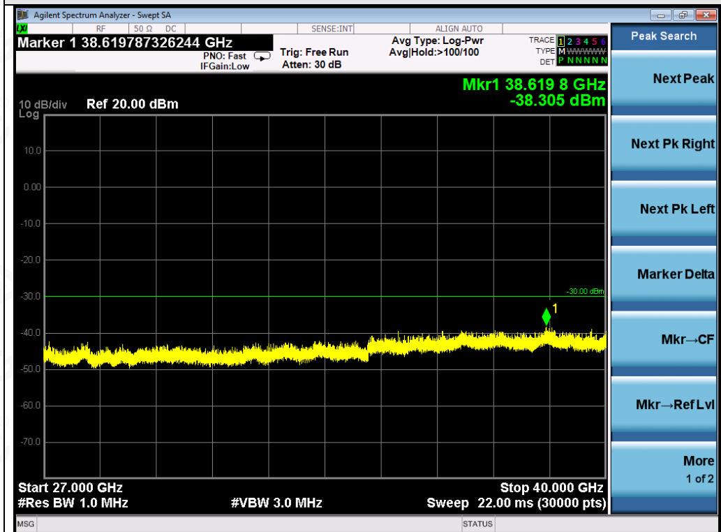
Test_Graph_OFDM_ANT1_5825_MCS0_Frequency Band5
