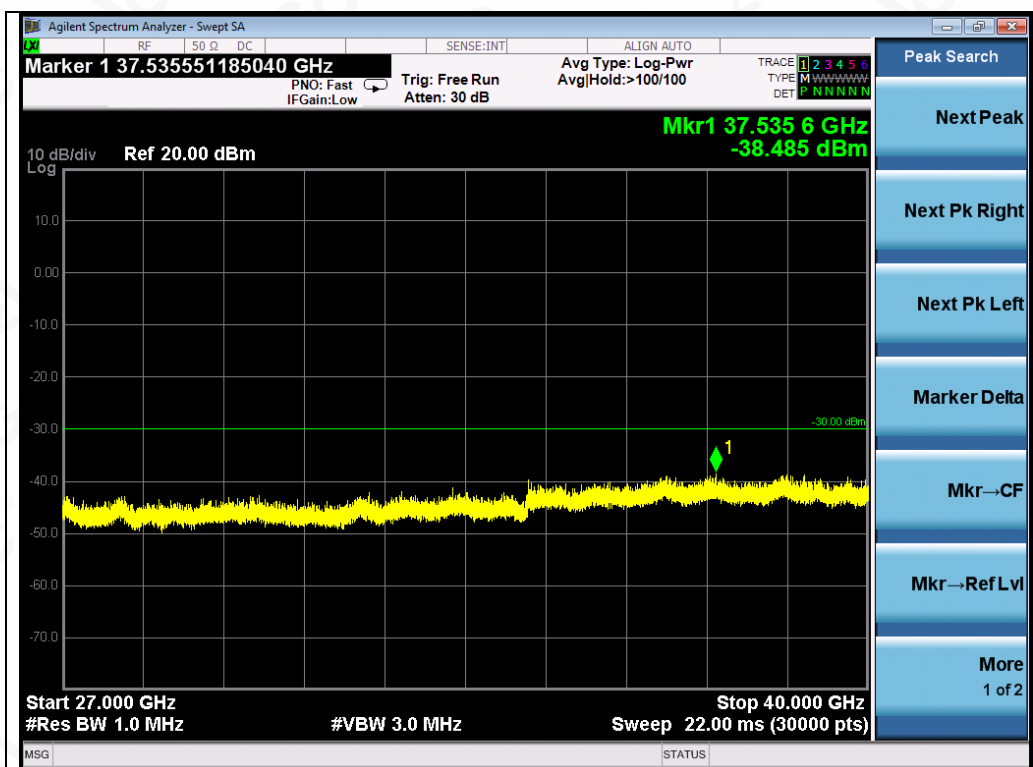
Test_Graph_OFDM_ANT1_5745_MCS0_Frequency Band5
