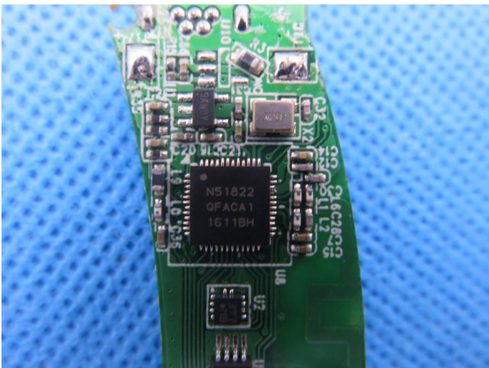
INTERNAL VIEW OF EUT-4(NRF51822)
