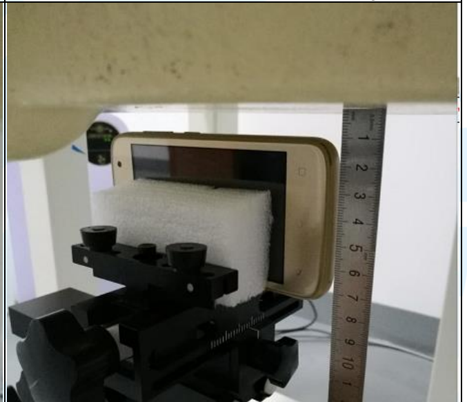
Right Side of EUT with 1.0 cm Gap
