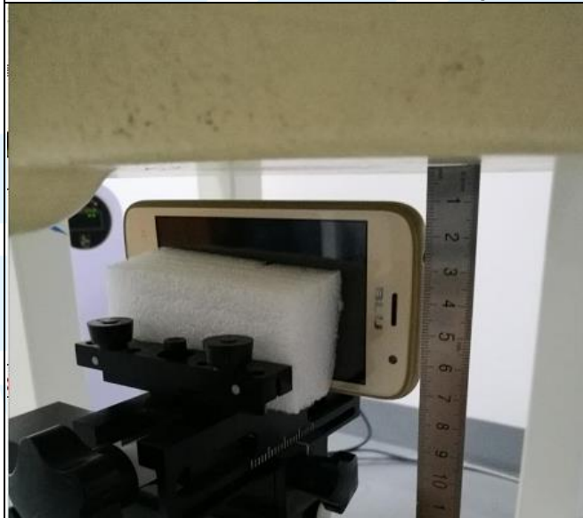
Left Side of EUT with 1.0 cm Gap
