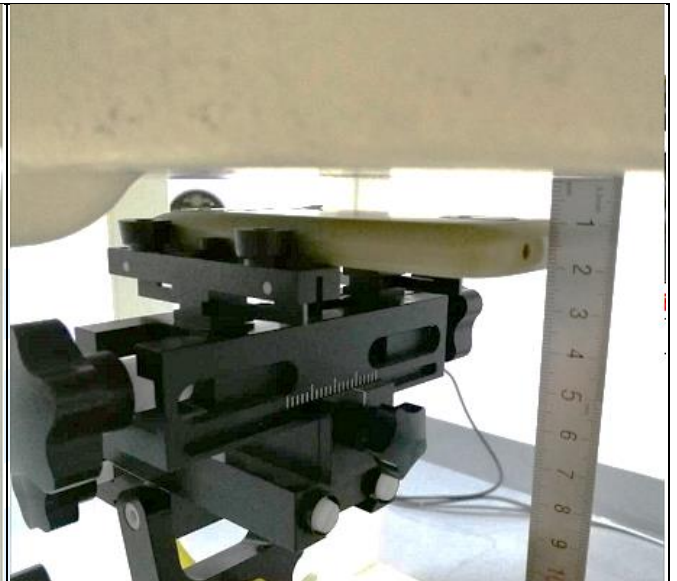
Rear Face of EUT with 1.0 cm Gap
