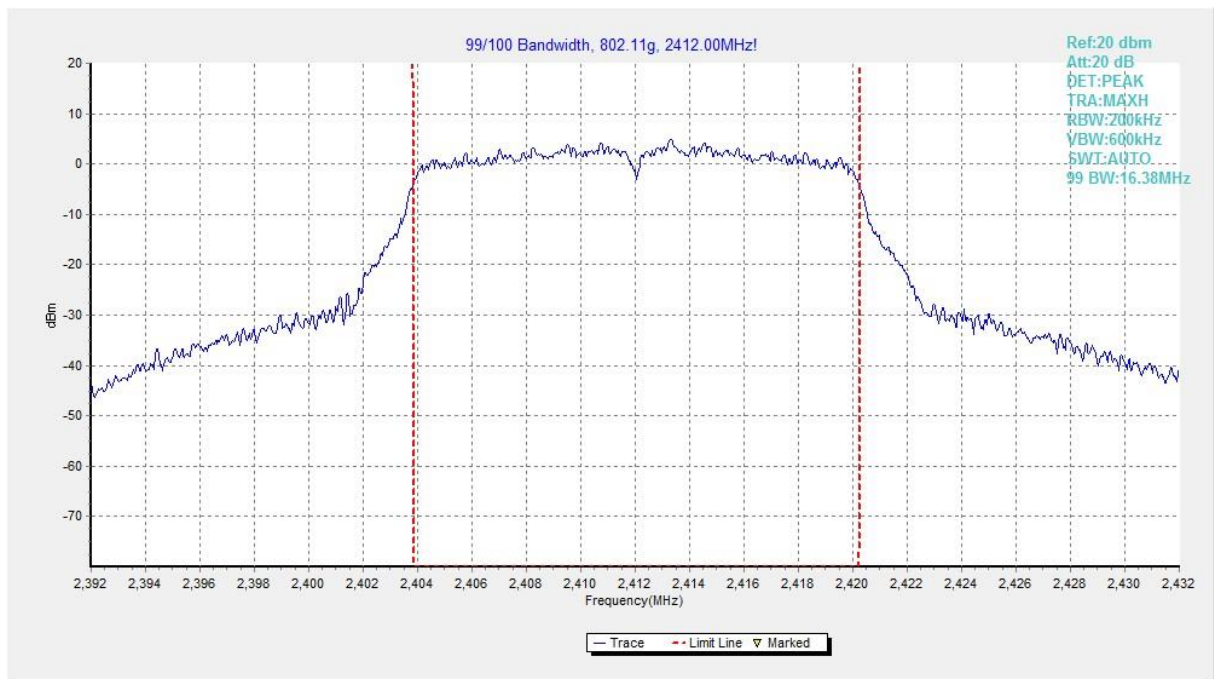
Fig.68 99% Occupied Bandwidth (802.11g, CH 1)
