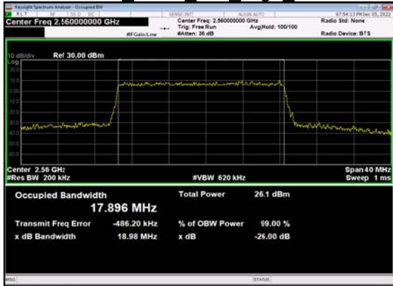
N7(20M)_DFT-s-OFDM_256 QAM Outer Full High CH
