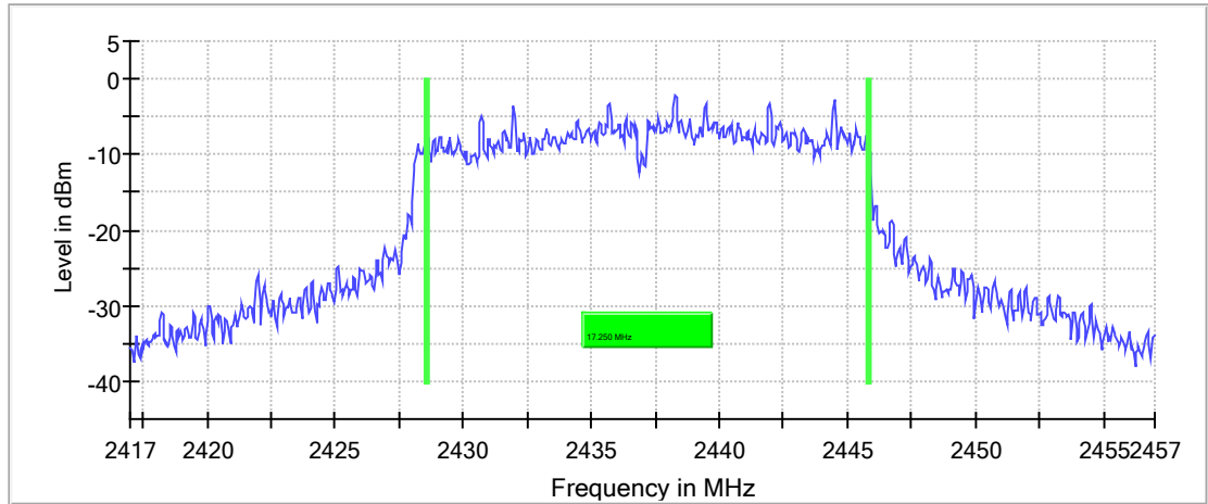
6 dB Bandwidth
