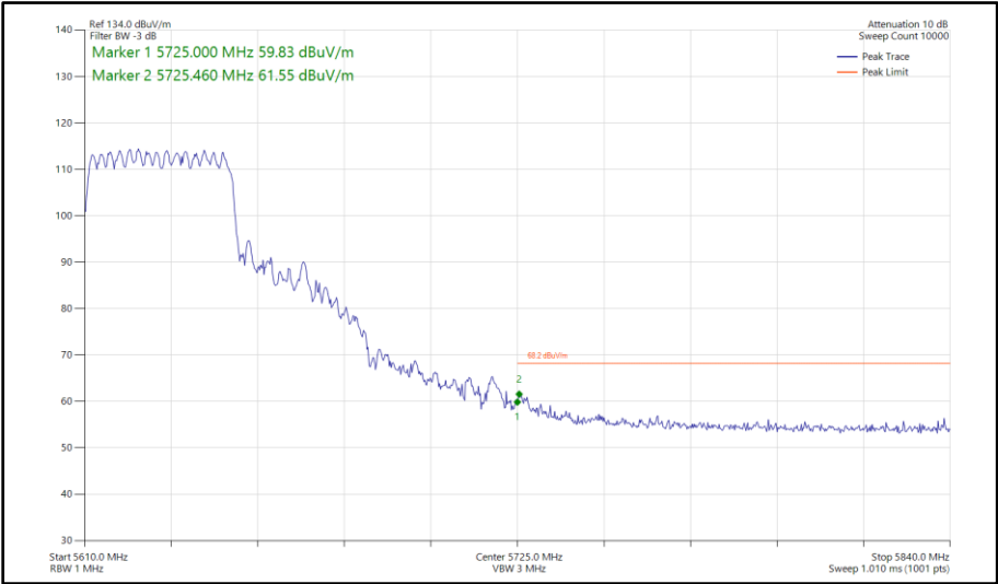
Figure 533 - 802.11ax HE40, SU, CDD, Core 0 - Core 1 - 5630 MHz Band Edge Frequency 5725 MHz
