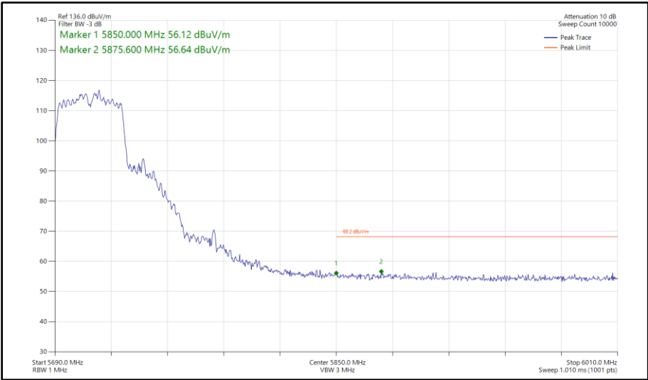
Figure 536 - 802.11n HT40, CDD, Core 0 - Core 1 - 5710 MHz Band Edge Frequency 5850 MHz
