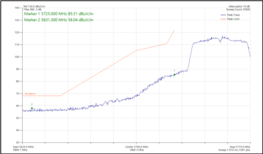
Figure 507 - 802.11n HT40, SISO, Core 1 - 5755 MHz Band Edge Frequency 5725 MHz
