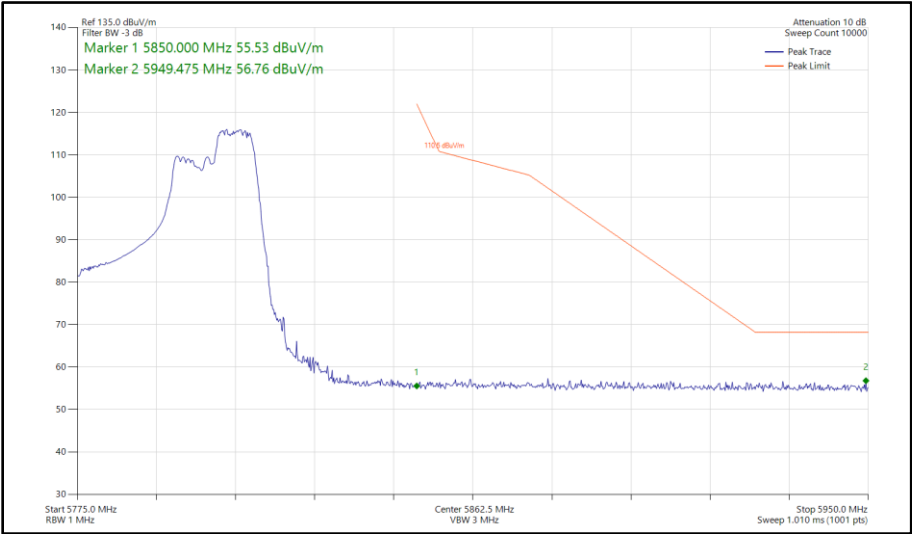
Figure 521 - 802.11ax HE40, RU 106-56, SISO, Core 1 - 5795 MHz Band Edge Frequency 5850 MHz
