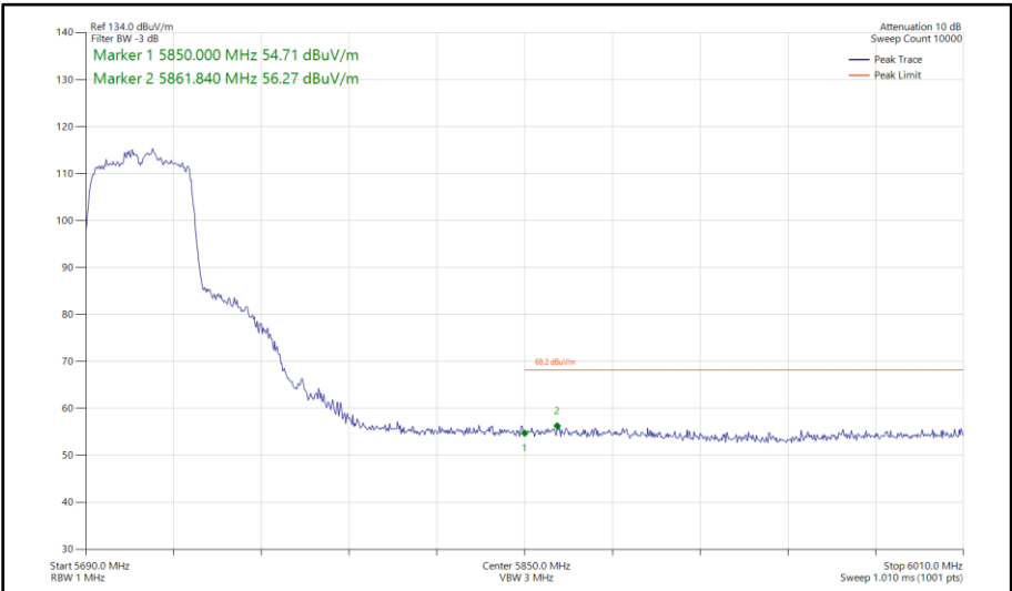
Figure 516 - 802.11n HT40, SISO, Core 1 - 5710 MHz Band Edge Frequency 5850 MHz
