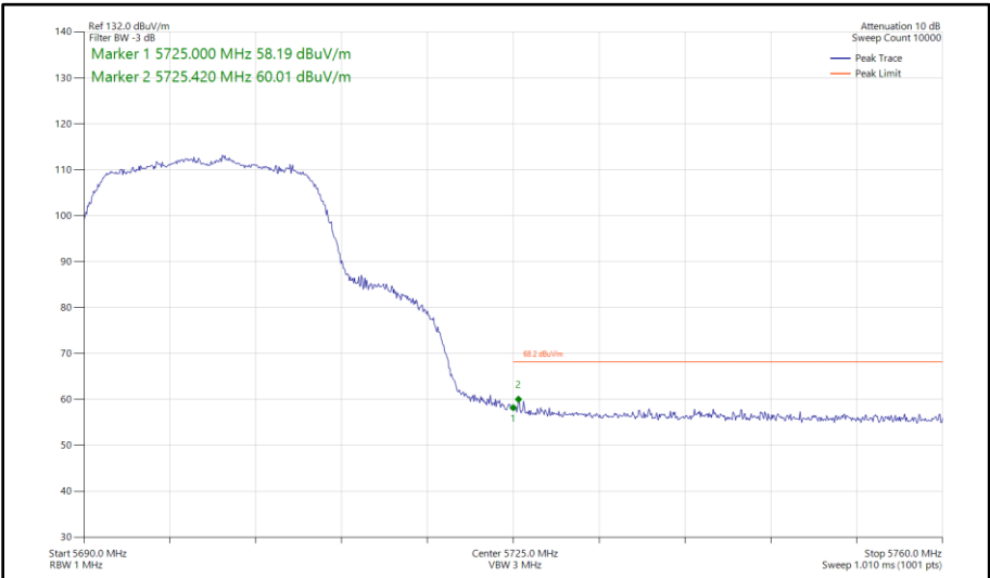
Figure 551 - 802.11n HT20, SDM, Core 0 - Core 1 - 5700 MHz Band Edge Frequency 5725 MHz
