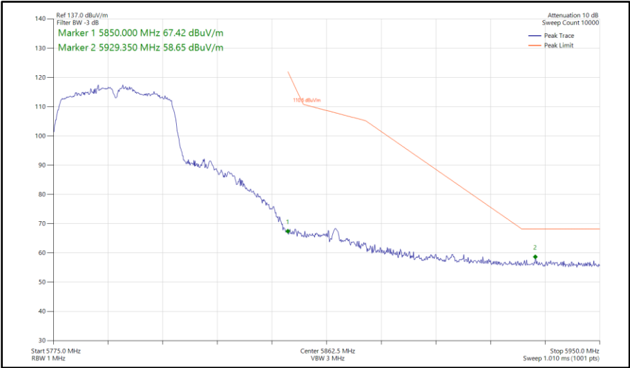
Figure 496 - 802.11n HT40, SISO, Core 0 - 5795 MHz Band Edge Frequency 5850 MHz
