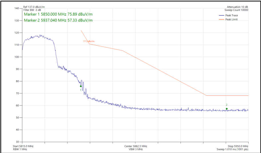
Figure 557 - 802.11n HT20, SDM, Core 0 - Core 1 - 5825 MHz Band Edge Frequency 5850 MHz
