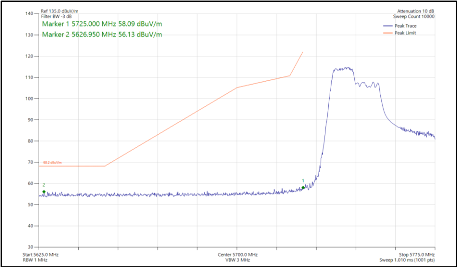
Figure 509 - 802.11ax HE40, RU 106-53, SISO, Core 1 - 5755 MHz Band Edge Frequency 5725 MHz
