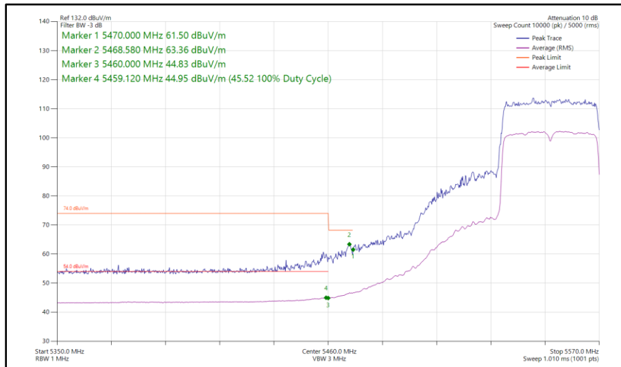
Figure 505 - 802.11ax HE40, SU, SISO, Core 1 - 5550 MHz Band Edge Frequency 5470 MHz
