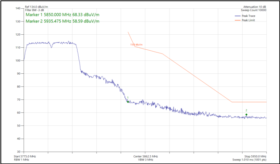
Figure 517 - 802.11n HT40, SISO, Core 1 - 5795 MHz Band Edge Frequency 5850 MHz
