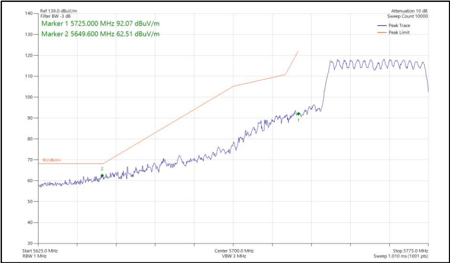
Figure 529 - 802.11ax HE40, SU, CDD, Core 0 - Core 1 - 5755 MHz Band Edge Frequency 5725 MHz
