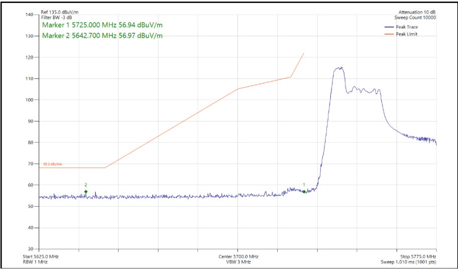
Figure 488 - 802.11ax HE40, RU 52-37, SISO, Core 0 - 5755 MHz Band Edge Frequency 5725 MHz
