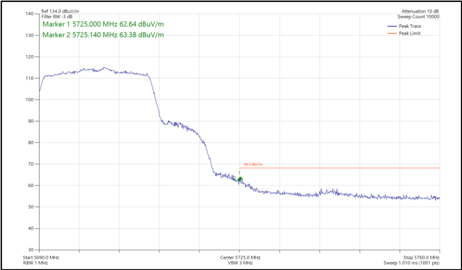
Figure 554 - 802.11ax HE20, SU, SDM, Core 0 - Core 1 - 5700 MHz Band Edge Frequency 5725 MHz
