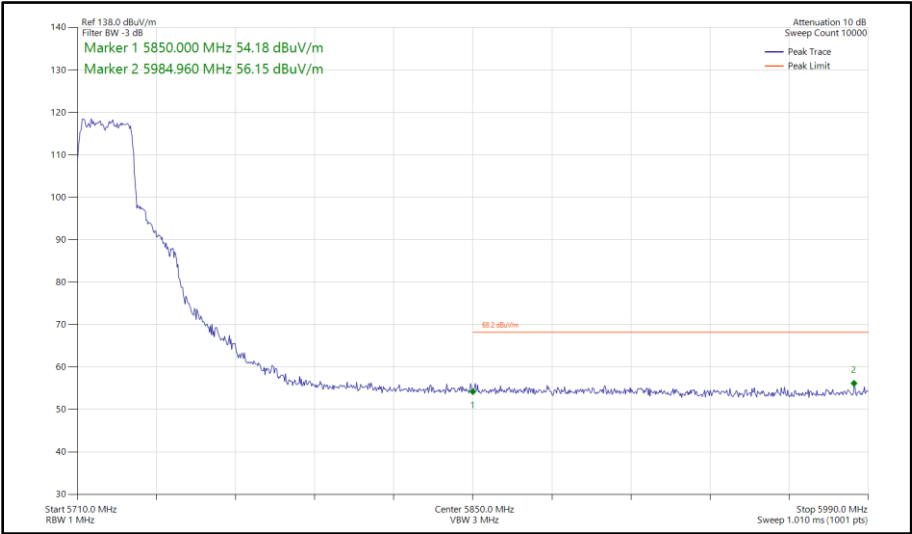
Figure 558 - 802.11ax HE20, SU, SDM, Core 0 - Core 1 - 5720 MHz Band Edge Frequency 5850 MHz
