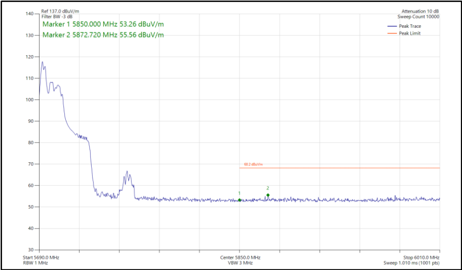
Figure 539 - 802.11ax HE40, RU 52-37, CDD, Core 0 - Core 1 - 5710 MHz Band Edge Frequency 5850 MHz
