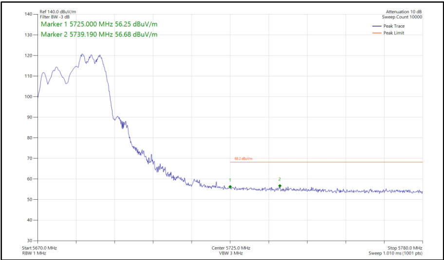
Figure 553 - 802.11ax HE20, RU 106-54, SDM, Core 0 - Core 1 - 5680 MHz Band Edge Frequency 5725 MHz
