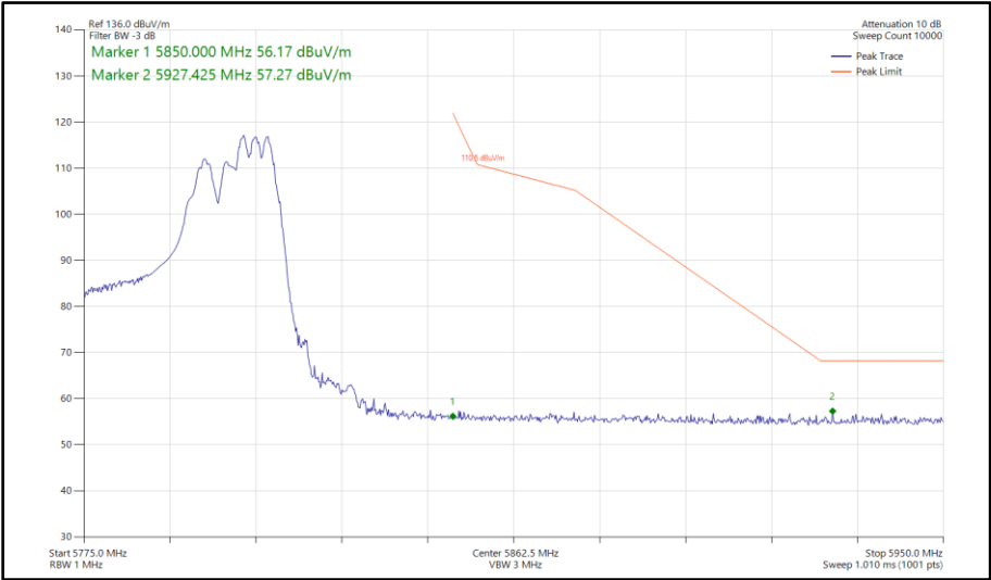
Figure 541 - 802.11ax HE40, RU 106-56, CDD, Core 0 - Core 1 - 5795 MHz Band Edge Frequency 5850 MHz
