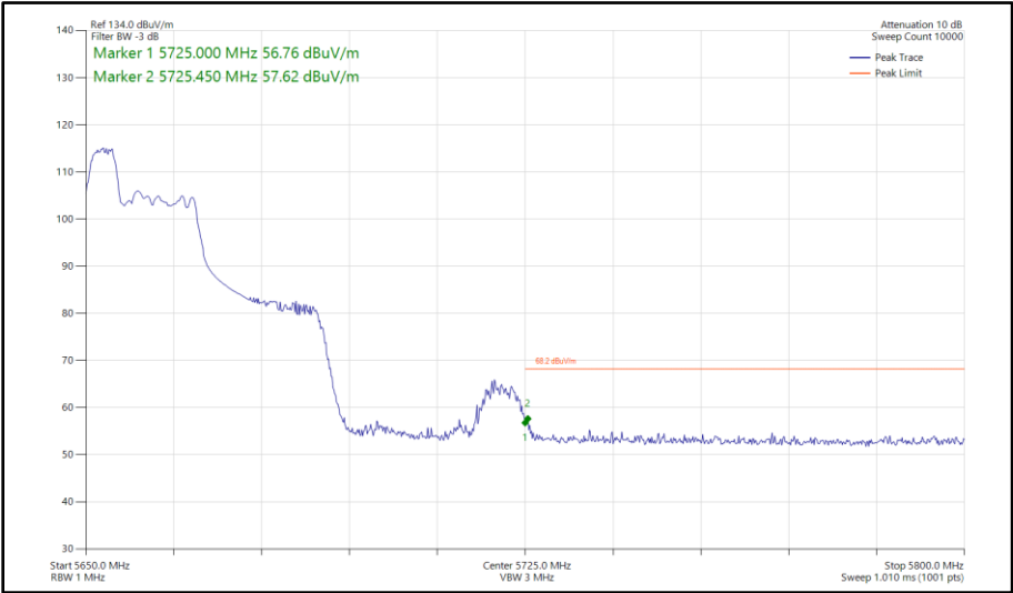
Figure 494 - 802.11ax HE40, RU 52-37, SISO, Core 0 - 5670 MHz Band Edge Frequency 5725 MHz
