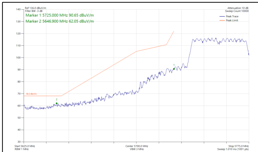
Figure 528 - 802.11n HT40, CDD, Core 0 - Core 1 - 5755 MHz Band Edge Frequency 5725 MHz
