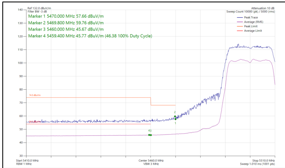
Figure 542 - 802.11n HT20, SDM, Core 0-1 - 5500 MHz Band Edge Frequency 5470 MHz
