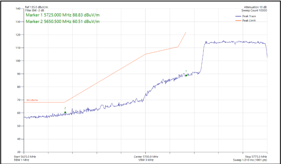
Figure 487 - 802.11ax HE40, SU, SISO, Core 0 - 5755 MHz Band Edge Frequency 5725 MHz
