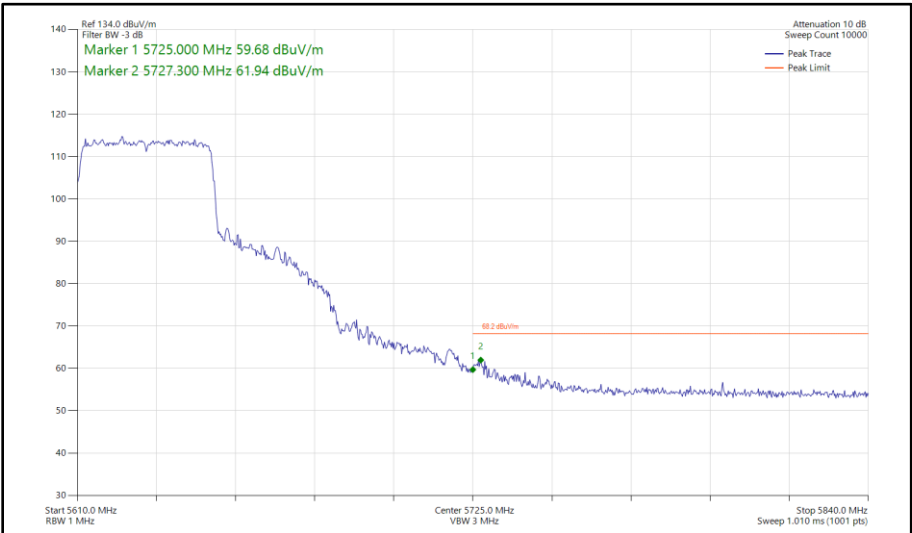
Figure 491 - 802.11ax HE40, SU, SISO, Core 0 - 5630 MHz Band Edge Frequency 5725 MHz
