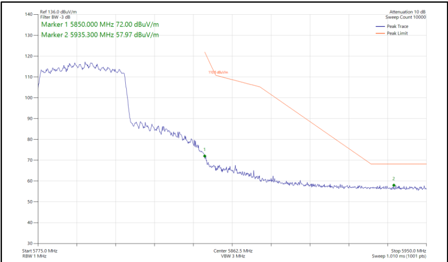
Figure 540 - 802.11ax HE40, SU, CDD, Core 0 - Core 1 - 5795 MHz Band Edge Frequency 5850 MHz
