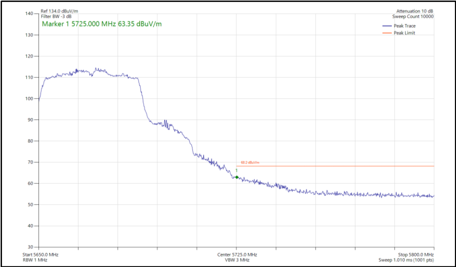
Figure 490 - 802.11n HT40, SISO, Core 0 - 5670 MHz Band Edge Frequency 5725 MHz
