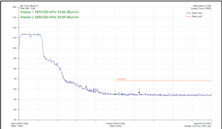
Figure 495 - 802.11n HT40, SISO, Core 0 - 5710 MHz Band Edge Frequency 5850 MHz
