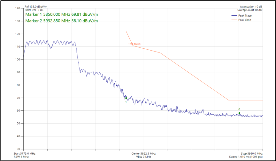
Figure 537 - 802.11n HT40, CDD, Core 0 - Core 1 - 5795 MHz Band Edge Frequency 5850 MHz
