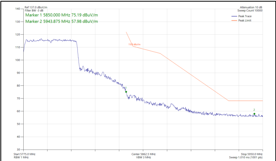
Figure 499 - 802.11ax HE40, SU, SISO, Core 0 - 5795 MHz Band Edge Frequency 5850 MHz
