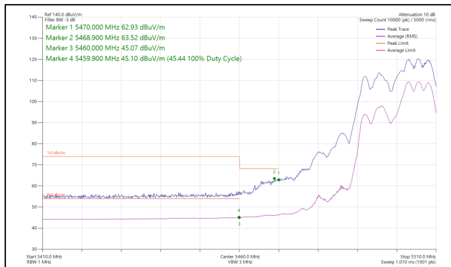
Figure 544 - 802.11ax HE20, RU 106-54, SDM, Core 0 - Core 1 - 5500 MHz Band Edge Frequency 5470 MHz
