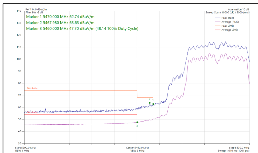
Figure 522 - 802.11n HT40, CDD, Core 0 - Core 1 - 5510 MHz Band Edge Frequency 5470 MHz
