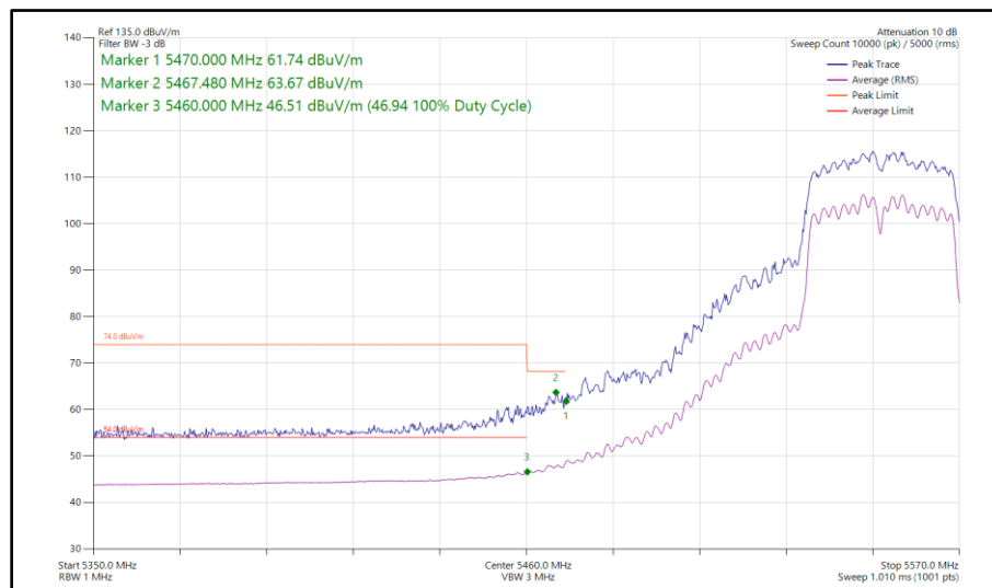
Figure 523 - 802.11n HT40, CDD, Core 0 - Core 1 - 5550 MHz Band Edge Frequency 5470 MHz
