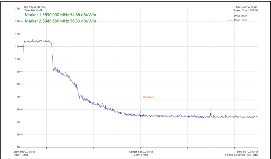
Figure 497 - 802.11ax HE40, SU, SISO, Core 0 - 5710 MHz Band Edge Frequency 5850 MHz
