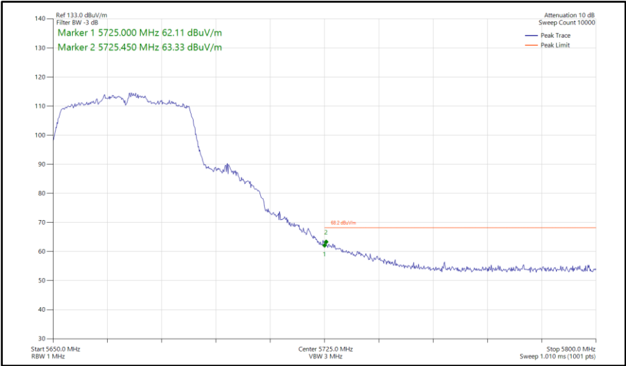
Figure 511 - 802.11n HT40, SISO, Core 1 - 5670 MHz Band Edge Frequency 5725 MHz
