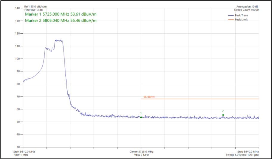
Figure 492 - 802.11ax HE40, RU 106-56, SISO, Core 0 - 5630 MHz Band Edge Frequency 5725 MHz
