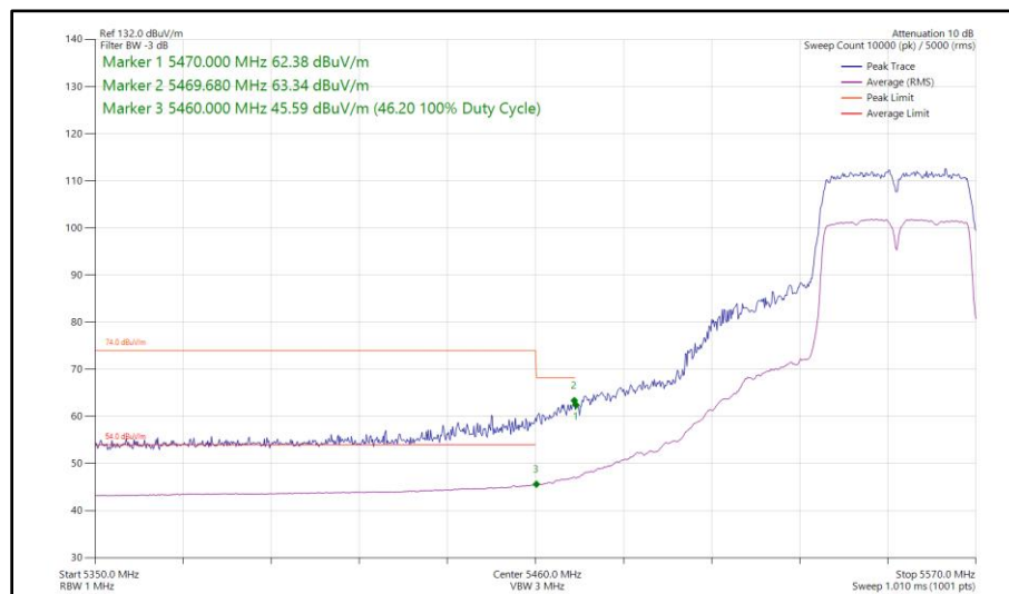
Figure 502 - 802.11n HT40, SISO, Core 1 - 5550 MHz Band Edge Frequency 5470 MHz
