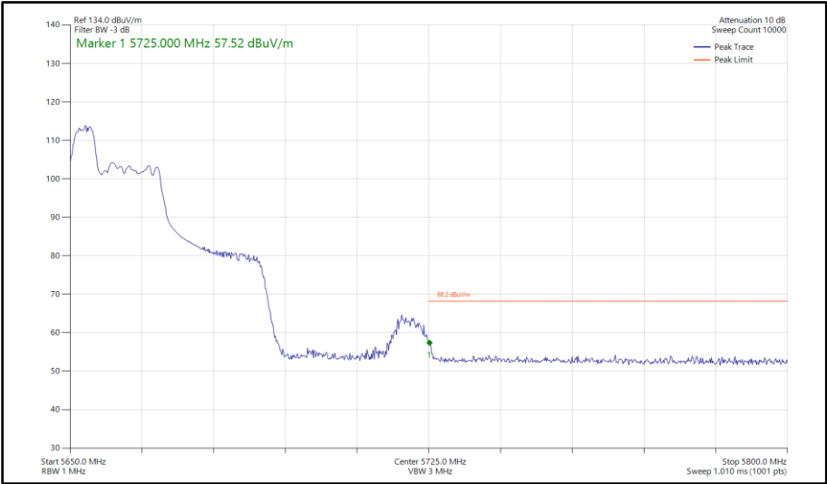
Figure 515 - 802.11ax HE40, RU 52-37, SISO, Core 1 - 5670 MHz Band Edge Frequency 5725 MHz
