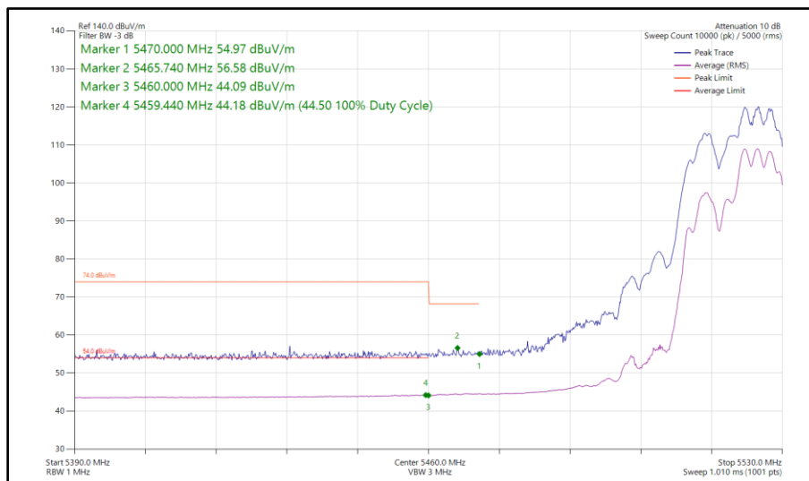
Figure 546 - 802.11ax HE20, RU 106-54, SDM, Core 0 - Core 1 - 5520 MHz Band Edge Frequency 5470 MHz
