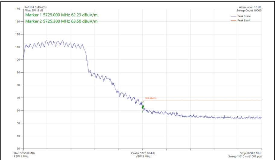
Figure 534 - 802.11ax HE40, SU, CDD, Core 0 - Core 1 - 5670 MHz Band Edge Frequency 5725 MHz
