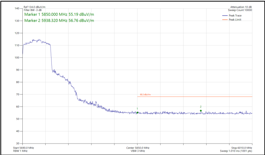
Figure 518 - 802.11ax HE40, SU, SISO, Core 1 - 5710 MHz Band Edge Frequency 5850 MHz
