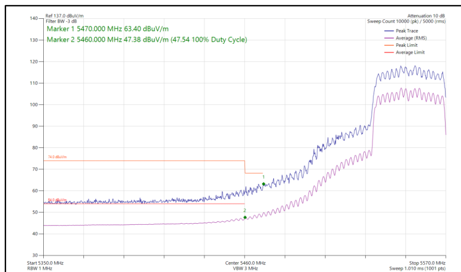
Figure 526 - 802.11ax HE40, SU, CDD, Core 0 - Core 1 - 5550 MHz Band Edge Frequency 5470 MHz
