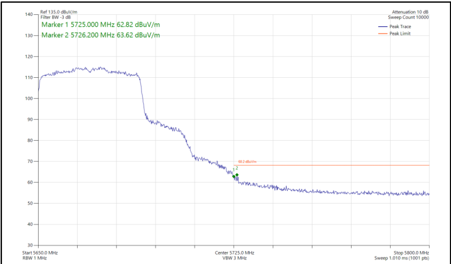
Figure 493 - 802.11ax HE40, SU, SISO, Core 0 - 5670 MHz Band Edge Frequency 5725 MHz
