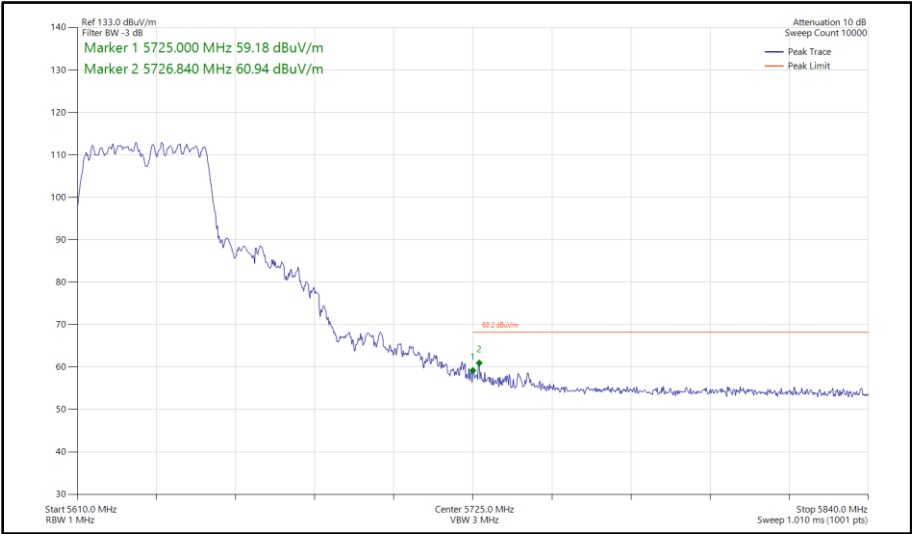
Figure 531 - 802.11n HT40, CDD, Core 0 - Core 1 - 5630 MHz Band Edge Frequency 5725 MHz
