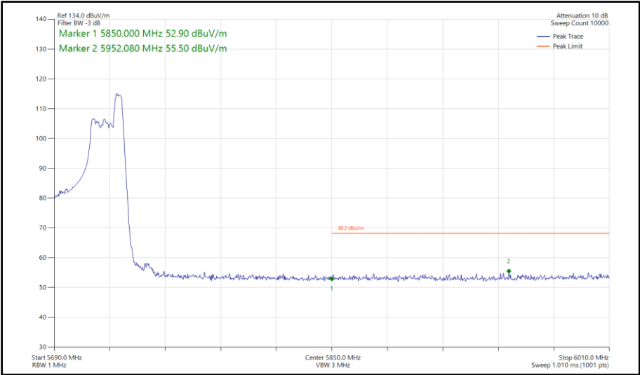
Figure 498 - 802.11ax HE40, RU 52-44, SISO, Core 0 - 5710 MHz Band Edge Frequency 5850 MHz
