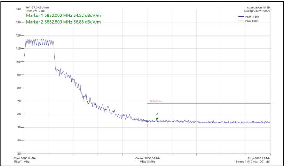
Figure 538 - 802.11ax HE40, SU, CDD, Core 0 - Core 1 - 5710 MHz Band Edge Frequency 5850 MHz
