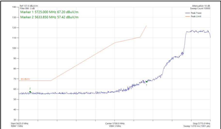
Figure 549 - 802.11ax HE20, SU, SDM, Core 0 - Core 1 - 5765 MHz Band Edge Frequency 5725 MHz
