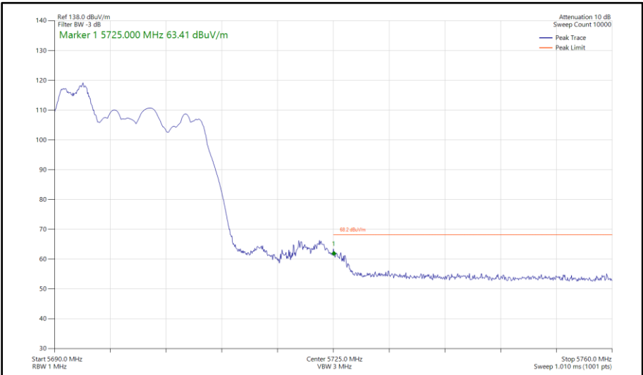
Figure 555 - 802.11ax HE20, RU 52-37, SDM, Core 0 - Core 1 - 5700 MHz Band Edge Frequency 5725 MHz
