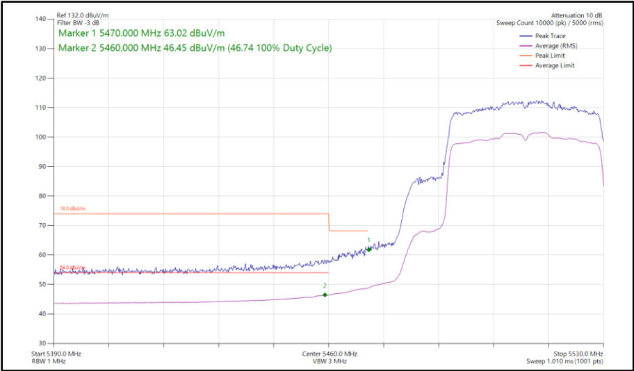
Figure 503 - 802.11ax HE40, SU, SISO, Core 1 - 5510 MHz Band Edge Frequency 5470 MHz
