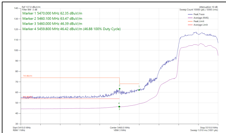
Figure 543 - 802.11ax HE20, SU, SDM, Core 0 - Core 1 - 5500 MHz Band Edge Frequency 5470 MHz
