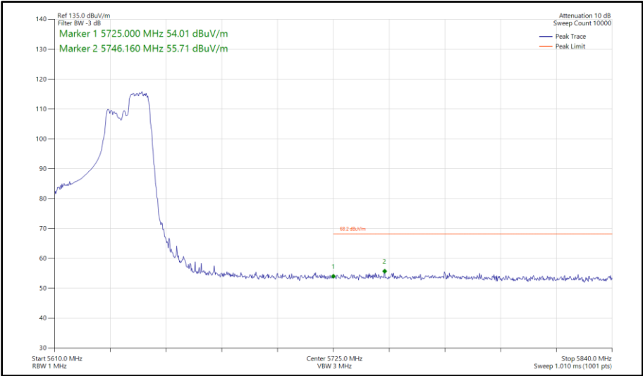
Figure 513 - 802.11ax HE40, RU 106-56, SISO, Core 1 - 5630 MHz Band Edge Frequency 5725 MHz
