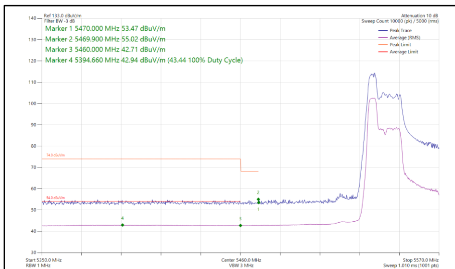
Figure 506 - 802.11ax HE40, RU 52-37, SISO, Core 1 - 5550 MHz Band Edge Frequency 5470 MHz
