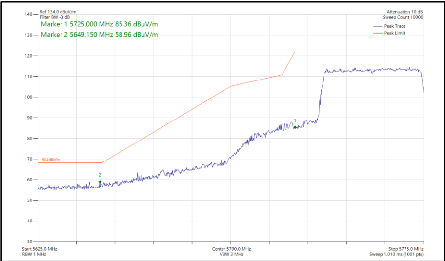
Figure 508 - 802.11ax HE40, SU, SISO, Core 1 - 5755 MHz Band Edge Frequency 5725 MHz
