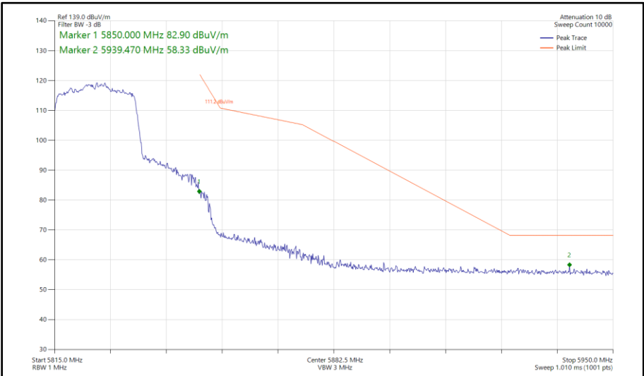
Figure 561 - 802.11ax HE20, SU, SDM, Core 0 - Core 1 - 5825 MHz Band Edge Frequency 5850 MHz
