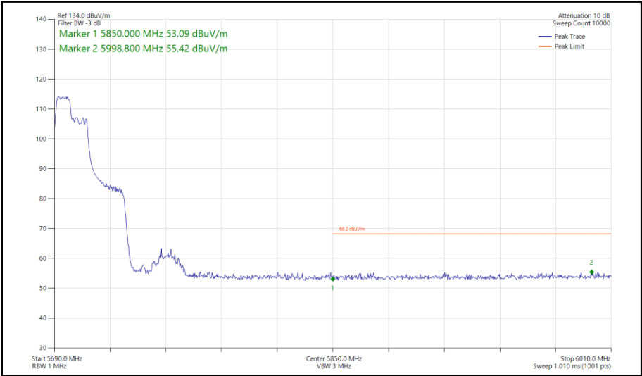
Figure 519 - 802.11ax HE40, RU 106-53, SISO, Core 1 - 5710 MHz Band Edge Frequency 5850 MHz
