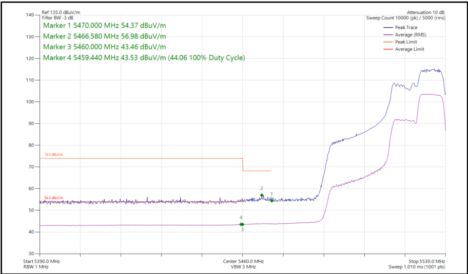
Figure 504 - 802.11ax HE40, RU 106-56, SISO, Core 1 - 5510 MHz Band Edge Frequency 5470 MHz
