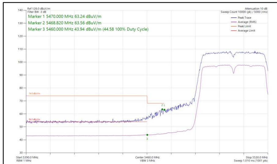
Figure 501 - 802.11n HT40, SISO, Core 1 - 5510 MHz Band Edge Frequency 5470 MHz
