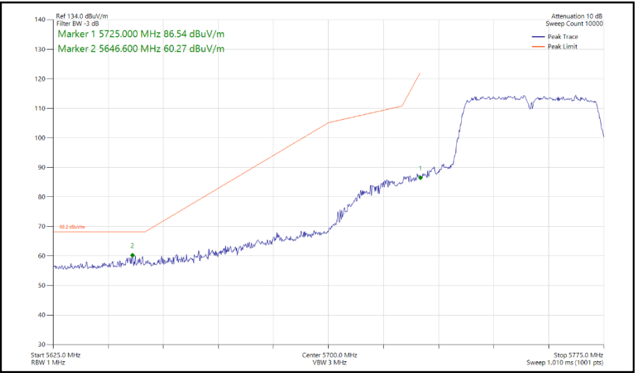
Figure 486 - 802.11n HT40, SISO, Core 0 - 5755 MHz Band Edge Frequency 5725 MHz
