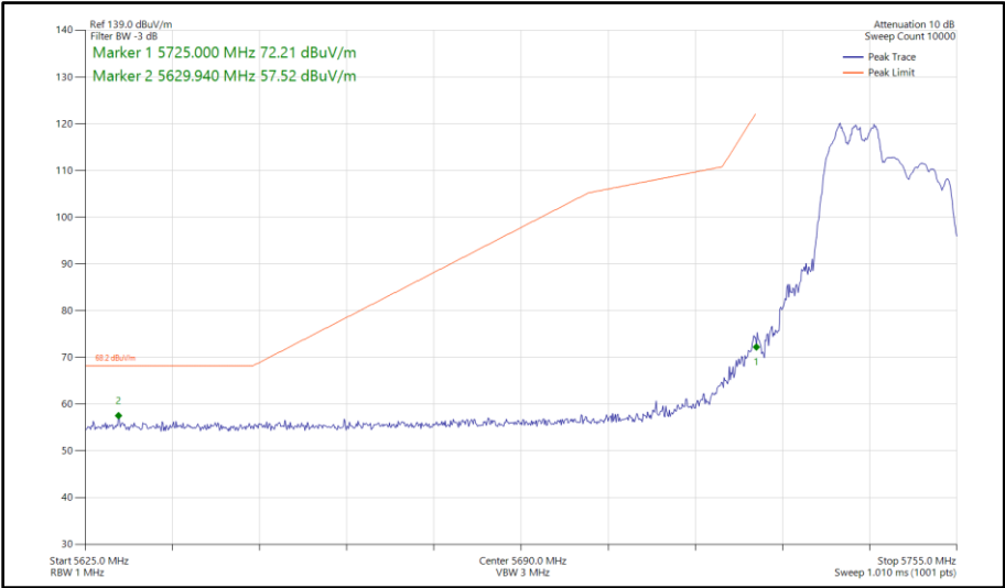
Figure 548 - 802.11ax HE20, RU 106-53, SDM, Core 0 - Core 1 - 5745 MHz Band Edge Frequency 5725 MHz
