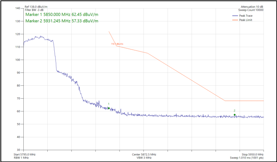
Figure 560 - 802.11ax HE20, SU, SDM, Core 0 - Core 1 - 5805 MHz Band Edge Frequency 5850 MHz
