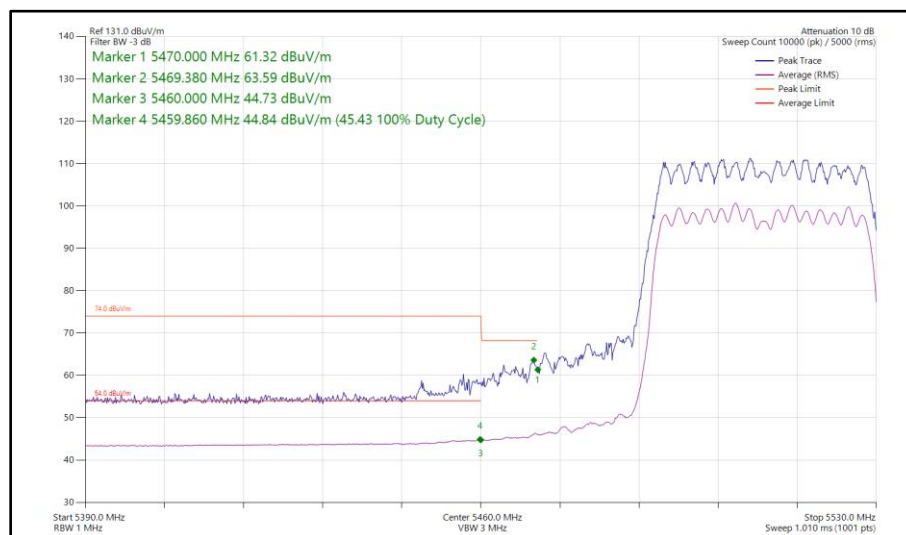
Figure 524 - 802.11ax HE40, SU, CDD, Core 0 - Core 1 - 5510 MHz Band Edge Frequency 5470 MHz
