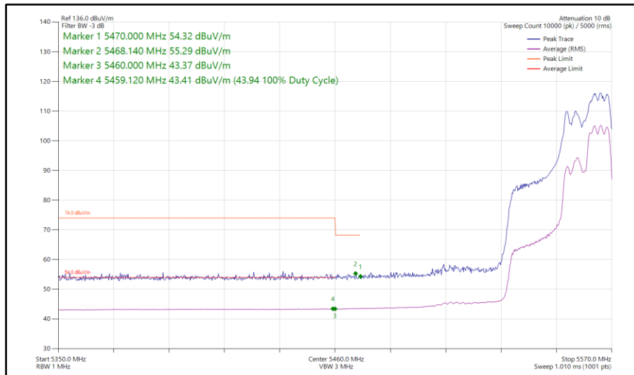
Figure 527 - 802.11ax HE40, RU 106-56, CDD, Core 0 - Core 1 - 5550 MHz Band Edge Frequency 5470 MHz
