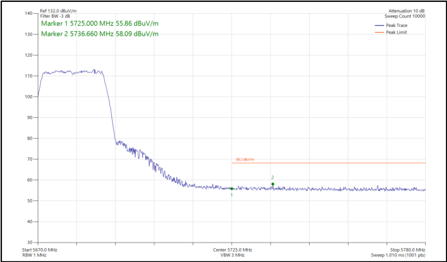
Figure 550 - 802.11n HT20, SDM, Core 0 - Core 1 - 5680 MHz Band Edge Frequency 5725 MHz
