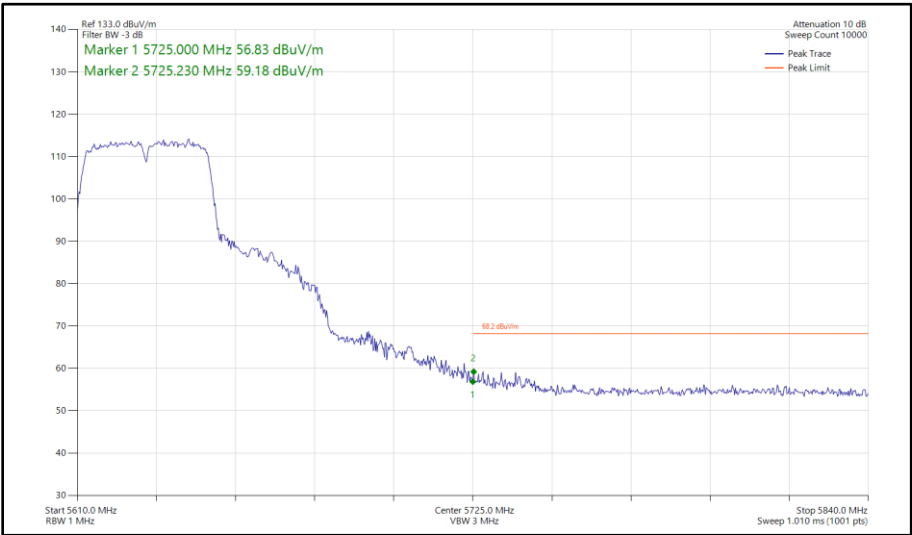
Figure 510 - 802.11n HT40, SISO, Core 1 - 5630 MHz Band Edge Frequency 5725 MHz
