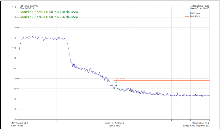
Figure 532 - 802.11n HT40, CDD, Core 0 - Core 1 - 5670 MHz Band Edge Frequency 5725 MHz
