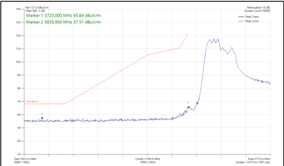
Figure 530 - 802.11ax HE40, RU 106-53, CDD, Core 0 - Core 1 - 5755 MHz Band Edge Frequency 5725 MHz
