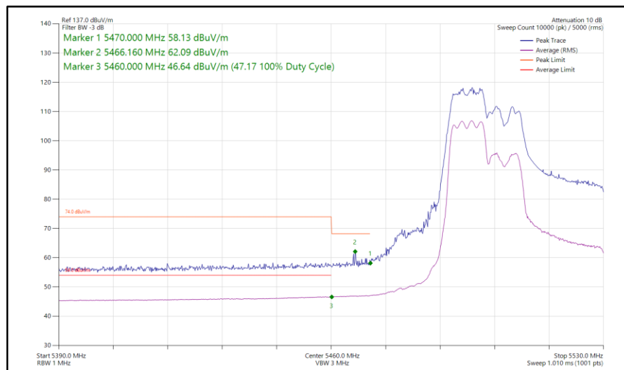
Figure 525 - 802.11ax HE40, RU 106-53, CDD, Core 0 - Core 1 - 5510 MHz Band Edge Frequency 5470 MHz
