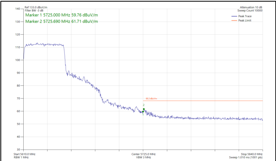
Figure 512 - 802.11ax HE40, SU, SISO, Core 1 - 5630 MHz Band Edge Frequency 5725 MHz
