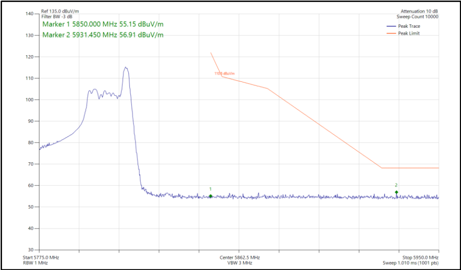
Figure 500 - 802.11ax HE40, RU 26-17, SISO, Core 0 - 5795 MHz Band Edge Frequency 5850 MHz
