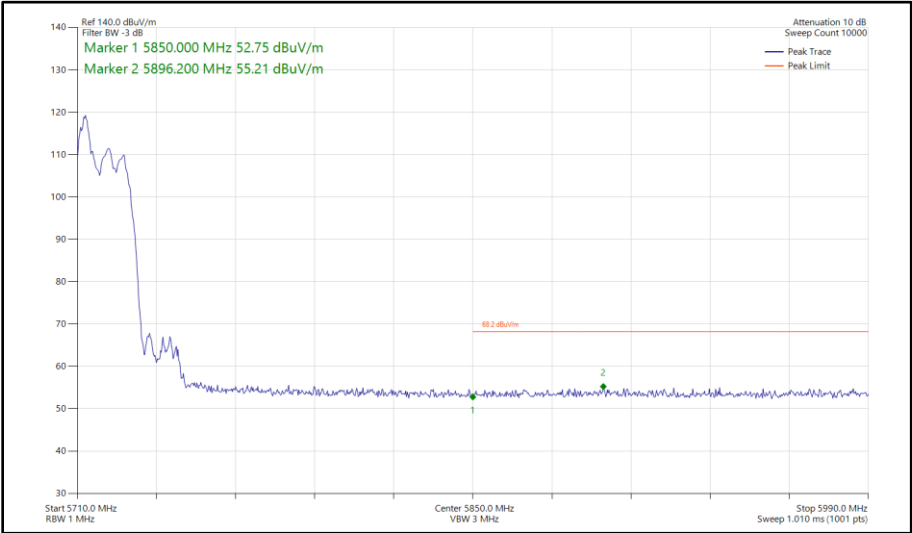
Figure 559 - 802.11ax HE20, RU 52-37, SDM, Core 0 - Core 1 - 5720 MHz Band Edge Frequency 5850 MHz
