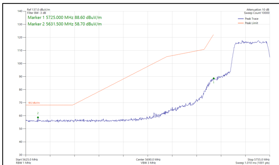
Figure 547 - 802.11n HT20, SDM, Core 0 - Core 1 - 5745 MHz Band Edge Frequency 5725 MHz
