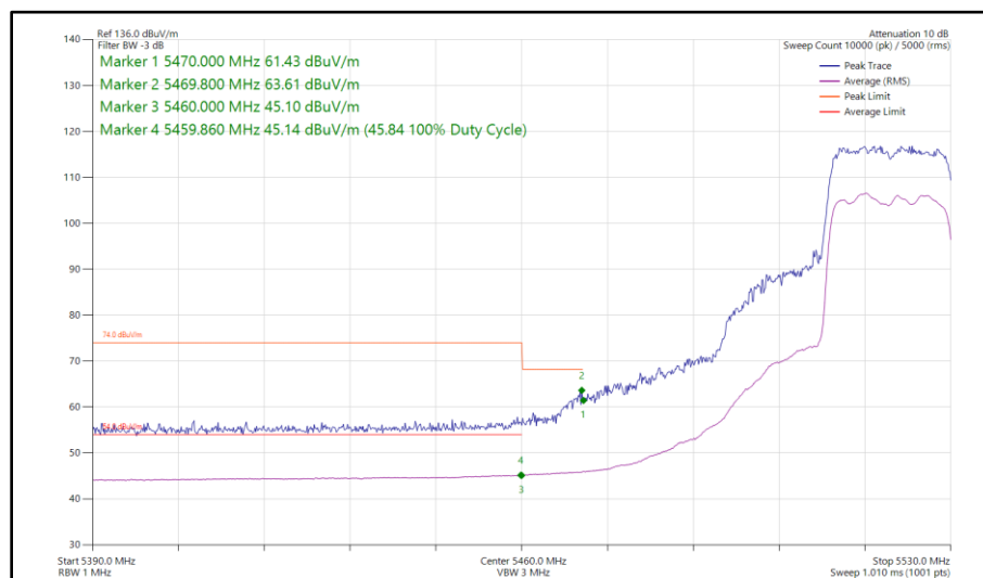
Figure 545 - 802.11ax HE20, SU, SDM, Core 0 - Core 1 - 5520 MHz Band Edge Frequency 5470 MHz
