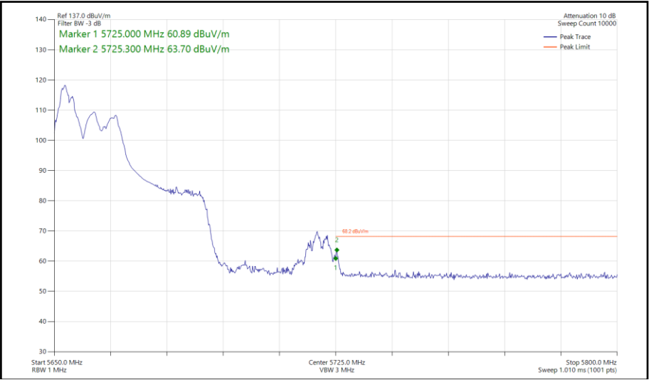
Figure 535 - 802.11ax HE40, RU 52-37, CDD, Core 0 - Core 1 - 5670 MHz Band Edge Frequency 5725 MHz
