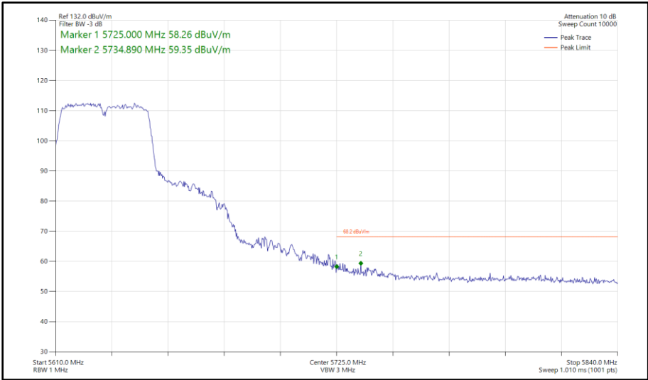
Figure 489 - 802.11n HT40, SISO, Core 0 - 5630 MHz Band Edge Frequency 5725 MHz
