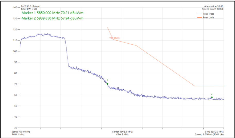
Figure 520 - 802.11ax HE40, SU, SISO, Core 1 - 5795 MHz Band Edge Frequency 5850 MHz
