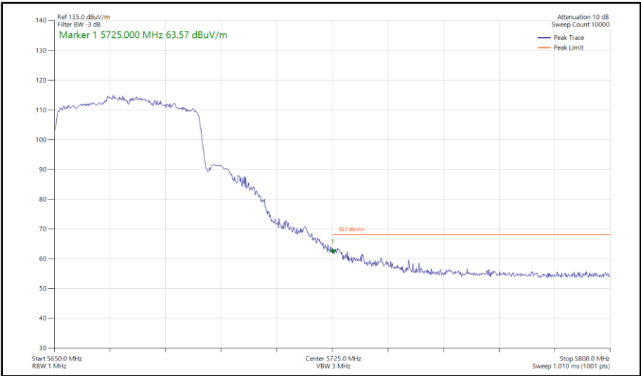
Figure 514 - 802.11ax HE40, SU, SISO, Core 1 - 5670 MHz Band Edge Frequency 5725 MHz
