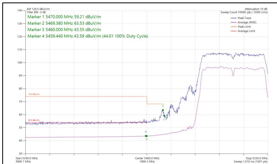
Figure 563 - 802.11ac VHT40, TxBF, Core 0 - Core 1 - 5510 MHz Band Edge Frequency 5470 MHz
