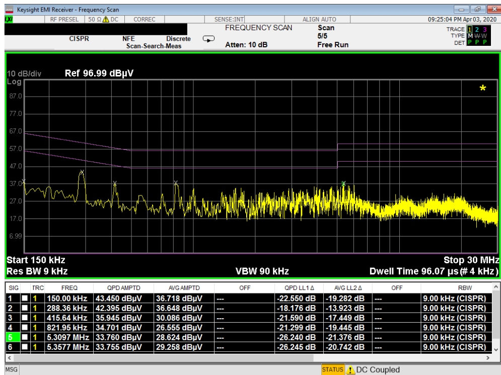
Plot 7-48. Line Conducted Plot with 802.11b (N)
