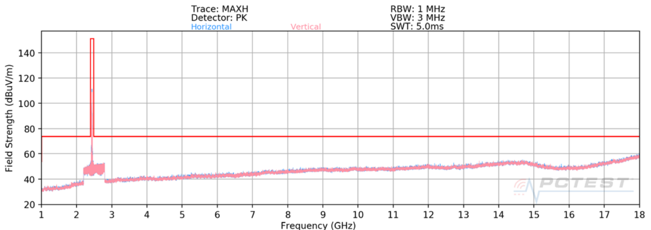
Plot 7-37. Radiated Spurious Plot above 1GHz (802.11b – Ch. 11)
