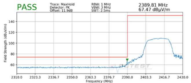
Plot 7-40. Radiated Restricted Lower Band Edge Measurement (Peak)
