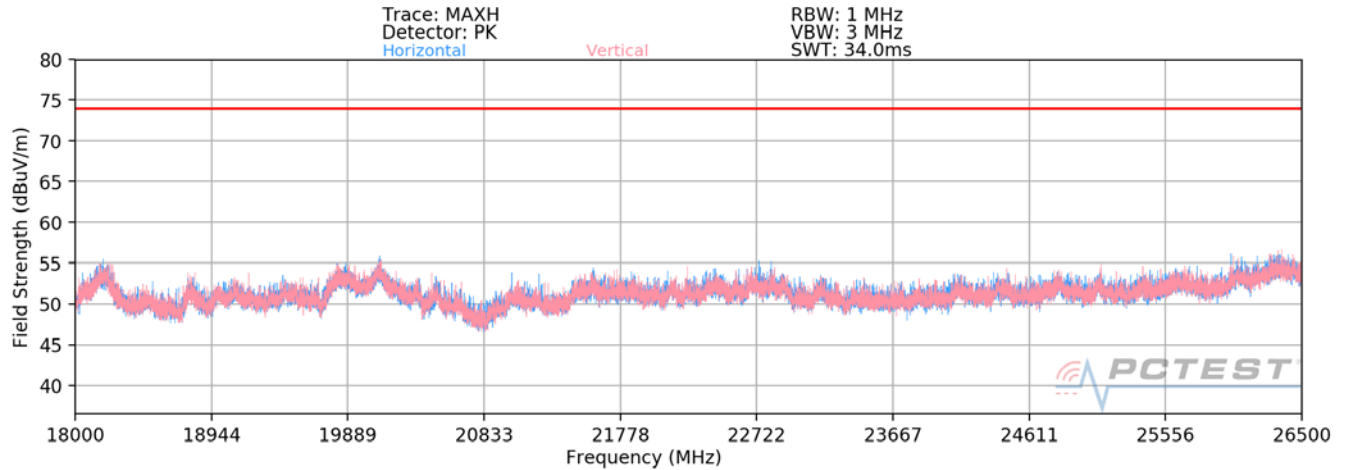
Plot 7-38. Radiated Spurious Plot above 18GHz
