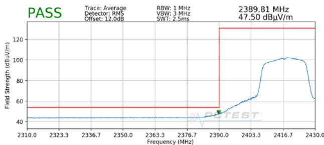
Plot 7-41. Radiated Restricted Lower Band Edge Measurement (Average)
