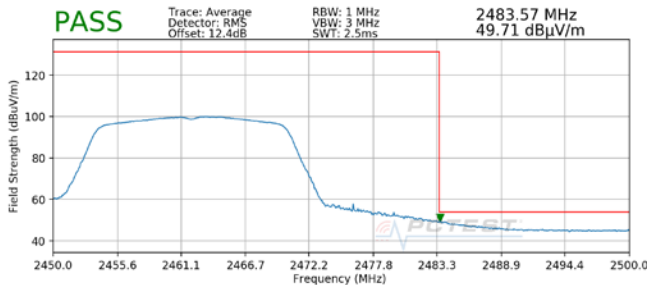
Plot 7-45. Radiated Restricted Upper Band Edge Measurement (Average)
