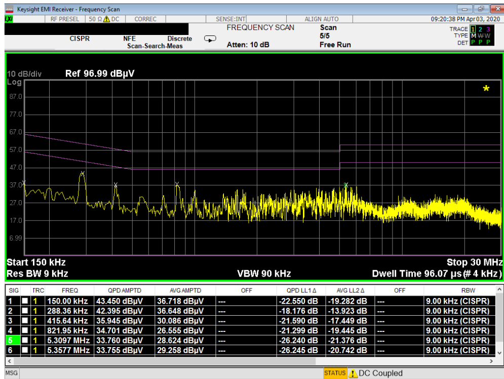
Plot 7-47. Line Conducted Plot with 802.11b (L1)
