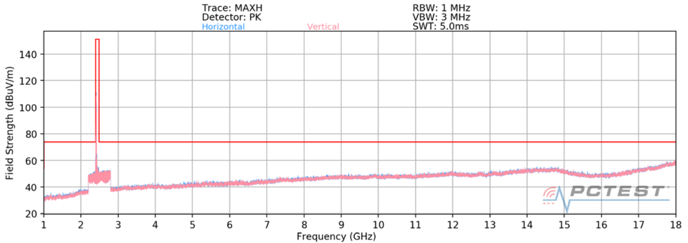
Plot 7-35. Radiated Spurious Plot above 1GHz (802.11b – Ch. 1)
