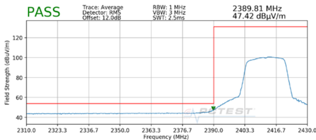
Plot 7-39. Radiated Restricted Lower Band Edge Measurement (Average)
