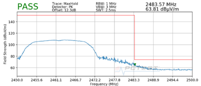
Plot 7-46. Radiated Restricted Upper Band Edge Measurement (Peak)
