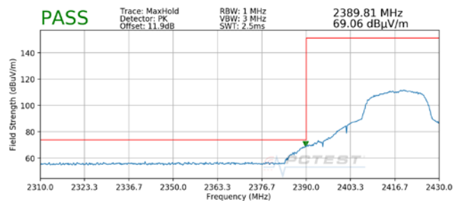
Plot 7-42. Radiated Restricted Lower Band Edge Measurement (Peak)
