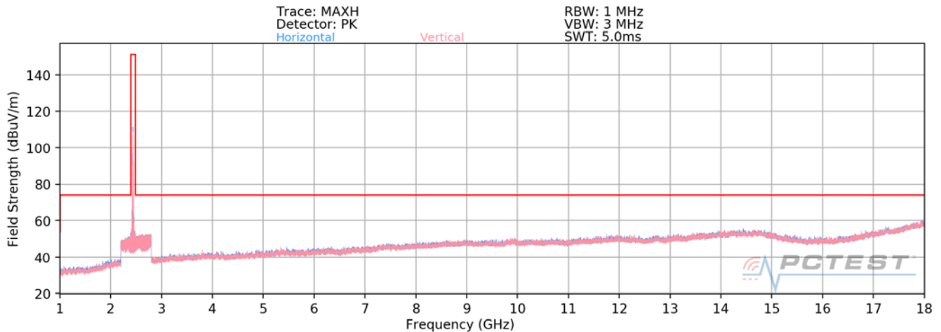
Plot 7-36. Radiated Spurious Plot above 1GHz (802.11b – Ch. 6)
