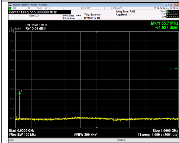
41-41-20MHz-20MHz-64QAM-64QAM-40942-41140-1RB #0-ORB#0-30~1000MHz-PASS
