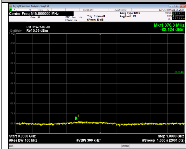
41-41-20MHz-20MHz-16QAM-16QAM-40641-40839-1RB #0-0RB#0-30~1000MHz-PASS
