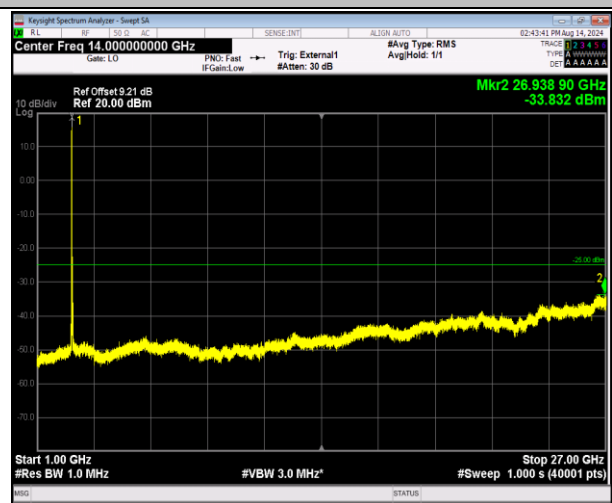
41-41-20MHz-20MHz-16QAM-16QAM-40641-40839-1RB#0 -0RB#0-1000~27000MHz-PASS
