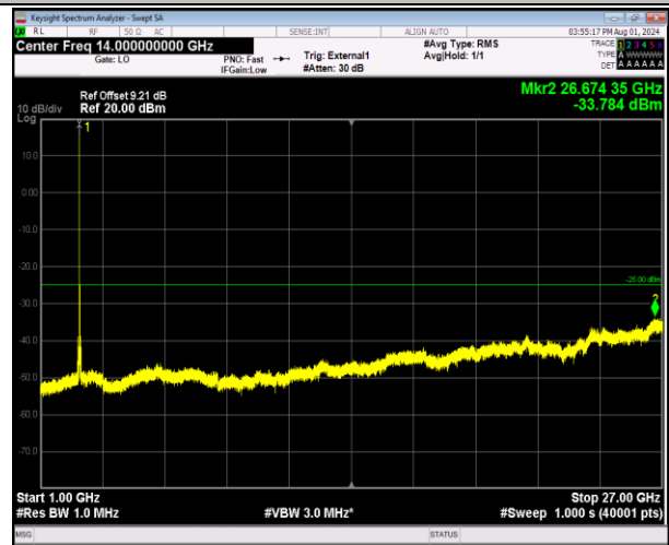
41-41-20MHz-20MHz-64QAM-64QAM-40942-41140-1RB#0 -ORB#0-1000~27000MHz-PASS
