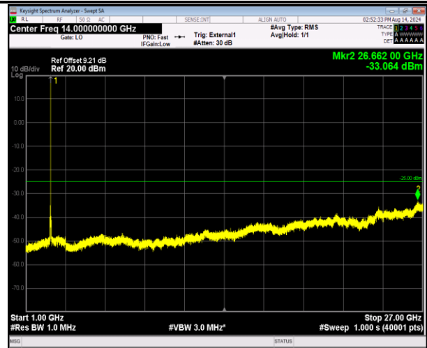
41-41-20MHz-20MHz-16QAM-16QAM-40942-41140-1RB#9 9-ORB#0-1000~27000MHz-PASS
