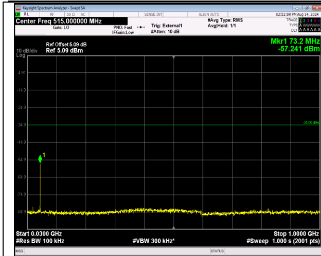
41-41-20MHz-20MHz-16QAM-16QAM-40942-41140-1RB #99-ORB#0-30~1000MHz-PASS
