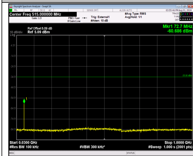
41-41-20MHz-20MHz-64QAM-64QAM-40942-41140-1RB #99-0RB#0-30~1000MHz-PASS
