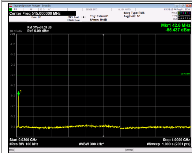
41-41-20MHz-20MHz-64QAM-64QAM-40641-40839-1RB #99-0RB#0-30~1000MHz-PASS
