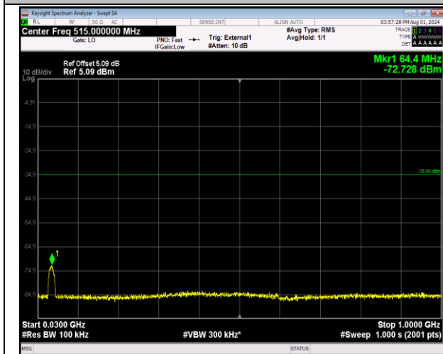
41-41-20MHz-20MHz-64QAM-64QAM-40942-41140-100 RB#0-100RB#0-30~1000MHz-PASS
