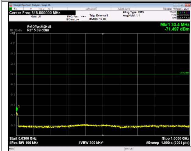
41-41-20MHz-20MHz-64QAM-64QAM-40641-40839-100 RB#0-100RB#0-30~1000MHz-PASS
