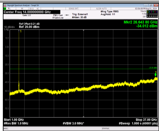
41-41-20MHz-20MHz-64QAM-64QAM-40942-41140-1RB#9 9-0RB#0-1000~27000MHz-PASS
