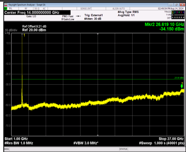
41-41-20MHz-20MHz-QPSK-QPSK-40942-41140-1RB#0-0 RB#0-1000~27000MHz-PASS
