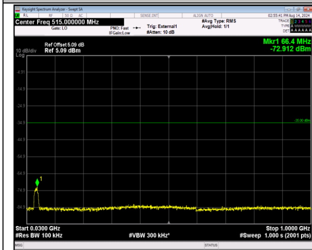
41-41-20MHz-20MHz-16QAM-16QAM-40942-41140-100 RB#0-100RB#0-30~1000MHz-PASS
