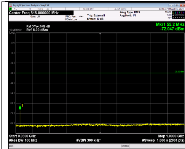
41-41-20MHz-20MHz-64QAM-64QAM-40942-41140-1RB #0-1RB#99-30~1000MHz-PASS
