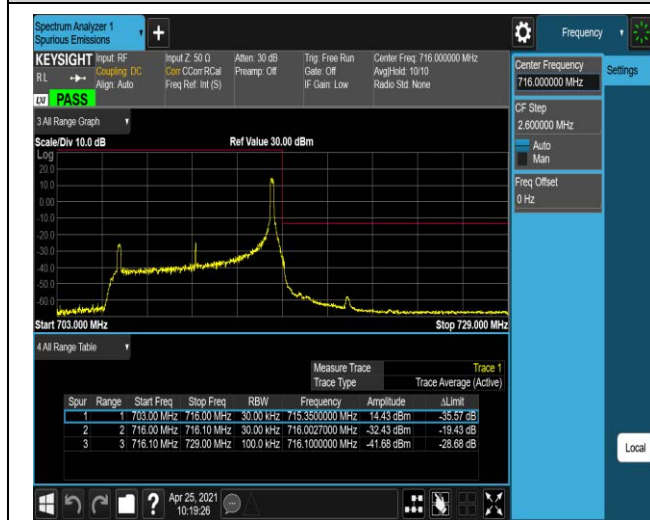
Band17-10MHz-16QAM-23800-1RB#49
