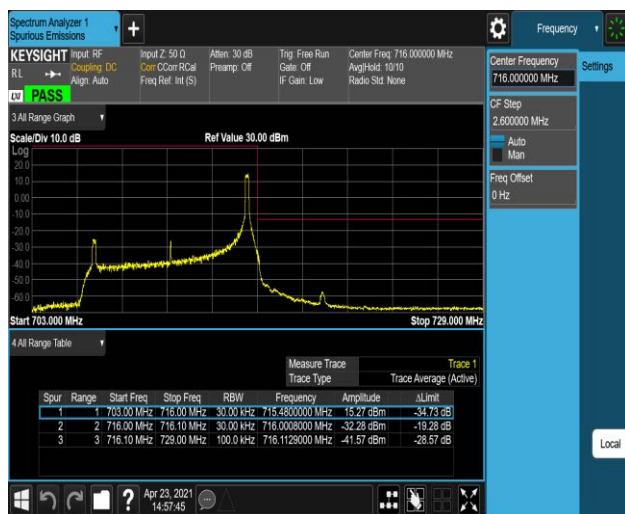
Band17-5MHz-QPSK-23755-1RB#0
