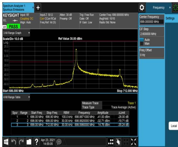
Band12-10MHz-16QAM-23060-50RB#0
