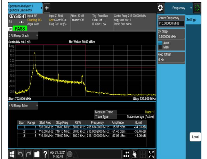
Band12-10MHz-QPSK-23130-50RB#0
