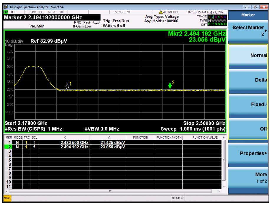
(PEAK, Channel 39)
