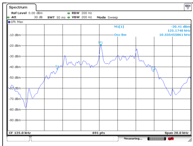
INT1 Antenna
