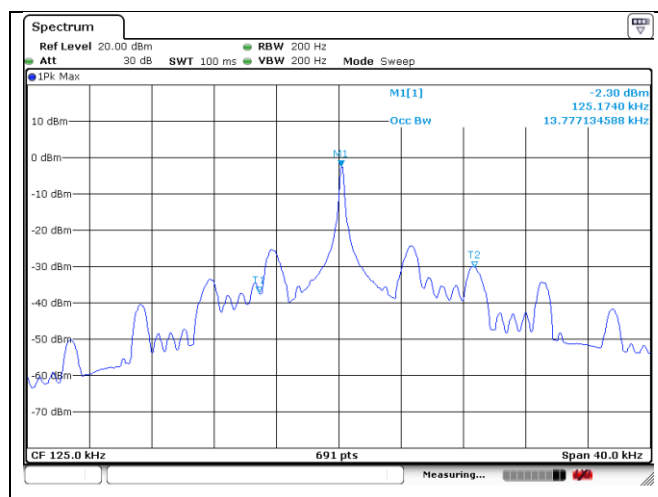
SSB Antenna
