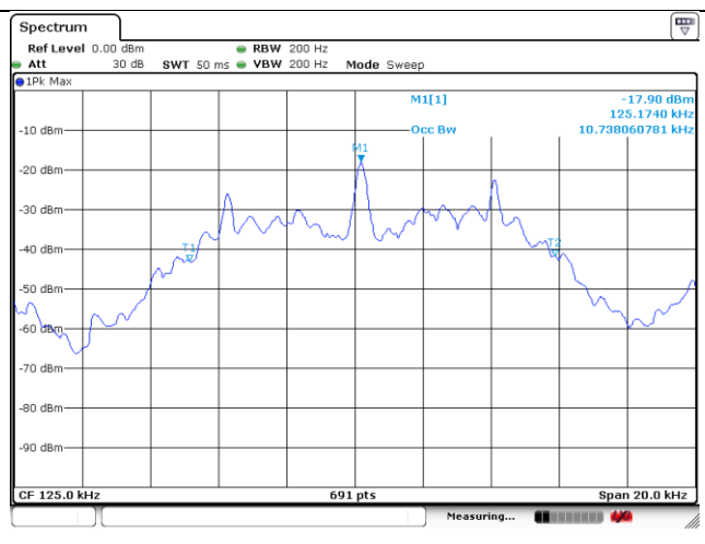
INT2 Antenna
