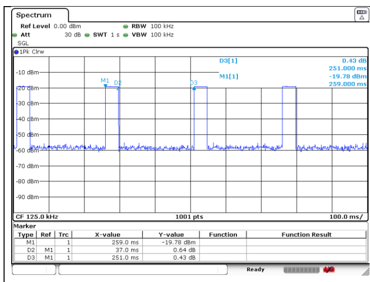
INT1 Antenna
