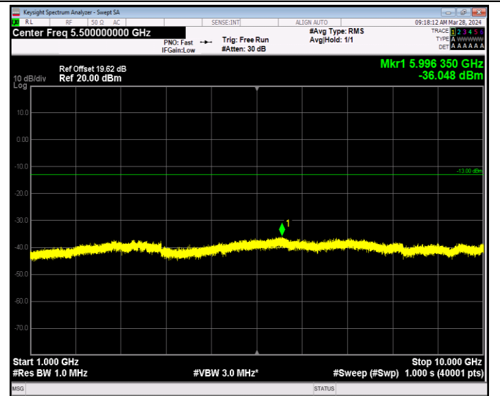
Band13_10MHz_64QAM_23230_1RB#0_1000~10000_1000~10000
