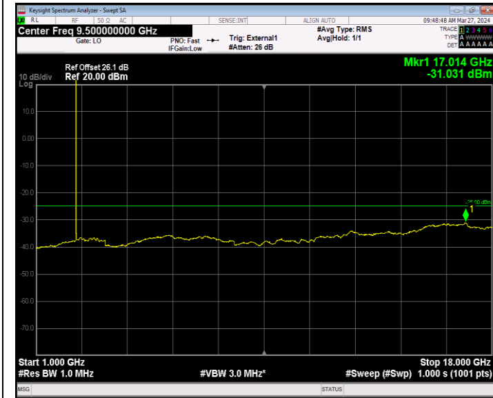
Band41_5MHz_16QAM_39675_1RB#0_1000~18000_1000~18000 0
