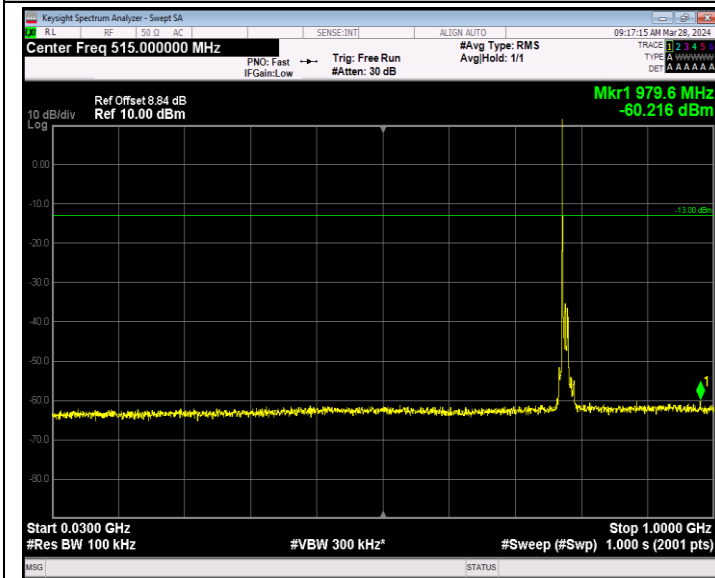
Band13_10MHz_QPSK_23230_1RB#0_30~1000_30~1000
