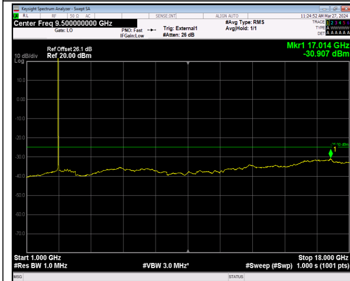
Band41_20MHz_QPSK_41490_1RB#0_1000~18000_1000~18000
