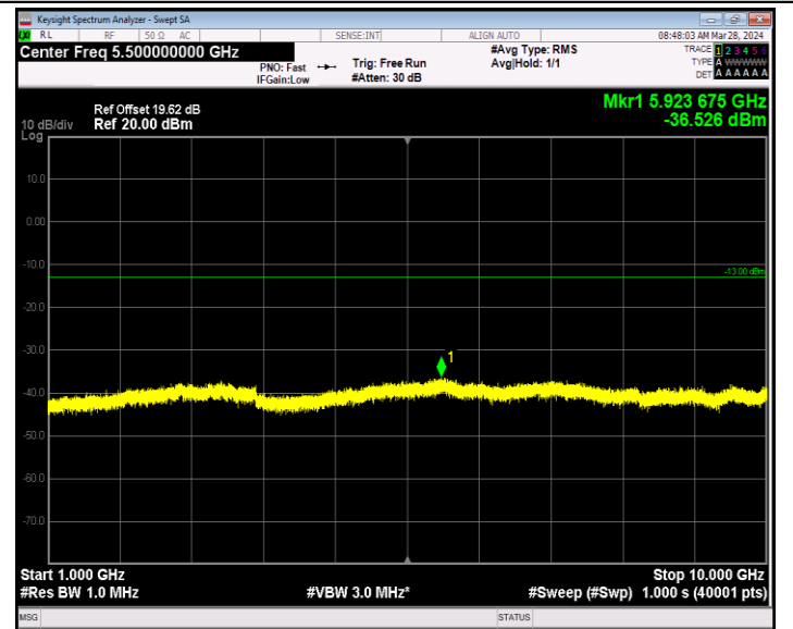
Band12_10MHz_64QAM_23095_1RB#0_1000~10000_1000~10000
