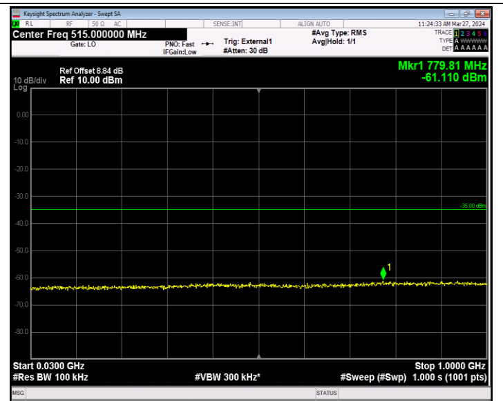
Band41_20MHz_QPSK_41490_1RB#0_30~1000_30~1000
