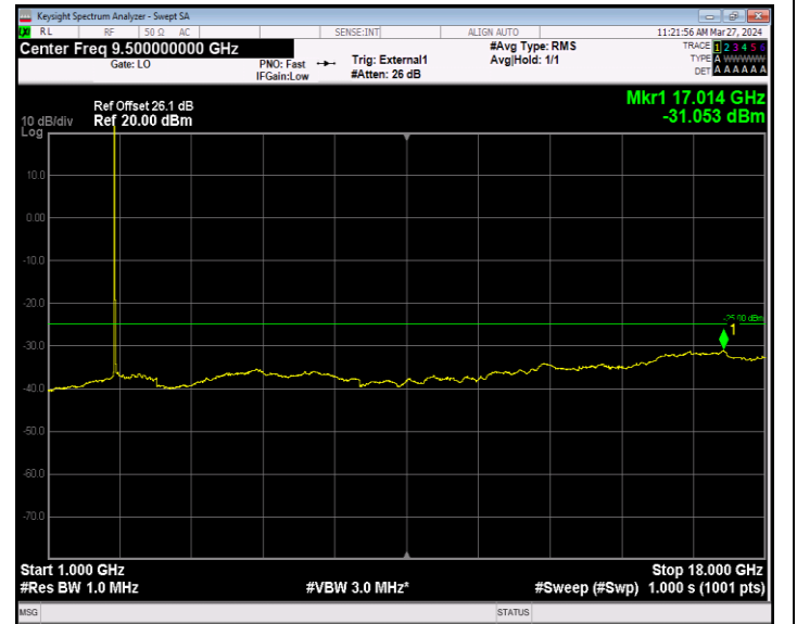
Band41_20MHz_QPSK_40620_1RB#0_1000~18000_1000~1800 0
