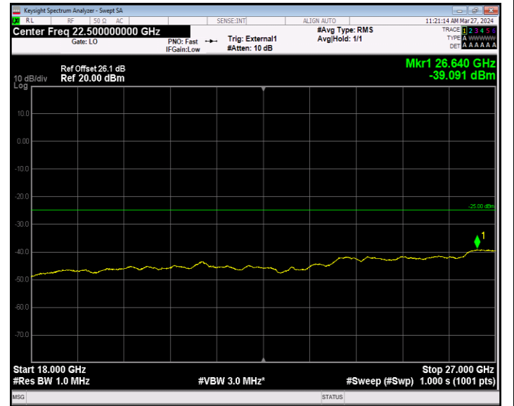
Band41_20MHz_64QAM_39750_1RB#0_18000~27000_18000~27000
