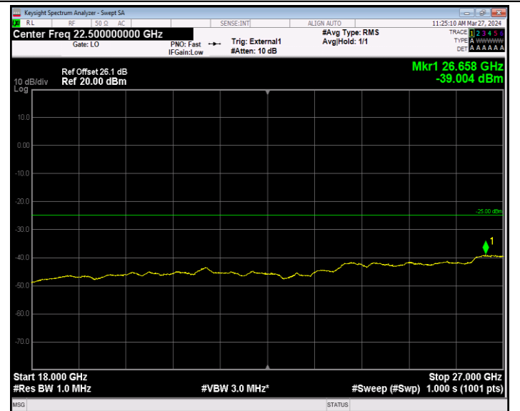
Band41_20MHz_QPSK_41490_1RB#0_18000~27000_18000~27000
