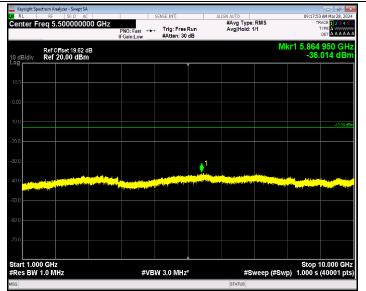
Band13_10MHz_16QAM_23230_1RB#0_1000~10000_1000~10000
