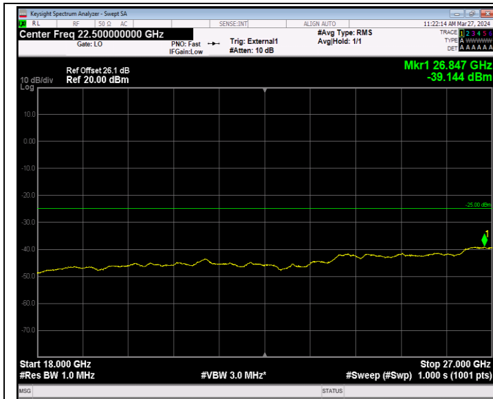
Band41_20MHz_QPSK_40620_1RB#0_18000~27000_18000~27000
