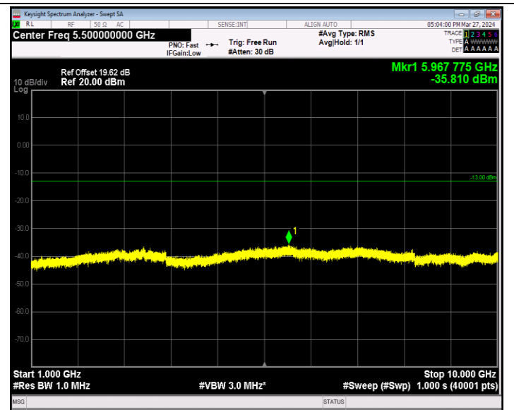
Band12_1.4MHz_64QAM_23095_1RB#0_1000~10000_1000~10000
