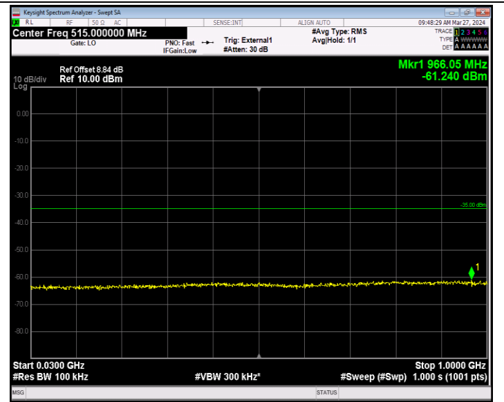
Band41_5MHz_16QAM_39675_1RB#0_30~1000_30~1000
