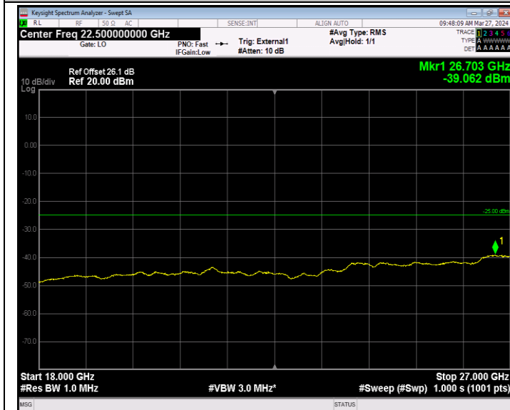
Band41_5MHz_QPSK_39675_1RB#0_18000~27000_18000~27000 00
