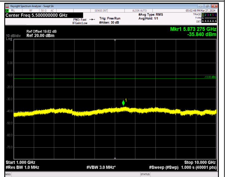
Band12_1.4MHz_64QAM_23017_1RB#0_1000~10000_1000~10000
