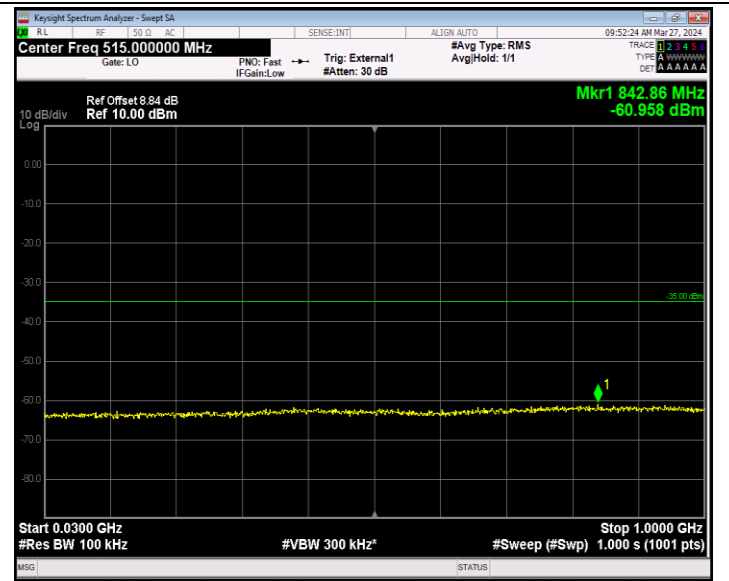
Band41_5MHz_64QAM_40620_1RB#0_30~1000_30~1000
