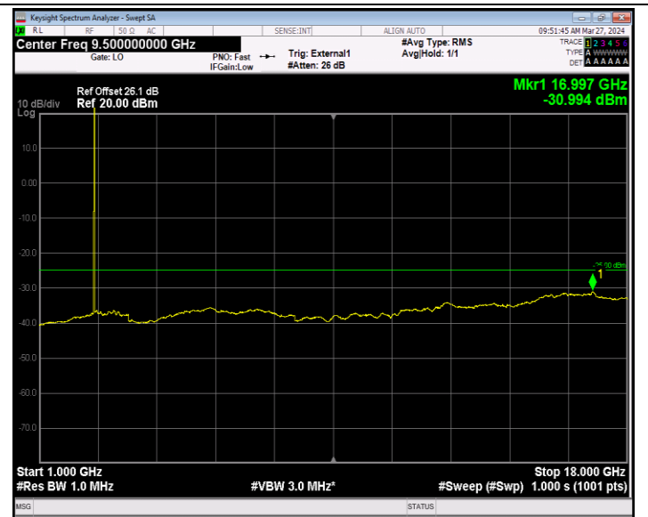
Band41_5MHz_16QAM_40620_1RB#0_1000~18000_1000~18000
