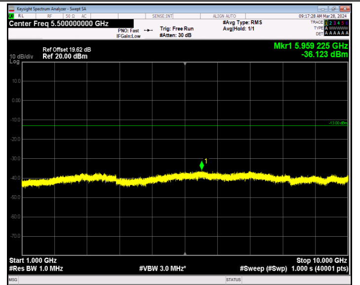
Band13_10MHz_QPSK_23230_1RB#0_1000~10000_1000~10000
