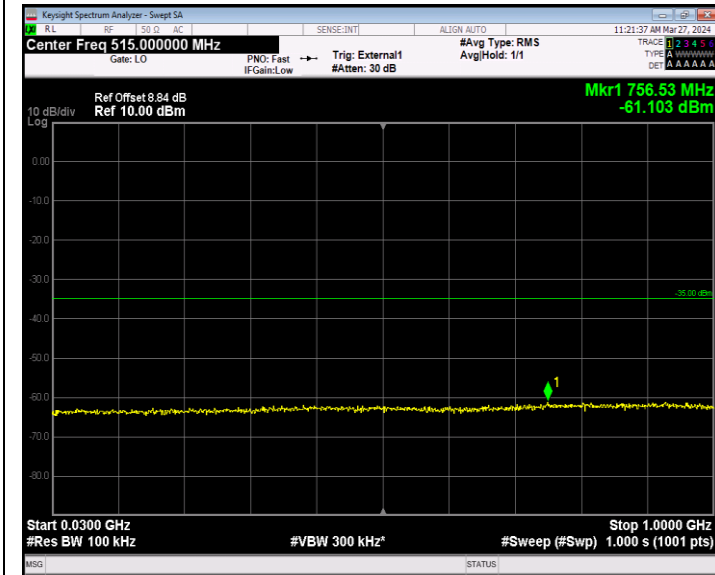
Band41_20MHz_QPSK_40620_1RB#0_30~1000_30~1000
