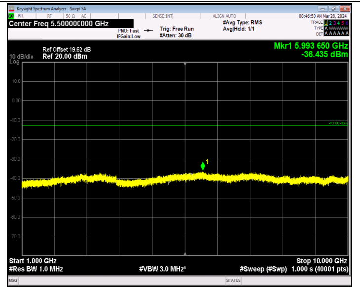
Band12_10MHz_64QAM_23060_1RB#0_1000~10000_1000~10000
