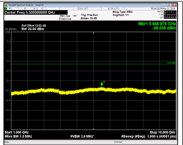
Band12_1.4MHz_16QAM_23173_1RB#0_1000~10000_1000~10000
