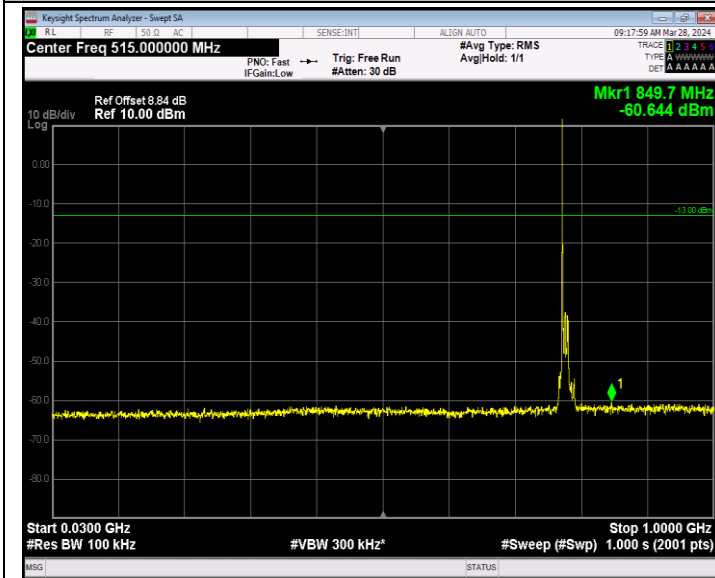
Band13_10MHz_64QAM_23230_1RB#0_30~1000_30~1000
