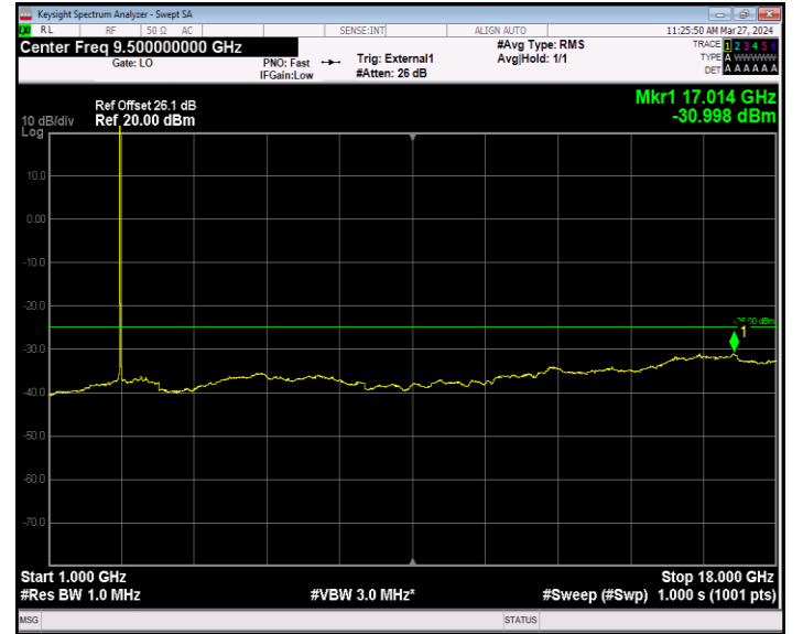
Band41_20MHz_16QAM_41490_1RB#0_1000~18000_1000~18000 00
