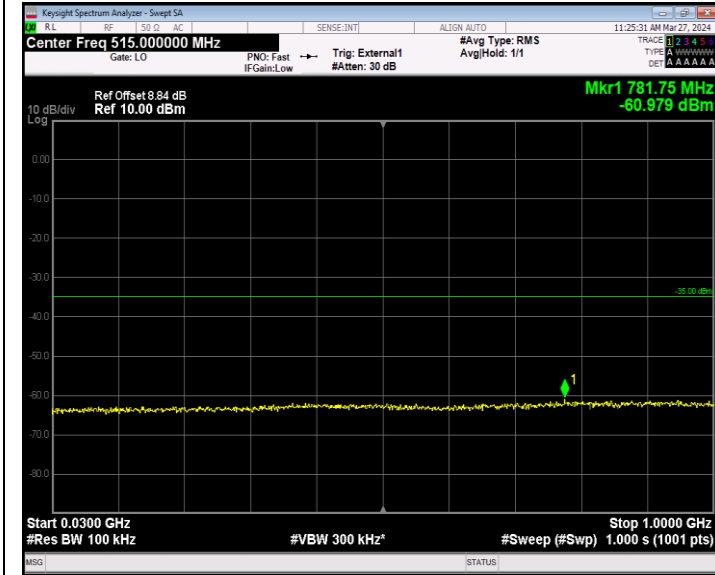
Band41_20MHz_16QAM_41490_1RB#0_30~1000_30~1000
