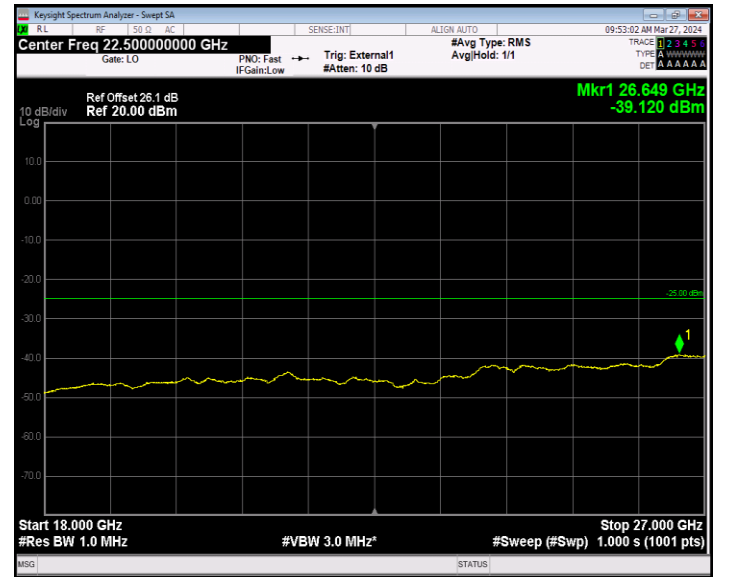
Band41_5MHz_64QAM_40620_1RB#0_18000~27000_18000~27000
