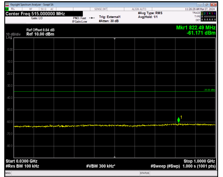
Band41_20MHz_64QAM_41490_1RB#0_30~1000_30~1000
