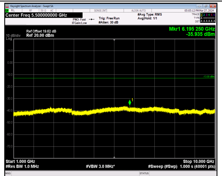
Band12_1.4MHz_64QAM_23173_1RB#0_1000~10000_1000~10000
