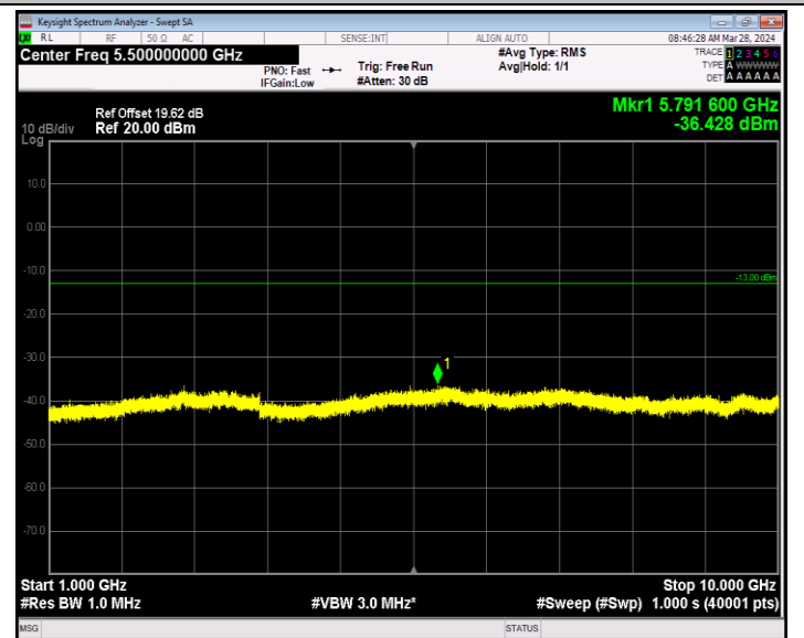
Band12_10MHz_16QAM_23060_1RB#0_1000~10000_1000~1000 00
