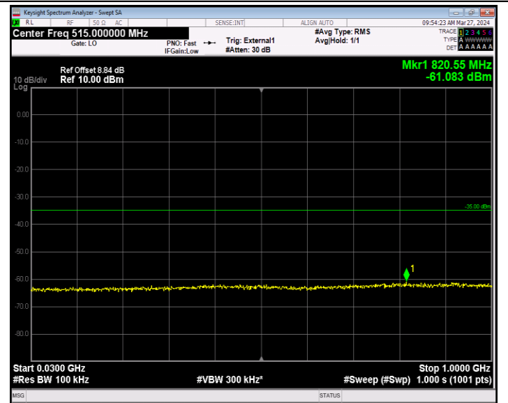
Band41_5MHz_16QAM_41565_1RB#0_30~1000_30~1000
