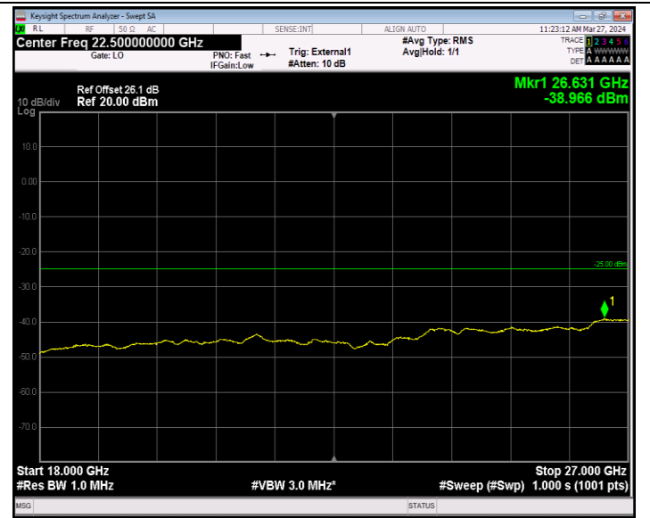
Band41_20MHz_16QAM_40620_1RB#0_18000~27000_18000~27000 7000
