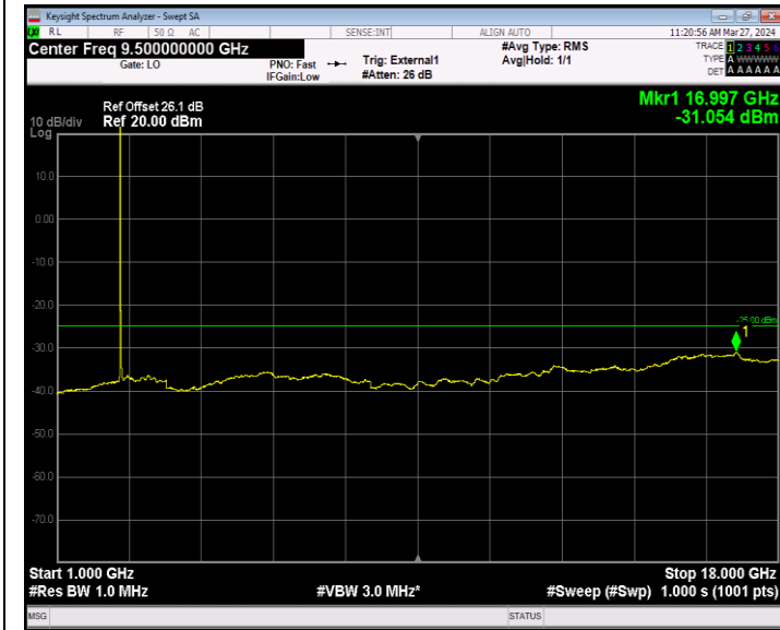
Band41_20MHz_64QAM_39750_1RB#0_1000~18000_1000~18000
