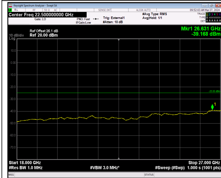
Band41_5MHz_16QAM_40620_1RB#0_18000~27000_18000~27000
