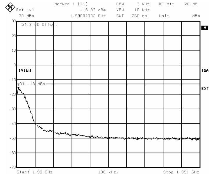
Figure 32 : +1 MHz adjacent band (Channel 810, Pmax), H4D, GMSK modulation
