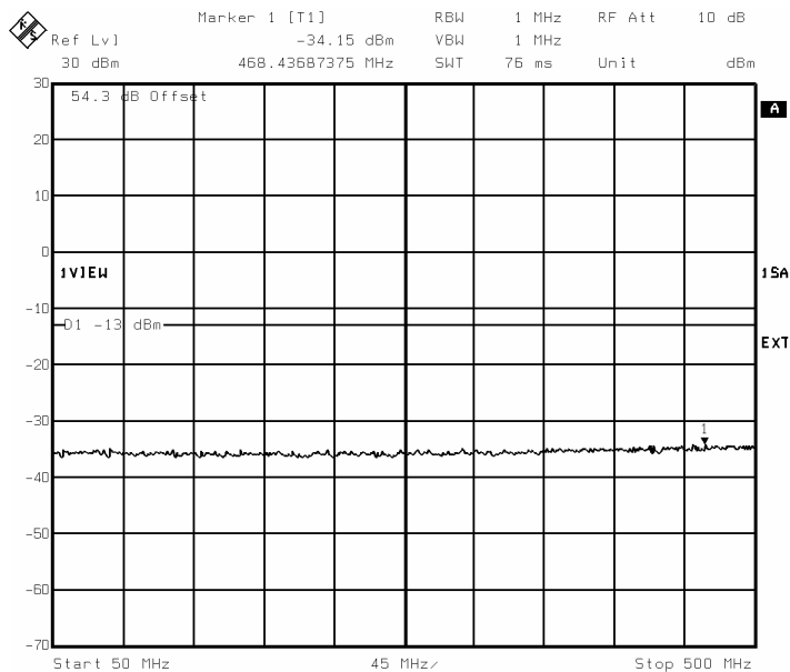
Figure 12: 50 MHz – 500 MHz
