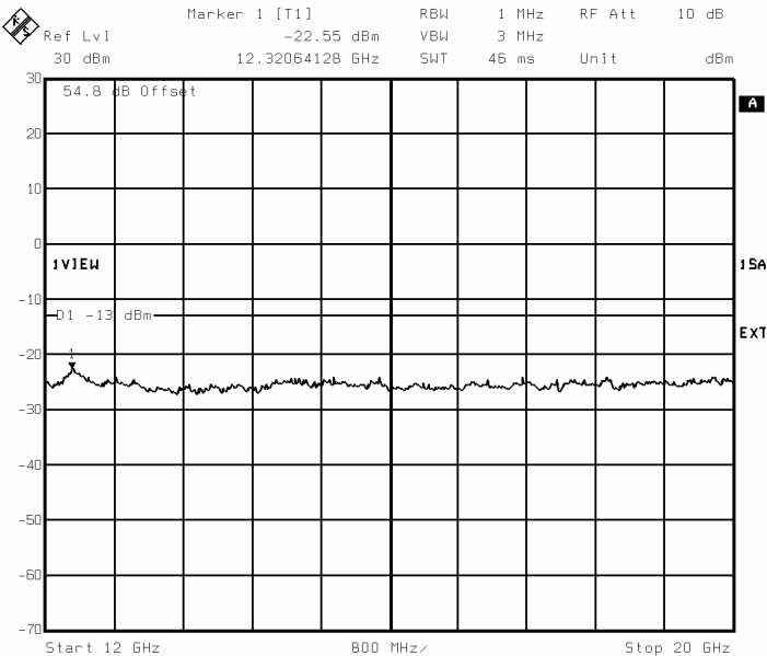
Figure 20 : 12 – 20 GHz
