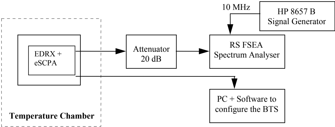
Figure 12 : Test configuration for Frequency Stability
