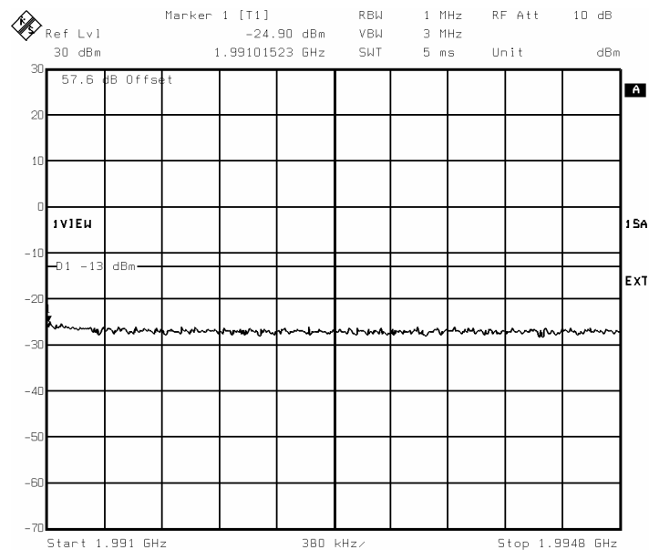
Figure 16 : 1991 – 1994.8 MHz
