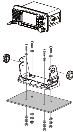
Desktop Mounting
