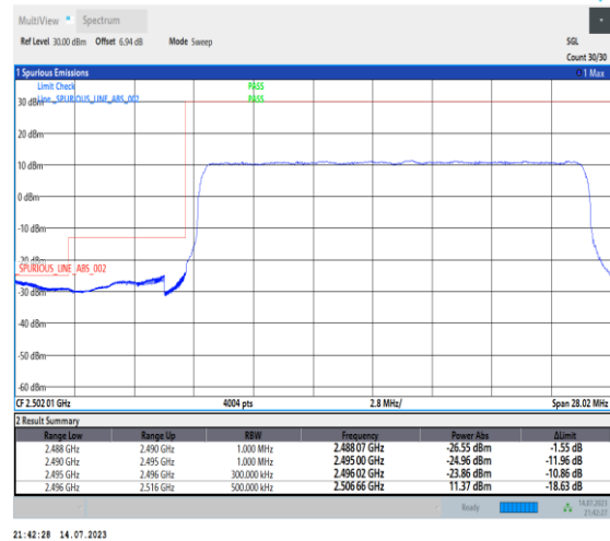
1-N41-PC1-30-20-L-3-DFT-PI2BPSK-Outer_Full-50@0-Ant0-1--PASS-see graph
