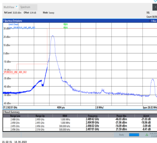
1-N41-PC1-30-20-L-4-CP-QPSK-Edge_1RB_Left-1@0-Ant0-1--PASS-see graph
