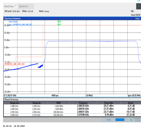
1-N41-PC1-30-20-L-6-CP-QPSK-Outer_Full-51@0-Ant0-1--PASS-see graph
