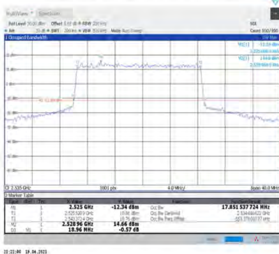
1-N7--15-20-M-1-DFT-QPSK-Outer_Full-100@0-Ant1-17.852-18.960-≤20-PASS
