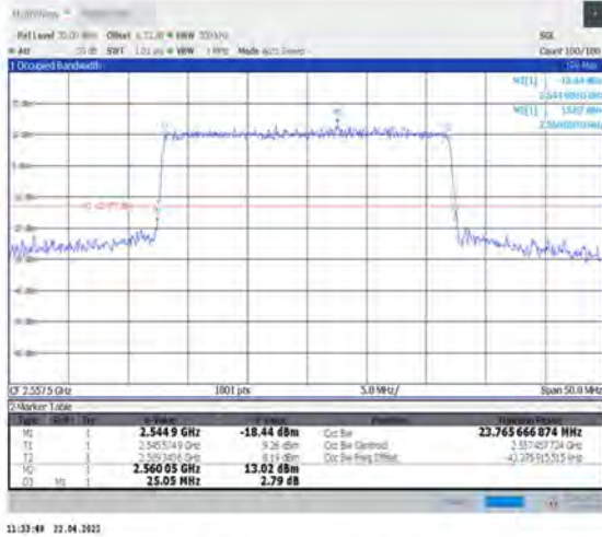
1-N7--15-25-H-7-CP-16QAM-Outer_Full-133@0-Ant1-23.766-25.050-≤25-PASS
