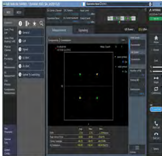
1-N7-PC3-15-40-M-1-DFT-PI2BPSK-Outer_Full-216@0-Ant1-see graph-PASS
