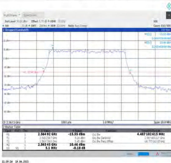
1-N7--15-5-H-5-DFT-256QAM-Outer_Full-25@0- Ant1-4.487-5.100-≤5-PASS
