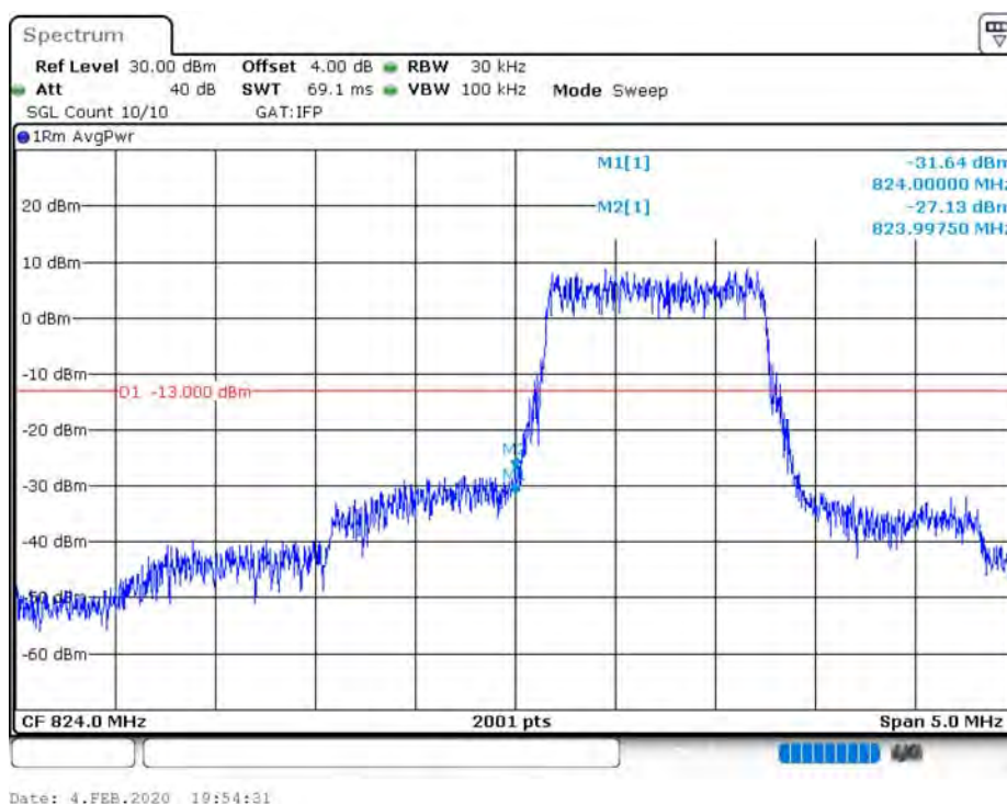
B26_CH26797_1.4M_QPSK_6RB0 (Part 22)
