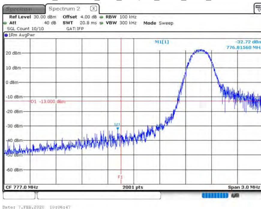
B13_CH23230_10M_16-QAM_1RB0_LOW_150k
