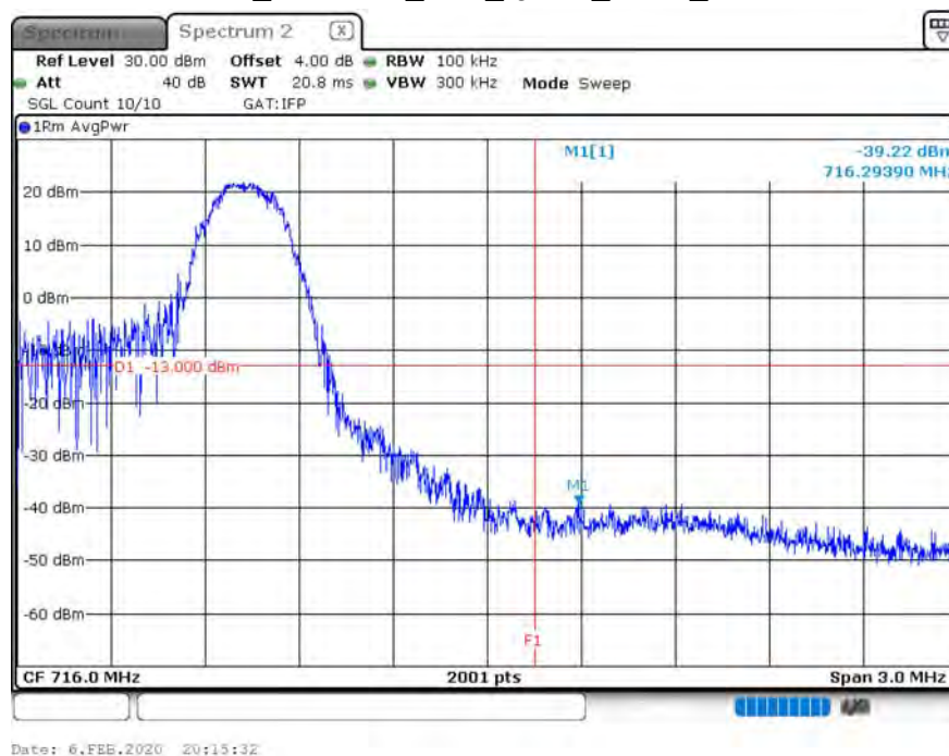
B12_CH23130_10M_QPSK_1RB5_150k
