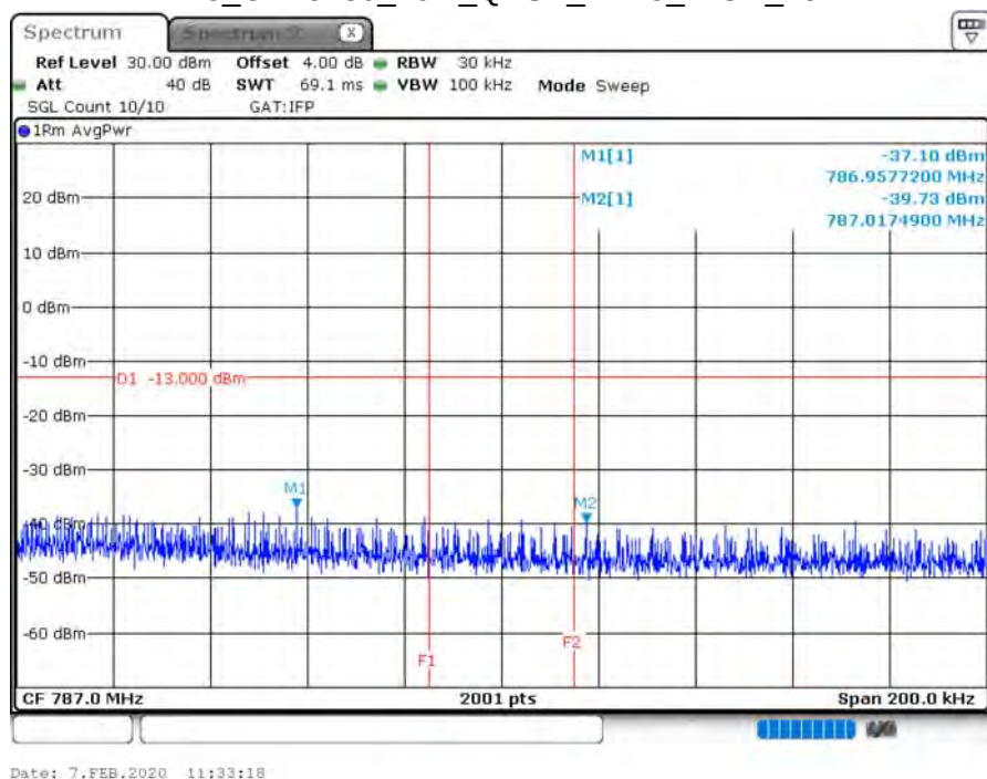
B13_CH23230_10M_QPSK_1RB5_HIGH_150k
