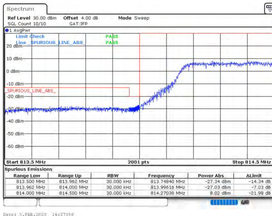
B26_CH26697_1.4M_QPSK_6RB0 (Part 90)
