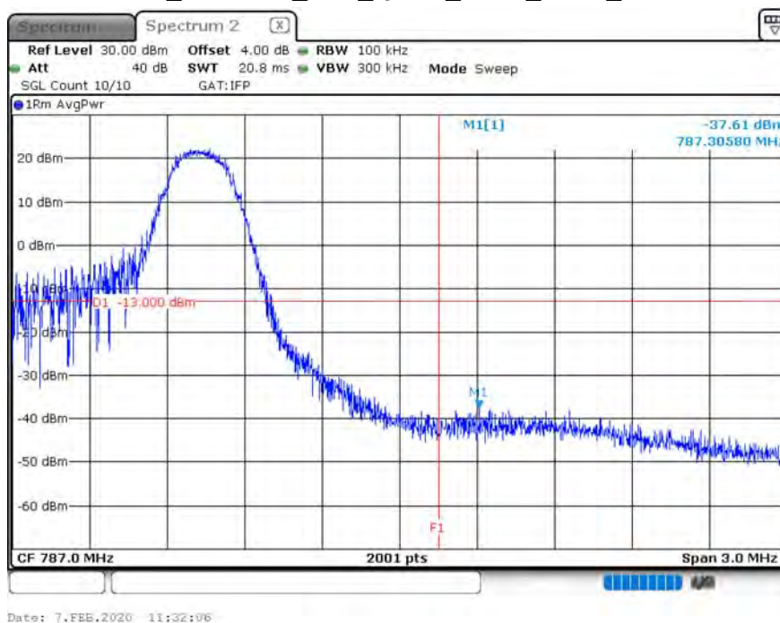
B13_CH23230_10M_QPSK_1RB5_HIGH_150k
