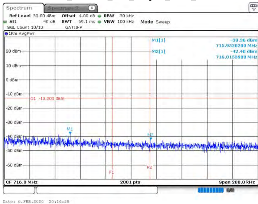
B12_CH23130_10M_16-QAM_1RB5_150k
