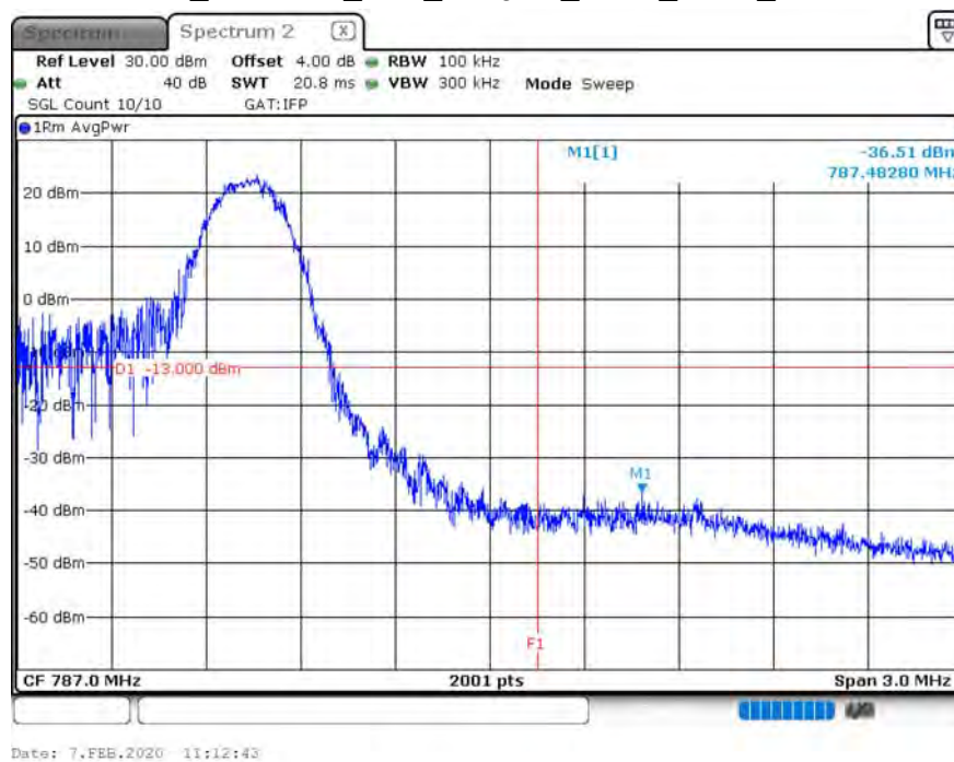
B13_CH23230_10M_16-QAM_1RB5_HIGH_150k
