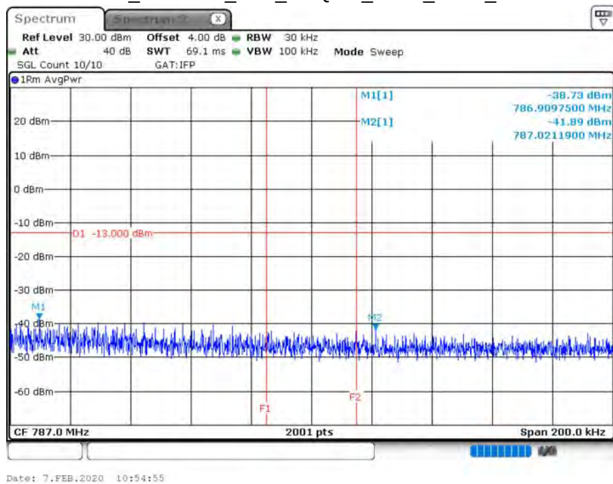
B13_CH23230_10M_16-QAM_1RB5_HIGH_150k
