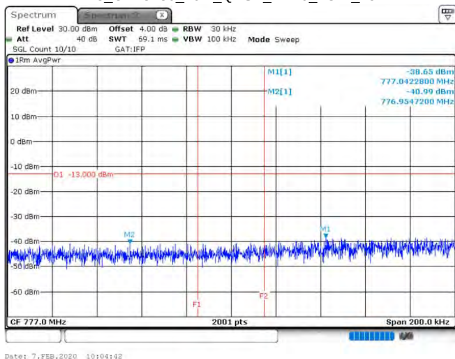
B13_CH23230_10M_QPSK_1RB0_LOW_150k
