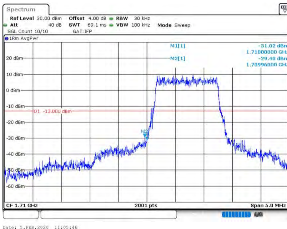
B66_CH131979_1.4M_QPSK_6RB0
