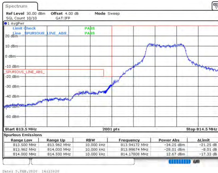
B26_CH26697_1.4M_QPSK_6RB0 (Part 90)
