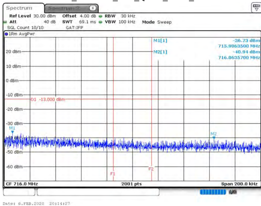
B12_CH23130_10M_QPSK_1RB5_150k
