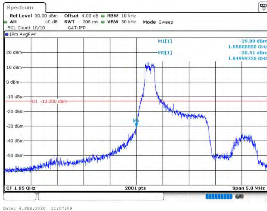
B25_CH26047_1.4M_QPSK_6RB0
