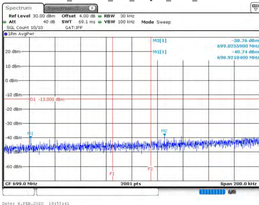
B12_CH23060_10M_16-QAM_1RB0_15k
