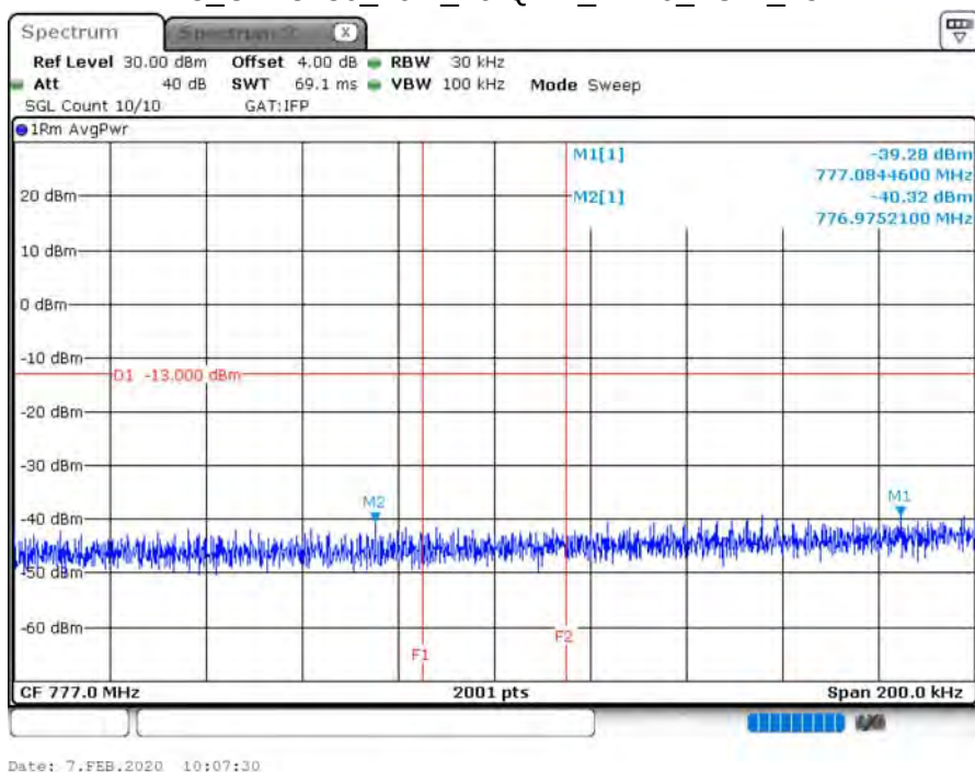
B13_CH23230_10M_16-QAM_1RB0_LOW_150k
