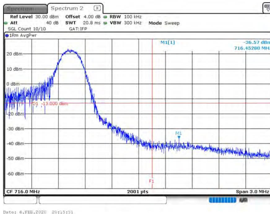
B12_CH23130_10M_16-QAM_1RB5_150k
