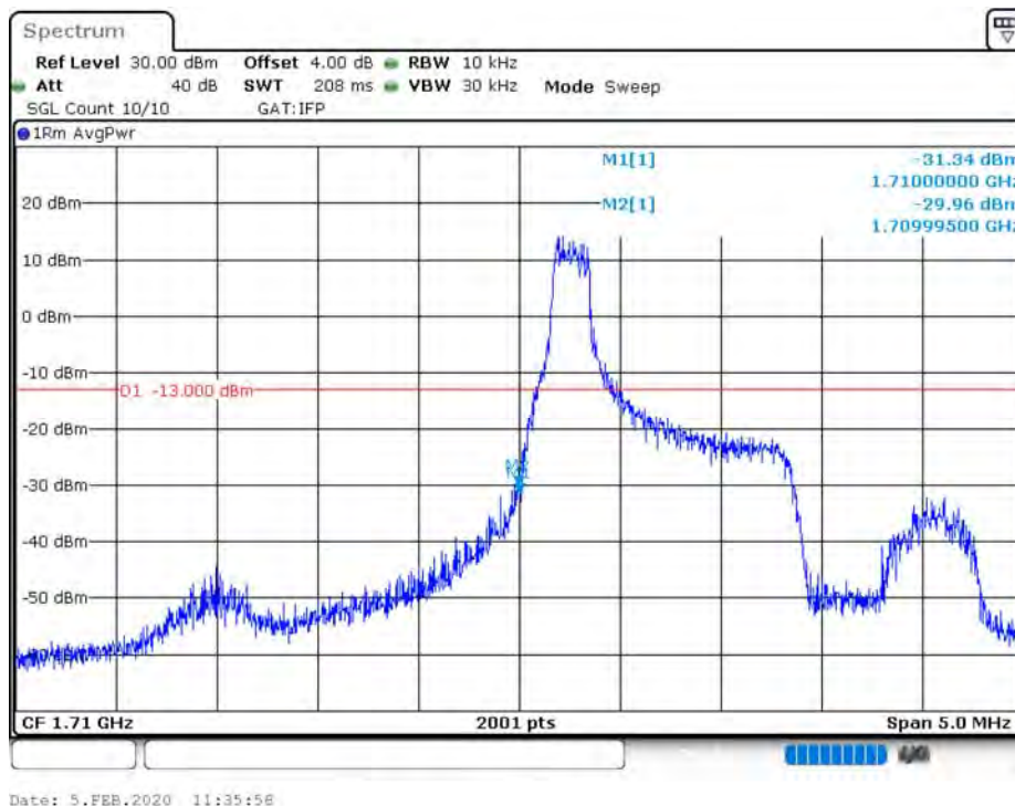
B66_CH131979_1.4M_QPSK_6RB0
