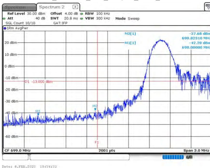
B12_CH23060_10M_16-QAM_1RB0_150k
