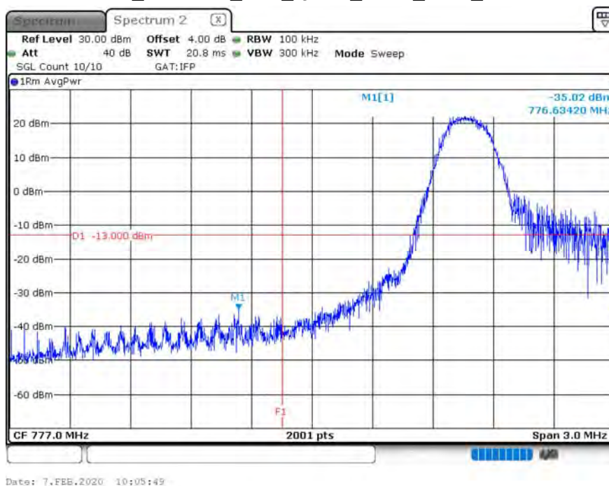
B13_CH23230_10M_QPSK_1RB0_LOW_150k
