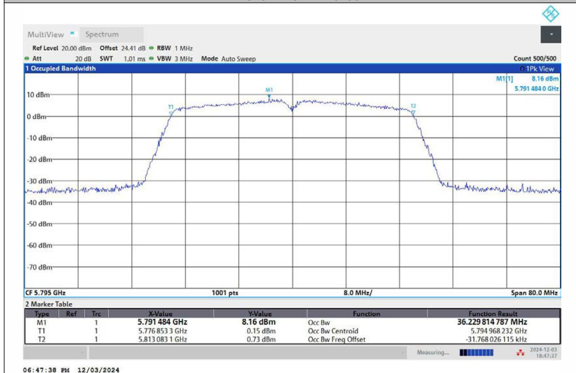
11AC40MIMO-Ant2-5795
