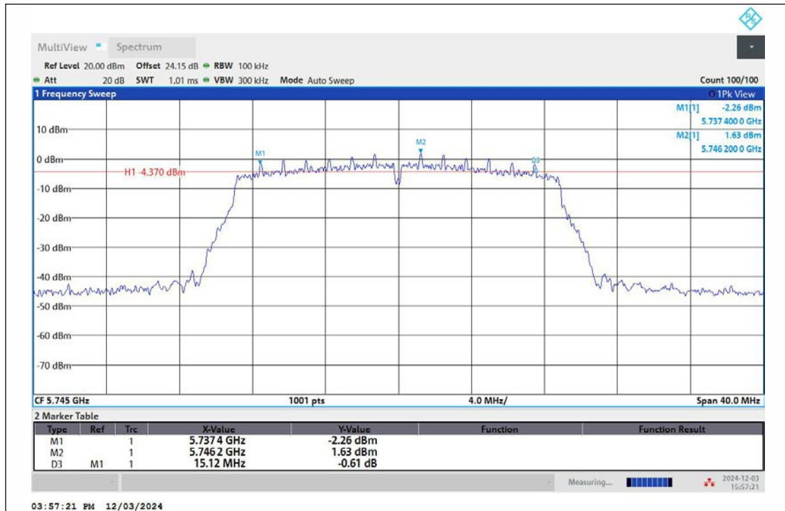
11N20MIMO-Ant1-5745-PASS
