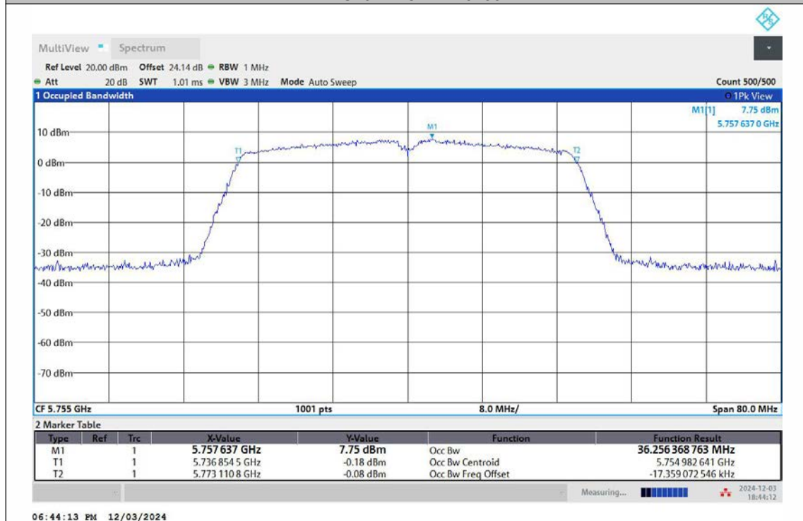
11AC40MIMO-Ant2-5755
