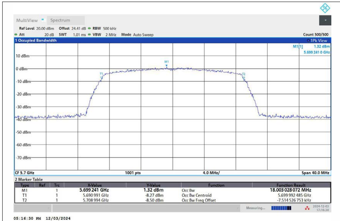
11AC20MIMO-Ant1-5700
