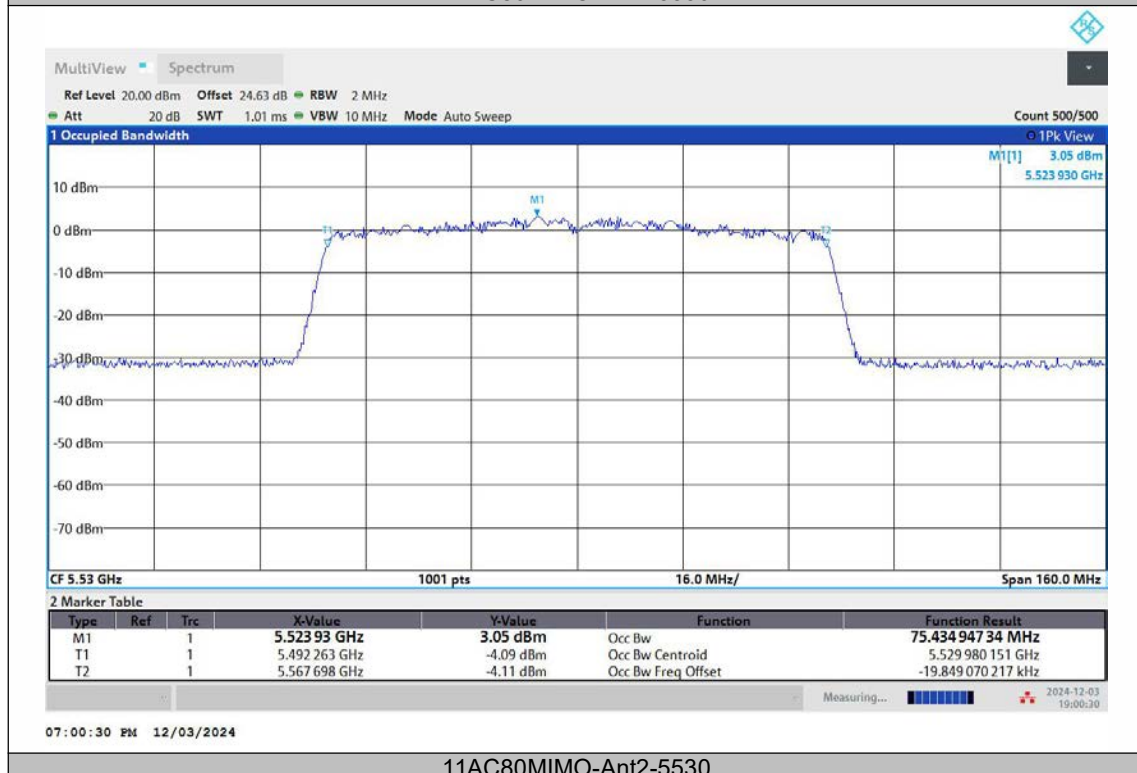
11AC80MIMO-Ant2-5530
