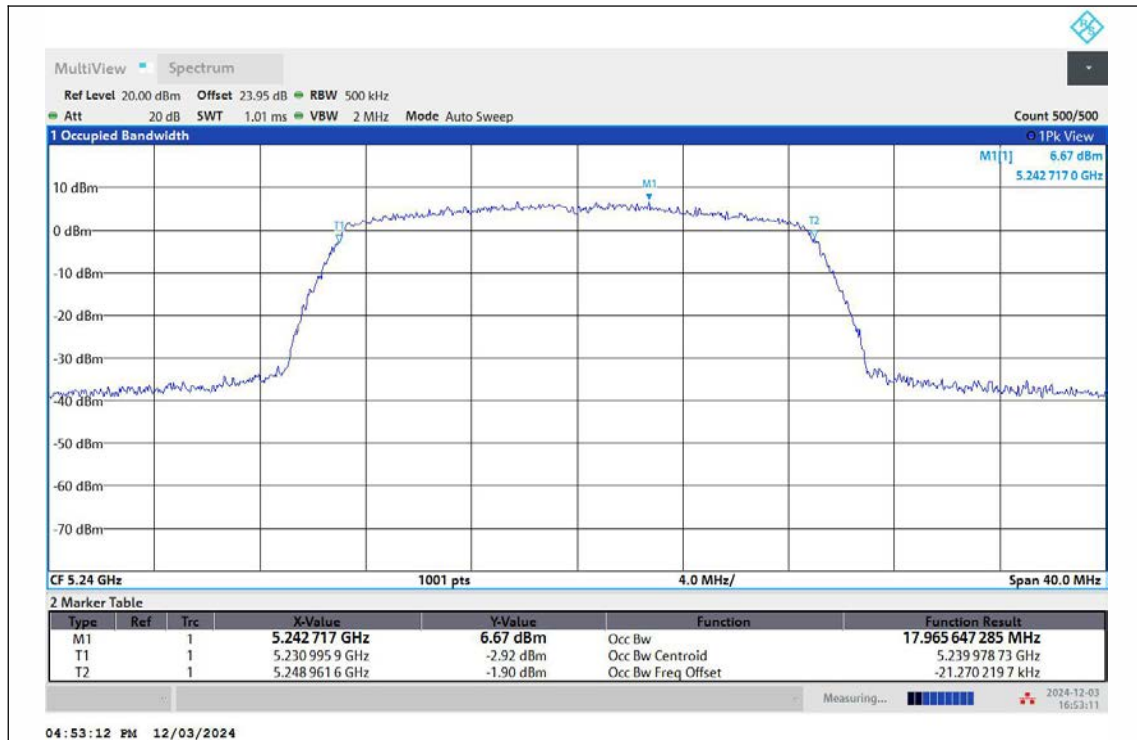
11AC20MIMO-Ant1-5240
