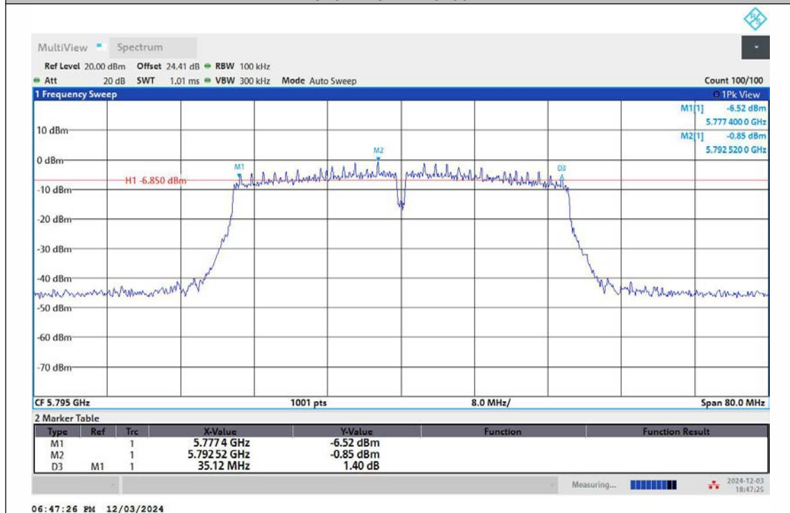
11AC40MIMO-Ant2-5795-PASS
