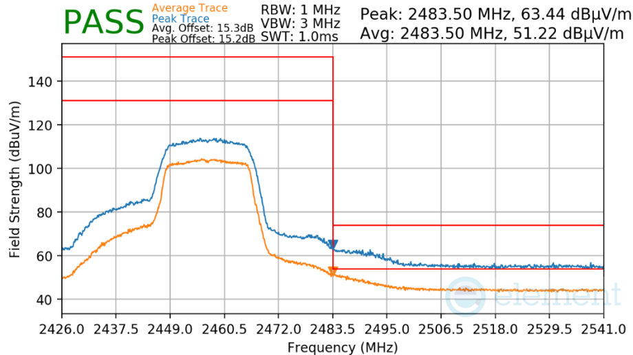
Plot 7-580 Radiated Restricted Upper Band Edge Measurement Antenna WF7
