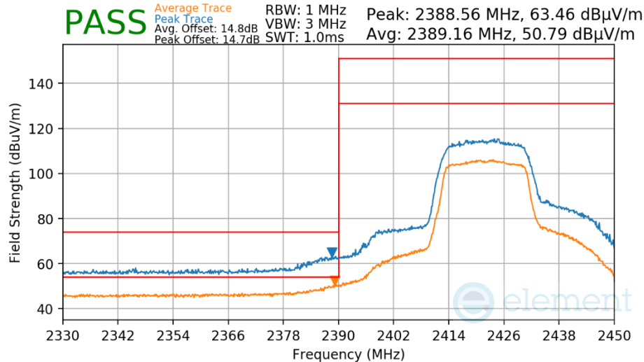
Plot 7-556 Radiated Restricted Lower Band Edge Measurement Antenna WF7
