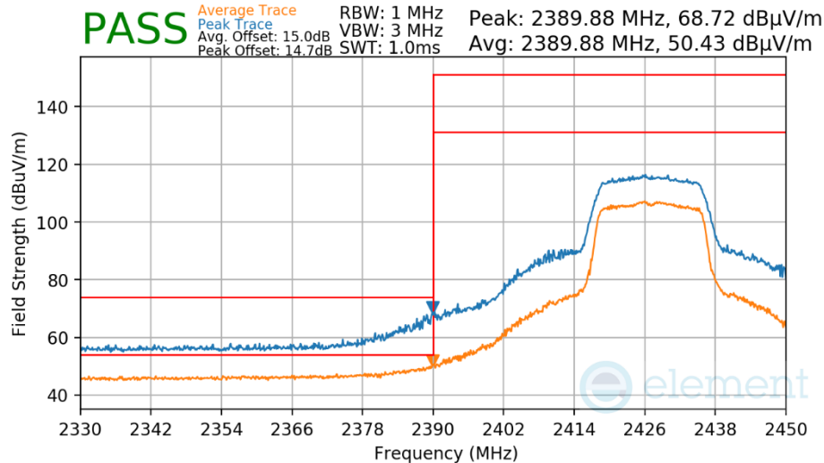
Plot 7-560 Radiated Restricted Lower Band Edge Measurement Antenna WF7
