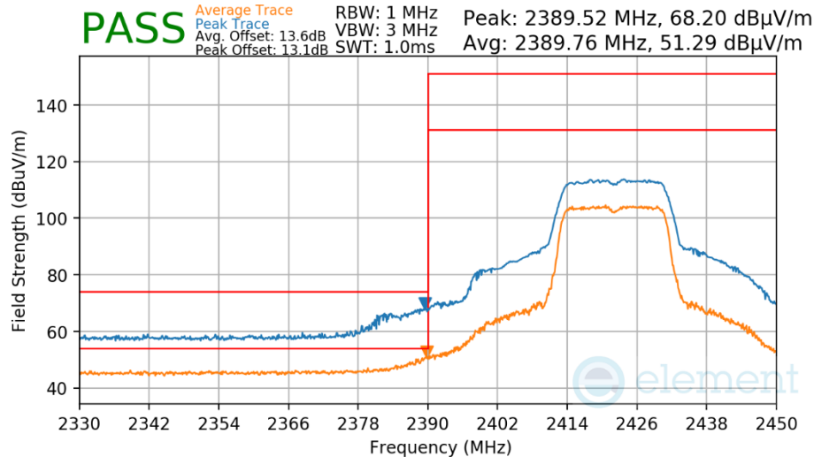
Plot 7-558 Radiated Restricted Lower Band Edge Measurement Antenna WF7
