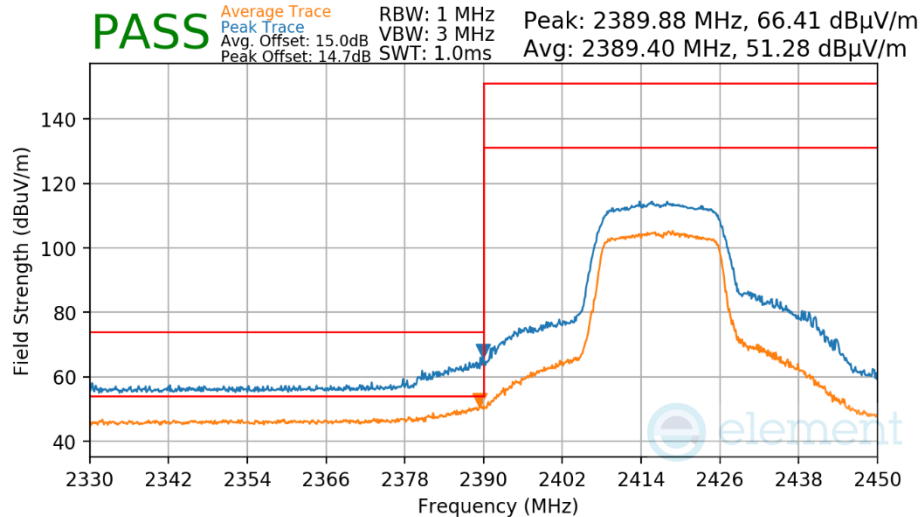
Plot 7-554 Radiated Restricted Lower Band Edge Measurement Antenna WF7
