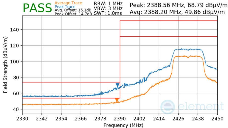
Plot 7-564 Radiated Restricted Lower Band Edge Measurement Antenna WF7
