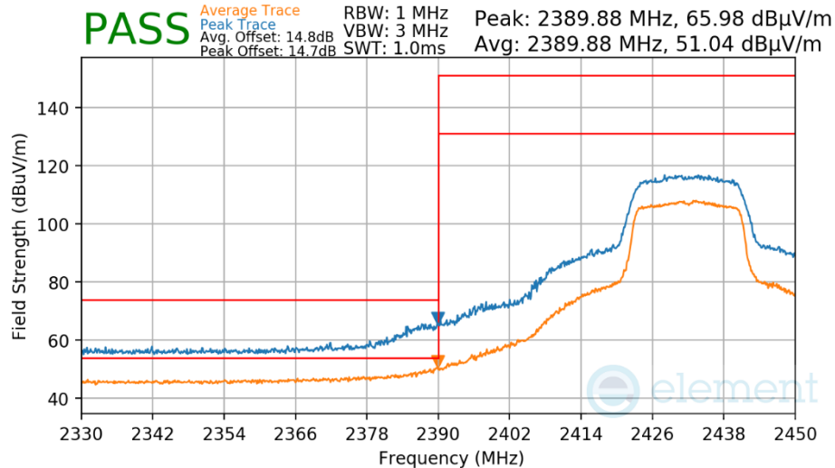
Plot 7-562 Radiated Restricted Lower Band Edge Measurement Antenna WF7
