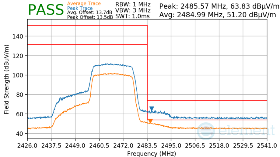
Plot 7-543 Radiated Restricted Upper Band Edge Measurement Antenna WF8
