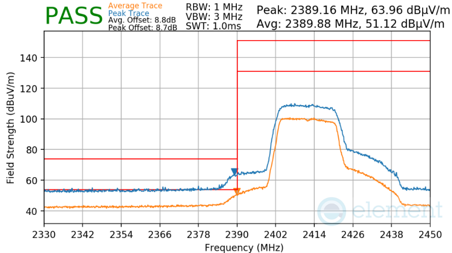
Plot 7-550 Radiated Restricted Lower Band Edge Measurement Antenna WF7
