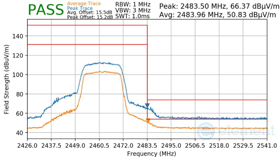
Plot 7-584 Radiated Restricted Upper Band Edge Measurement Antenna WF7
