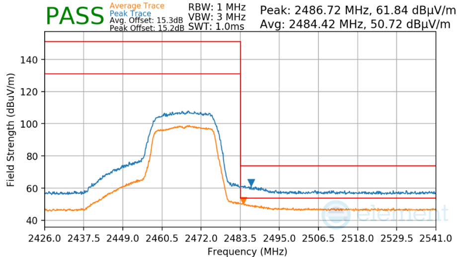
Plot 7-586 Radiated Restricted Upper Band Edge Measurement Antenna WF7
