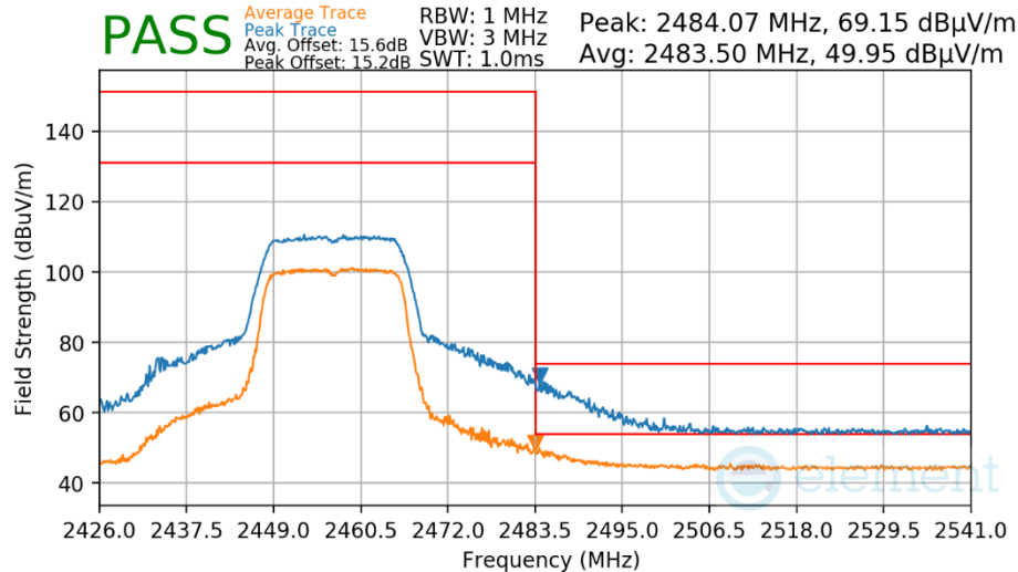
Plot 7-582 Radiated Restricted Upper Band Edge Measurement Antenna WF7
