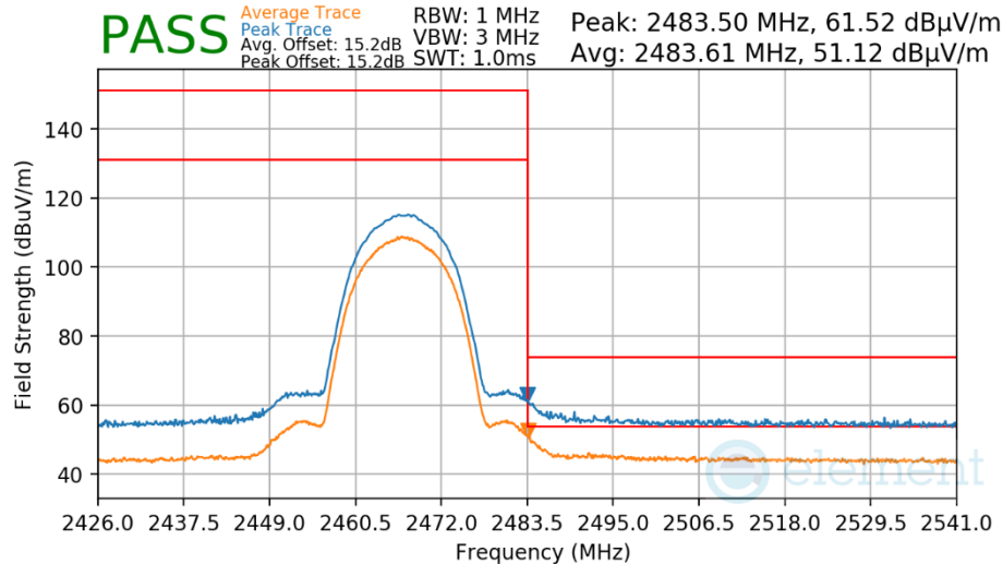
Plot 7-548 Radiated Restricted Upper Band Edge Measurement Antenna WF7
