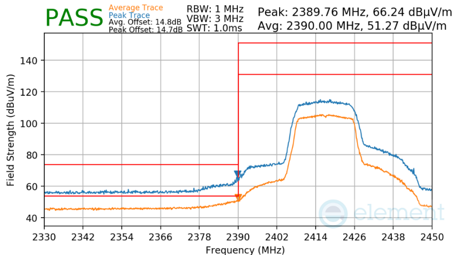
Plot 7-553 Radiated Restricted Lower Band Edge Measurement Antenna WF7
