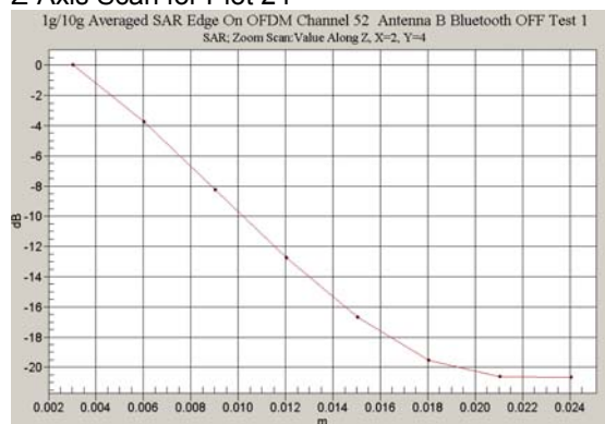
Z-Axis Scan for Plot 24
