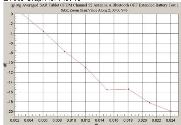
Z-Axis Graph for Plot 19
