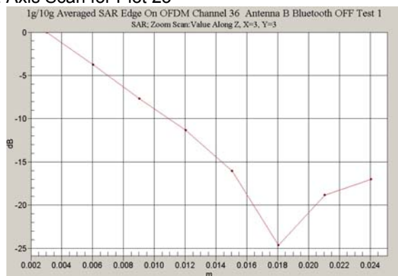
Z-Axis Scan for Plot 23
