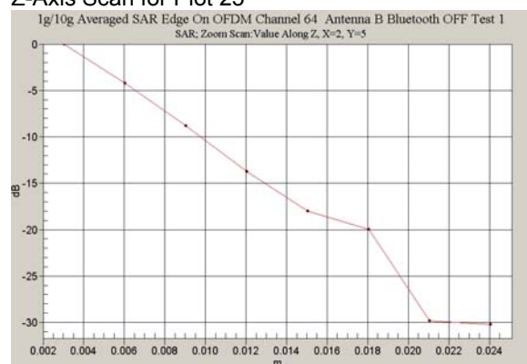
Z-Axis Scan for Plot 25
