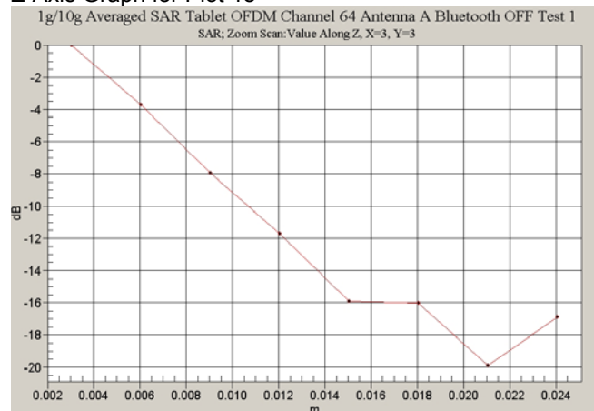
Z-Axis Graph for Plot 18
