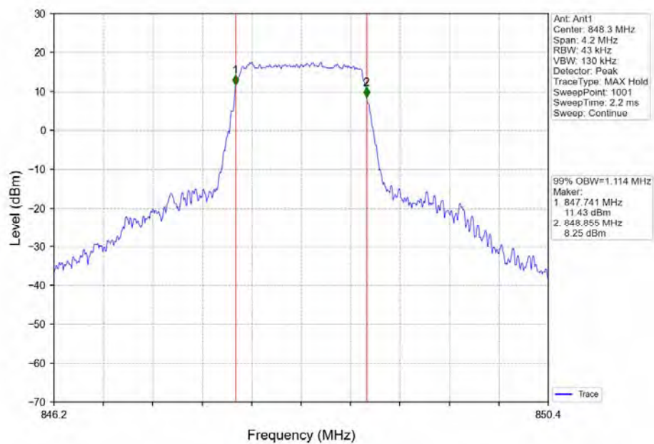
Band5_1.4MHz_16QAM_HCH_848.3MHz_RB_6_0_NTNV
