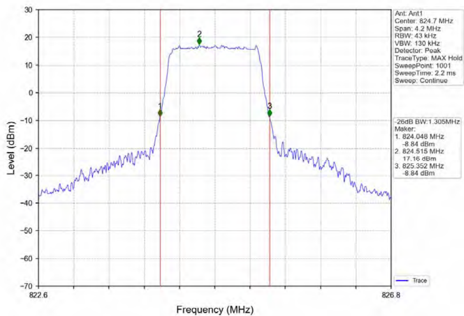
Band5_1.4MHz_16QAM_LCH_824.7MHz_RB_6_0_NTNV
