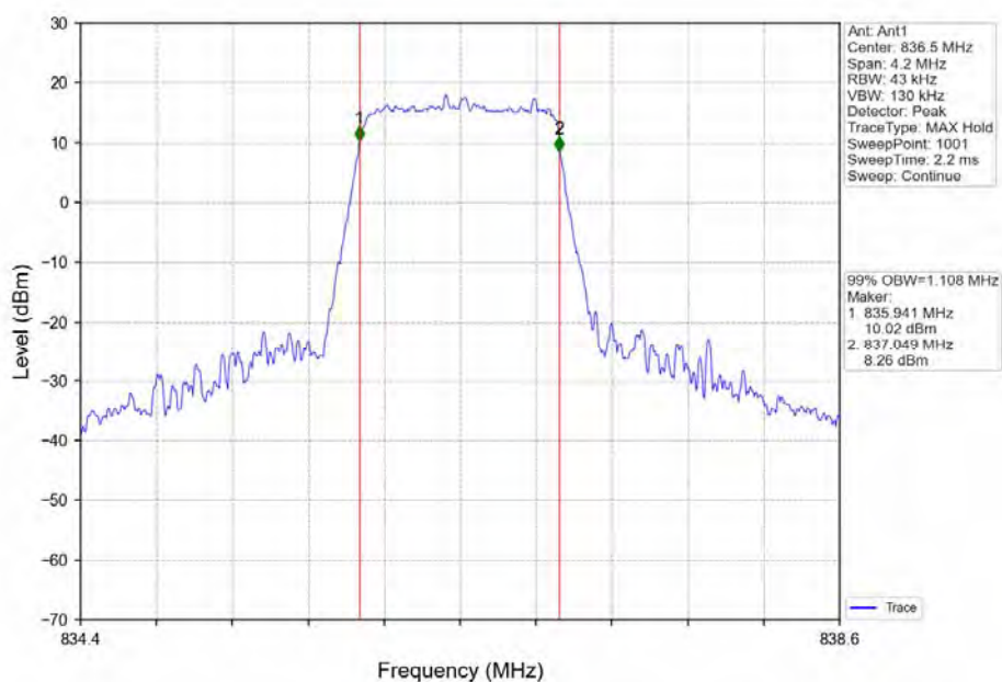
Band5_1.4MHz_64QAM_MCH_836.5MHz_RB_6_0_NTNV
