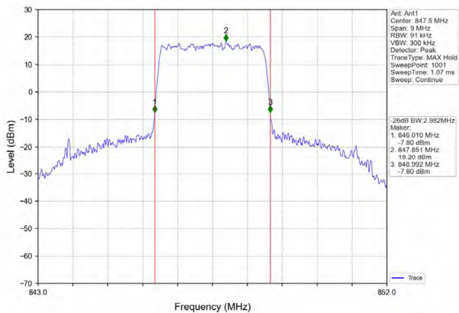
Band5_3MHz_QPSK_HCH_847.5MHz_RB_15_0_NTNV
