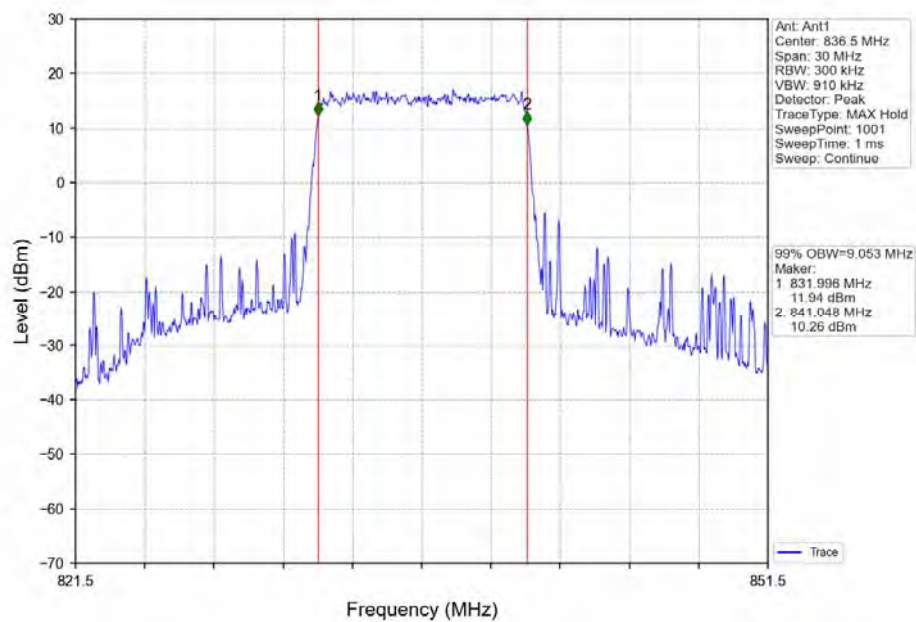
Band5_10MHz_16QAM_MCH_836.5MHz_RB_50_0_NTNV
