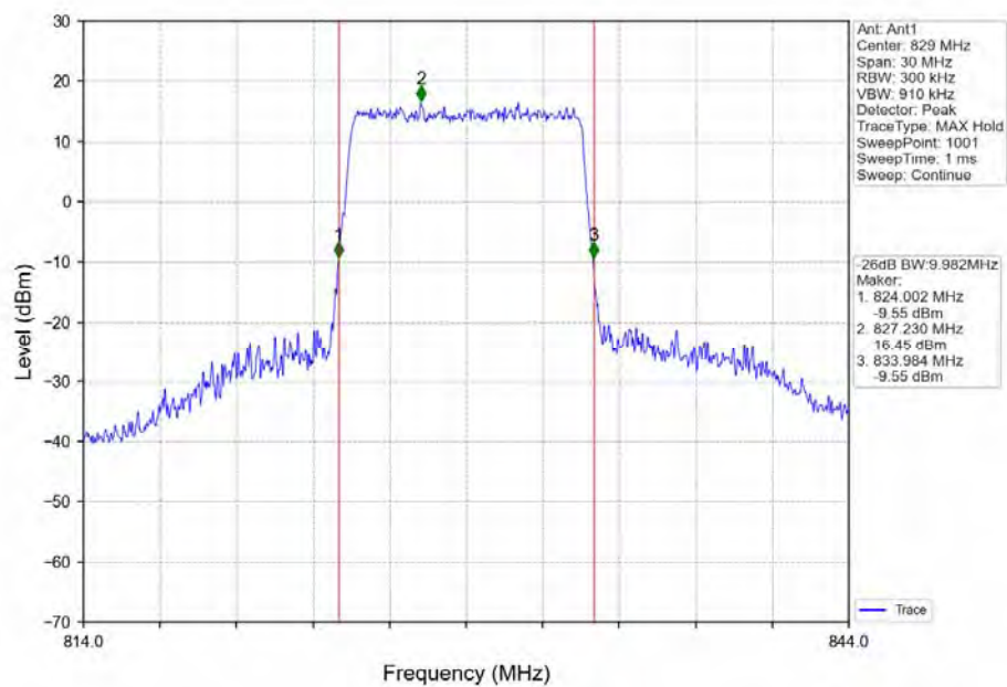
Band5_10MHz_64QAM_LCH_829MHz_RB_50_0_NTNV
