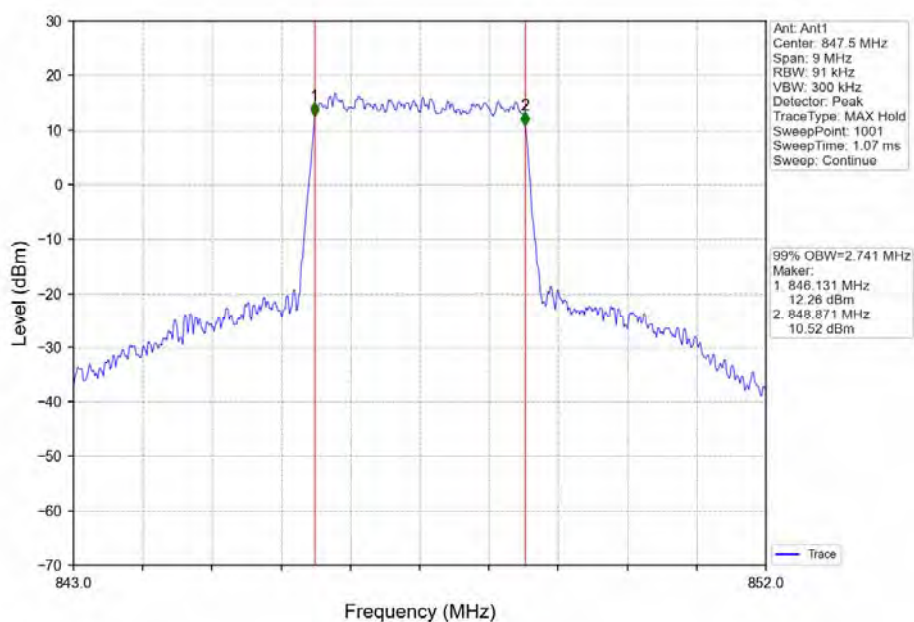
Band5_3MHz_64QAM_HCH_847.5MHz_RB_15_0_NTNV
