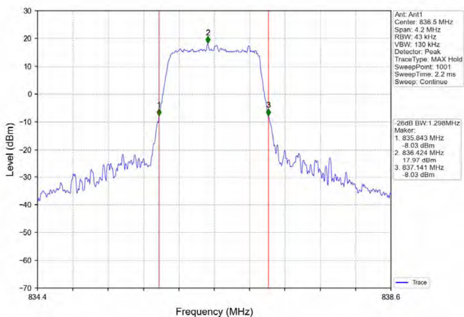
Band5_1.4MHz_64QAM_MCH_836.5MHz_RB_6_0_NTNV
