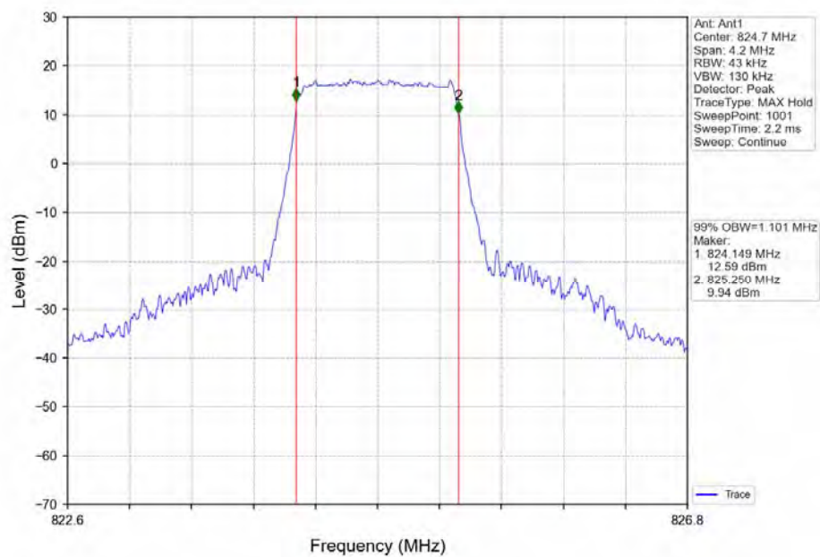
Band5_1.4MHz_16QAM_LCH_824.7MHz_RB_6_0_NTNV
