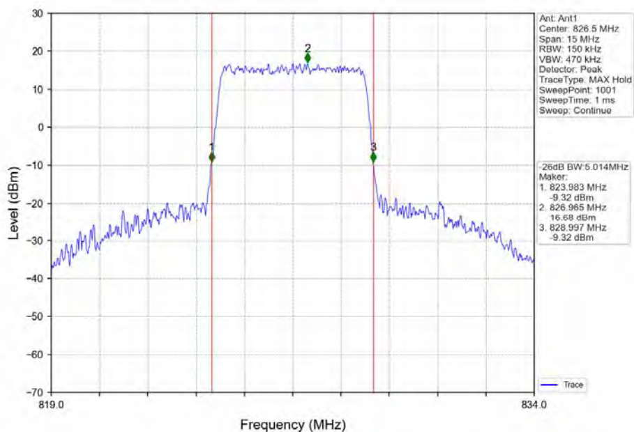
Band5_5MHz_16QAM_LCH_826.5MHz_RB_25_0_NTNV
