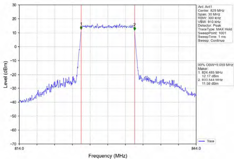
Band5_10MHz_64QAM_LCH_829MHz_RB_50_0_NTNV
