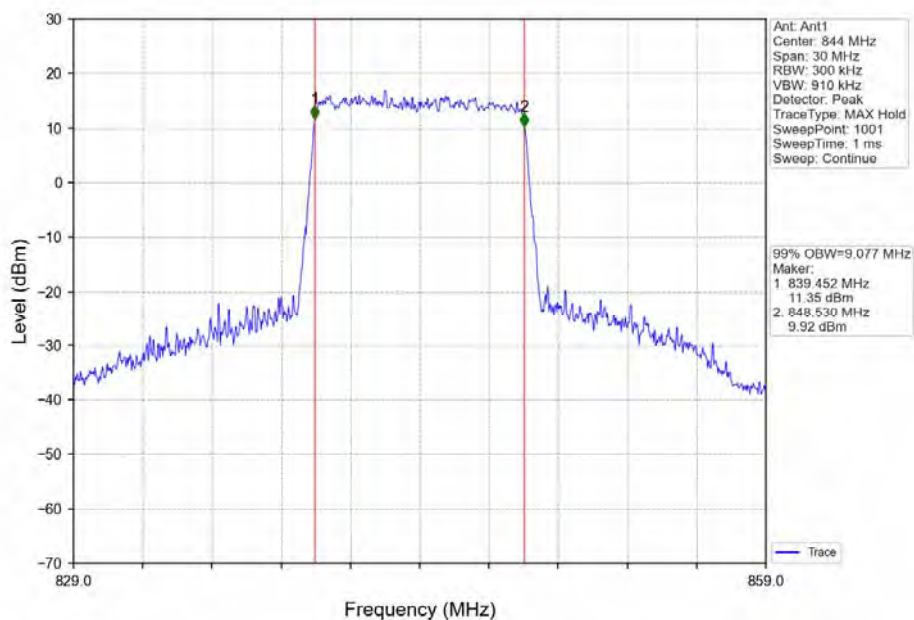
Band5_10MHz_64QAM_HCH_844MHz_RB_50_0_NTNV
