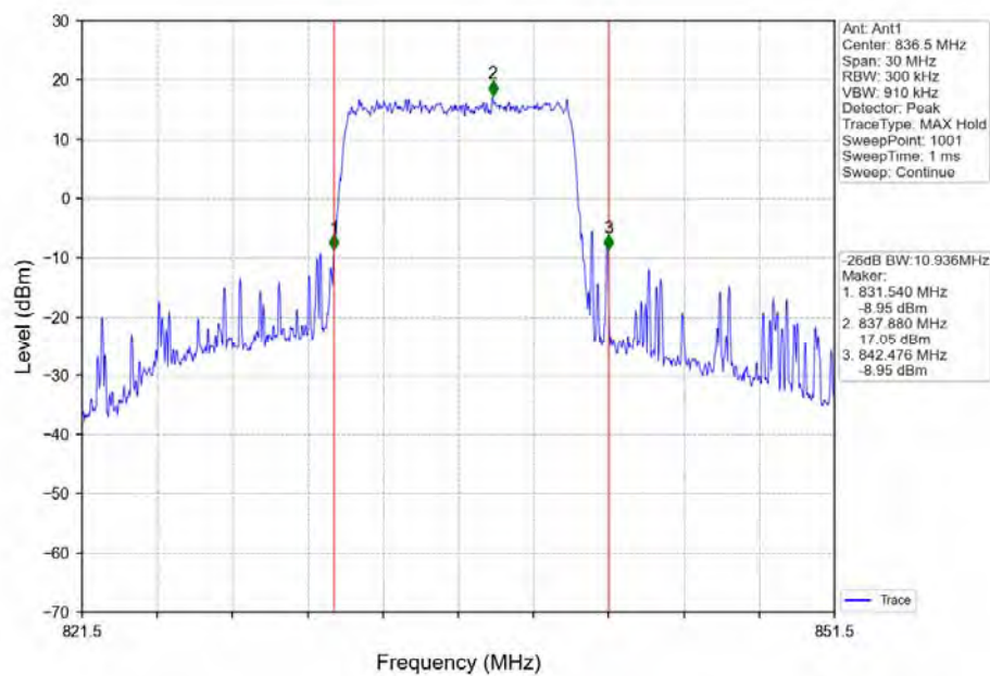
Band5_10MHz_16QAM_MCH_836.5MHz_RB_50_0_NTNV
