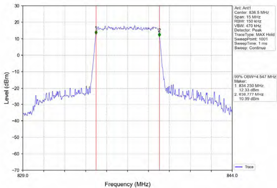
Band5_5MHz_QPSK_MCH_836.5MHz_RB_25_0_NTNV
