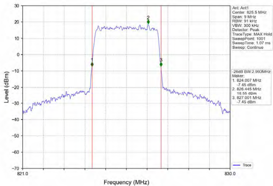
Band5_3MHz_QPSK_LCH_825.5MHz_RB_15_0_NTNV
