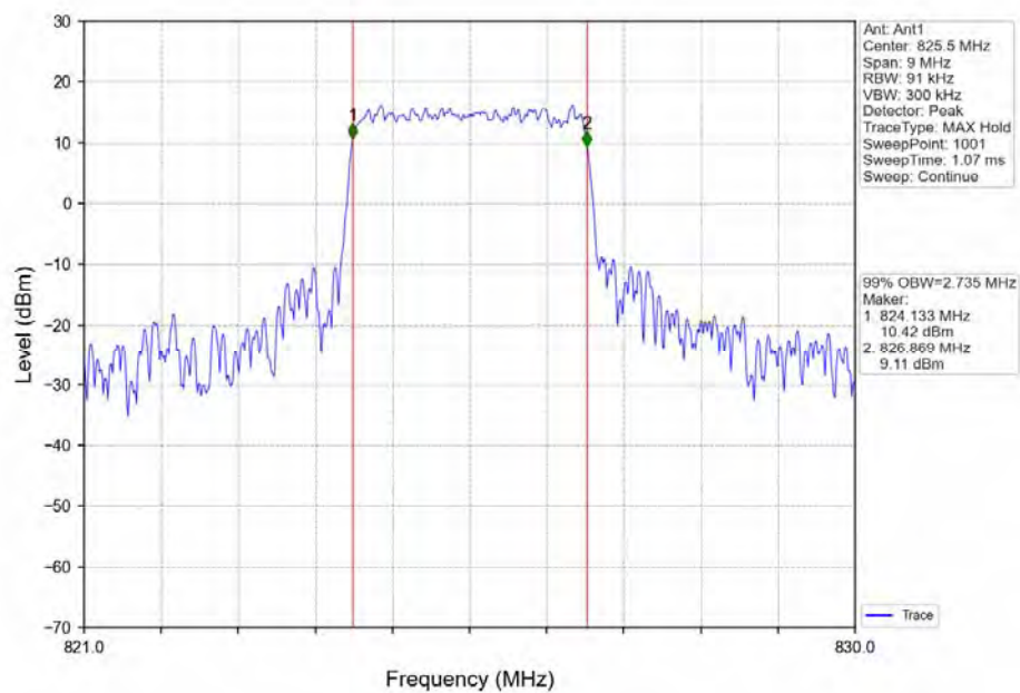
Band5_3MHz_64QAM_LCH_825.5MHz_RB_15_0_NTNV
