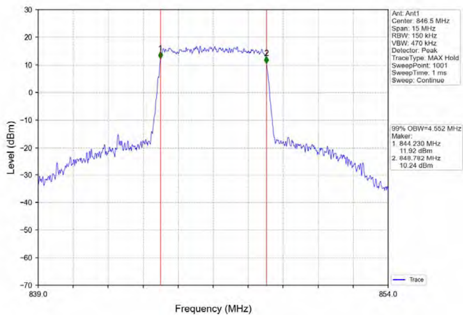
Band5_5MHz_16QAM_HCH_846.5MHz_RB_25_0_NTNV
