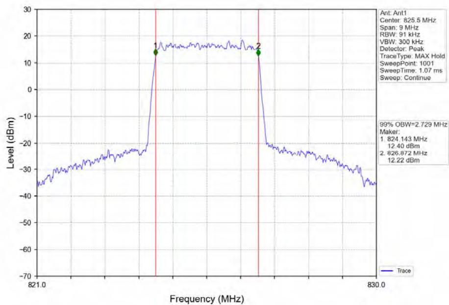
Band5_3MHz_QPSK_LCH_825.5MHz_RB_15_0_NTNV
