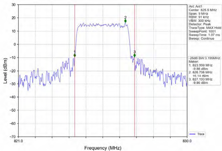
Band5_3MHz_64QAM_LCH_825.5MHz_RB_15_0_NTNV
