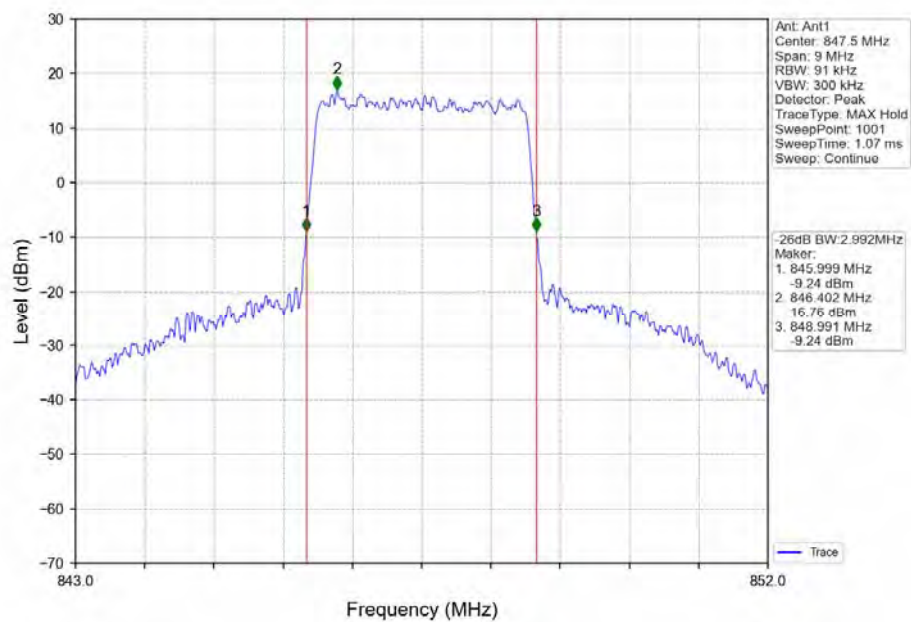
Band5_3MHz_64QAM_HCH_847.5MHz_RB_15_0_NTNV
