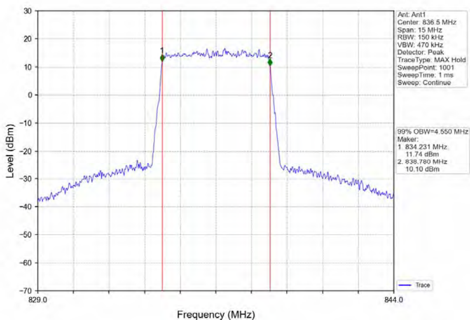
Band5_5MHz_64QAM_MCH_836.5MHz_RB_25_0_NTNV
