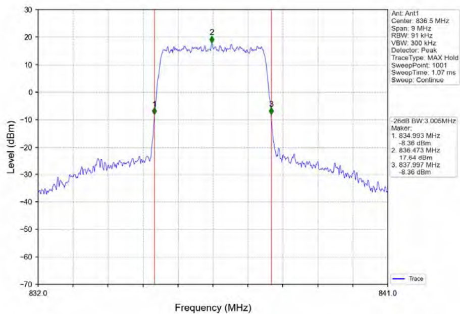
Band5_3MHz_16QAM_MCH_836.5MHz_RB_15_0_NTNV
