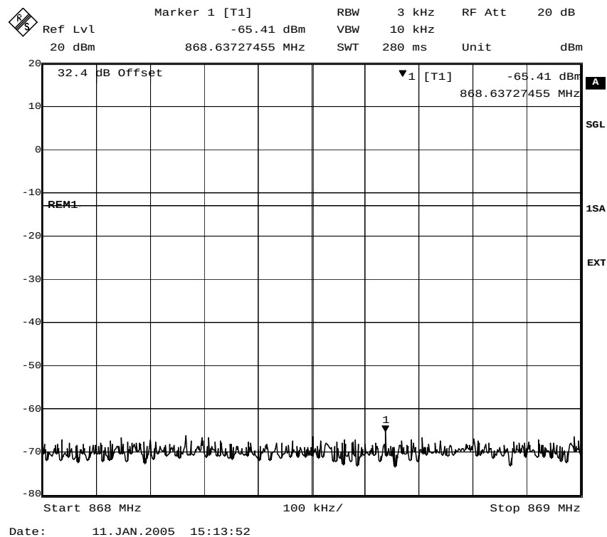
Fig. 47 – Spurious emissions in the frequency range 868 MHz – 869 MHz (8PSK modulation).
