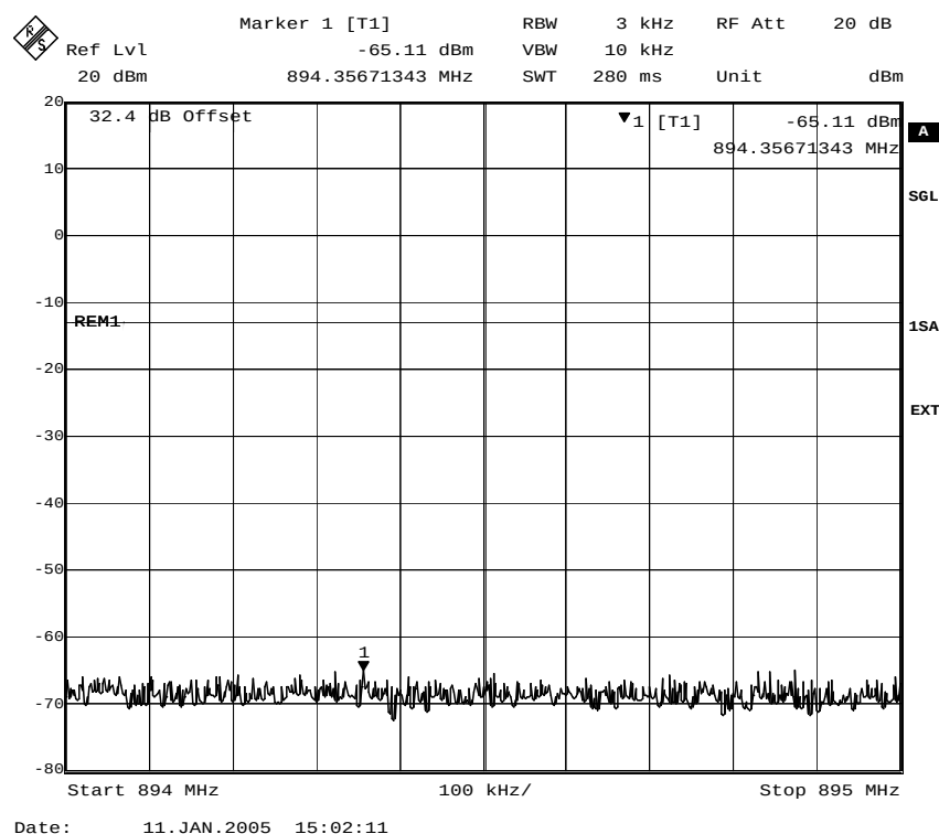
Fig. 38 – Spurious emissions in the frequency range 894 MHz – 895 MHz (GMSK modulation).
