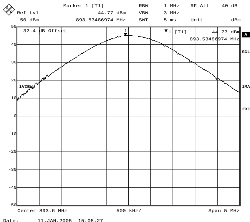
Fig. 11 – RF power at the antenna connector (8PSK modulation).
