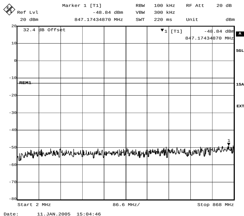
Fig. 35 – Spurious emissions in the frequency range 2 MHz – 868 MHz (8PSK modulation).
