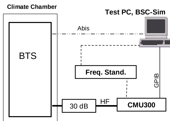
Fig. 2 – Measurement Test Configuration
