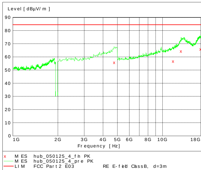
Fig. 61 – Radiated Emission 1 GHz – 18 GHz, 8PSK modulation.
