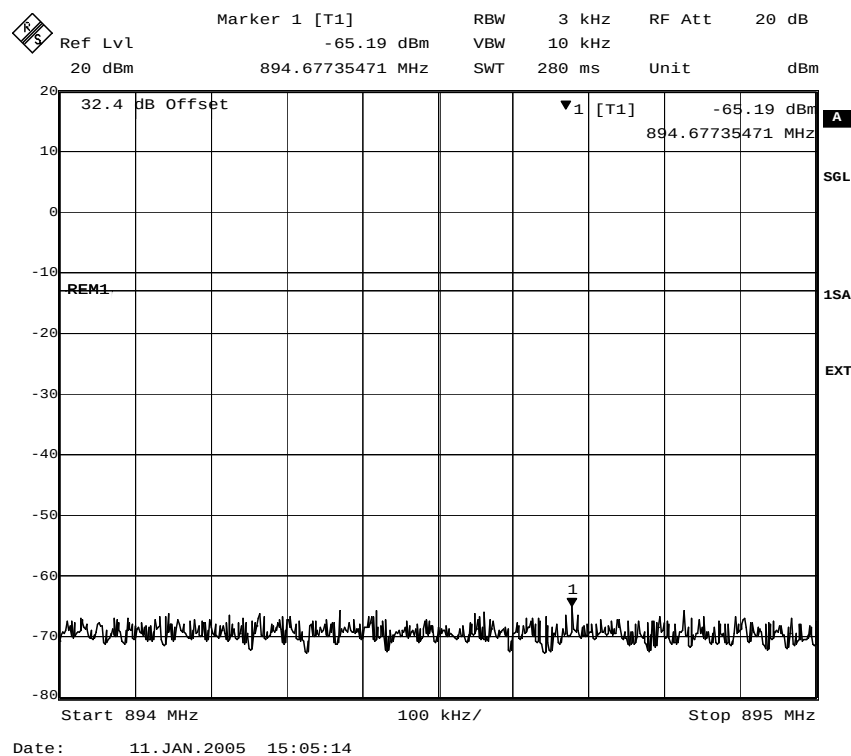
Fig. 39 – Spurious emissions in the frequency range 894 MHz – 895 MHz (8PSK modulation).
