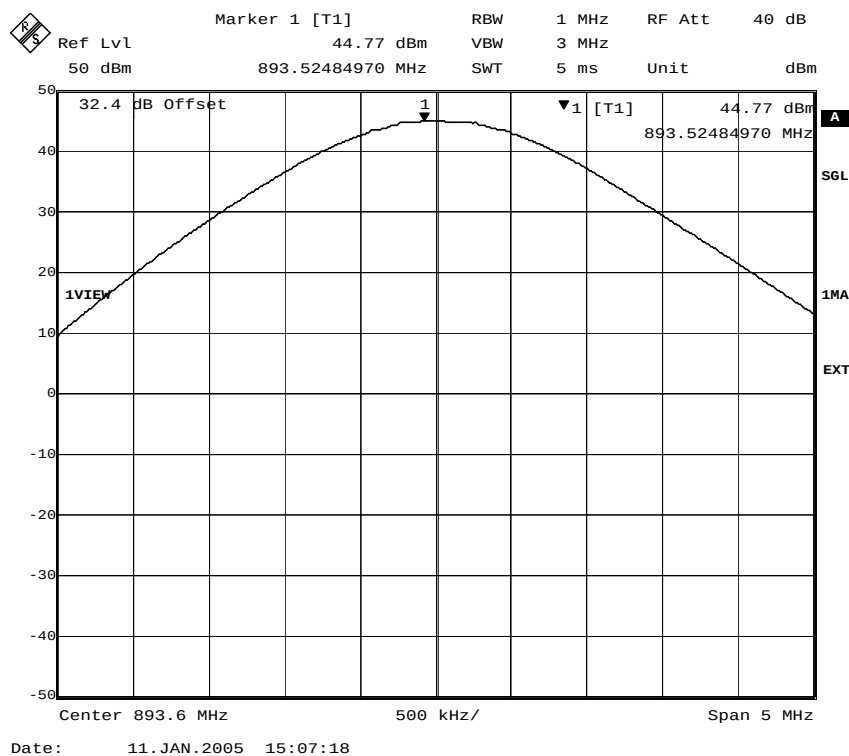
Fig. 10 – RF power at the antenna connector (GMSK modulation).
