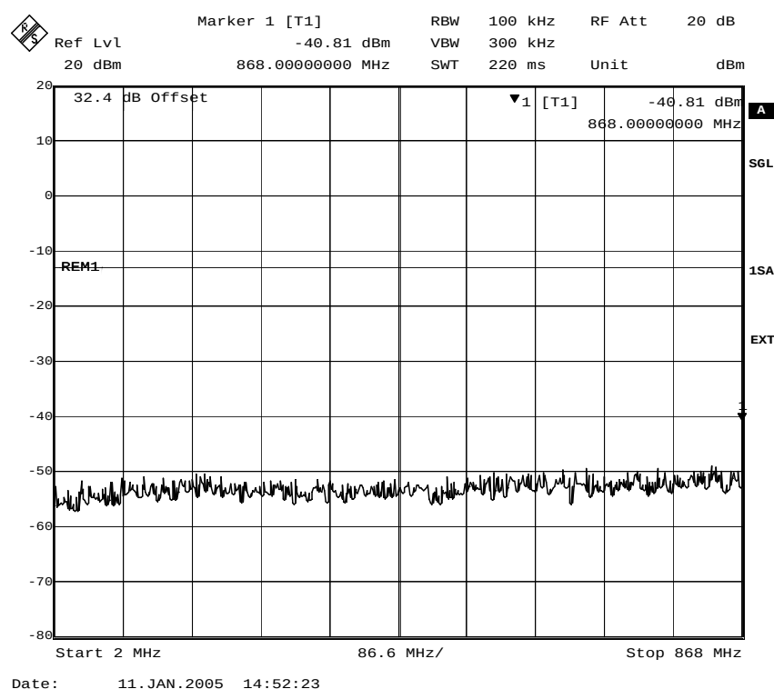
Fig. 24 – Spurious emissions in the frequency range 2 MHz – 868 MHz (GMSK modulation).
