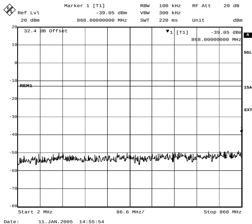
Fig. 25 – Spurious emissions in the frequency range 2 MHz – 868 MHz (8PSK modulation).
