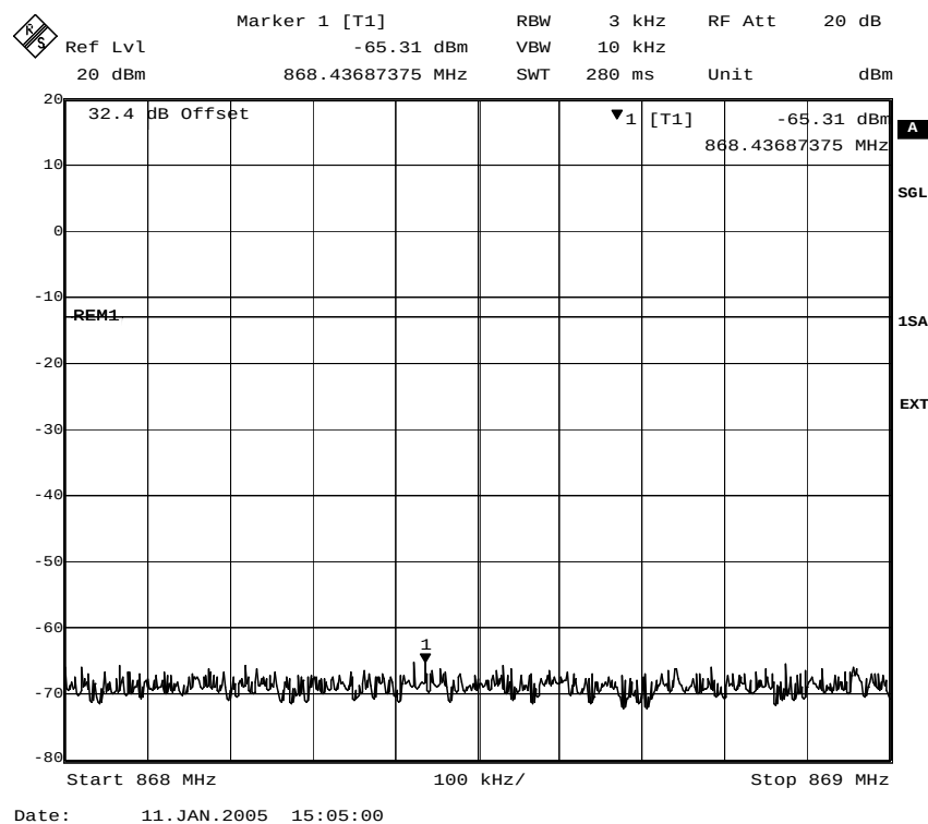
Fig. 37 – Spurious emissions in the frequency range 868 MHz – 869 MHz (8PSK modulation).
