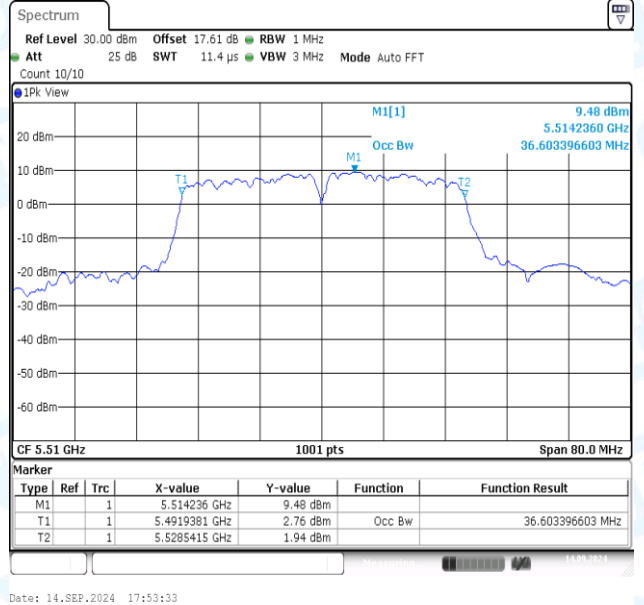
11N40MIMO-Ant2-5510
