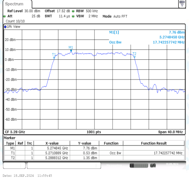
11AC20MIMO-Ant2-5280
