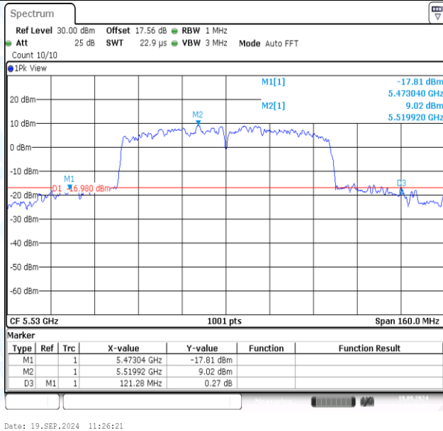
11AC80MIMO-Ant1-5530
