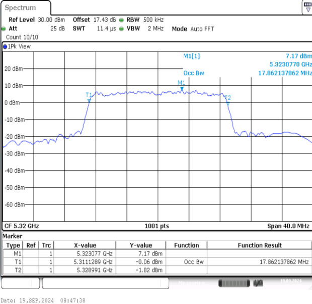
11AC20MIMO-Ant1-5320
