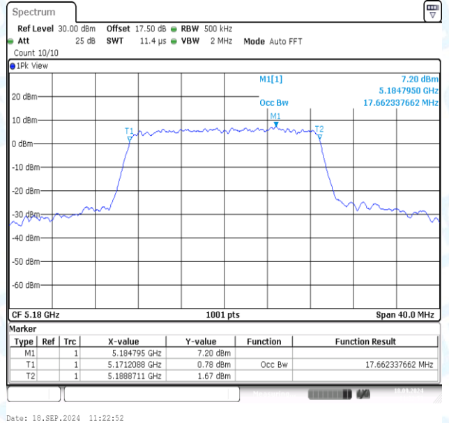
11AC20MIMO-Ant2-5180
