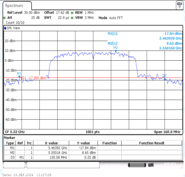
11AC80MIMO-Ant2-5530
