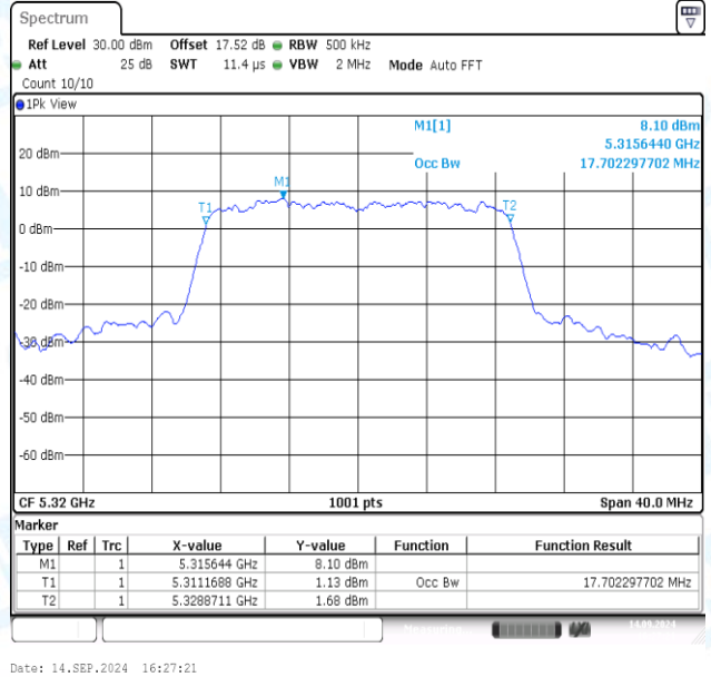
11N20MIMO-Ant2-5320
