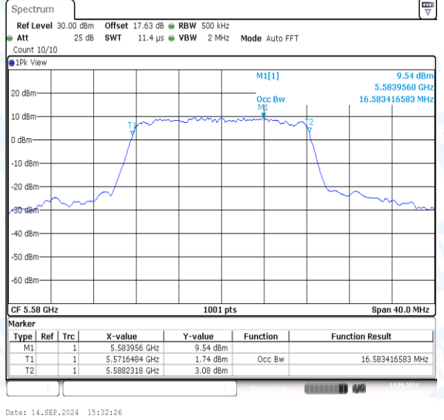
11A-Ant2-5580
