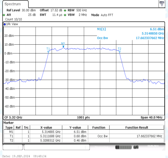
11AC20MIMO-Ant2-5320
