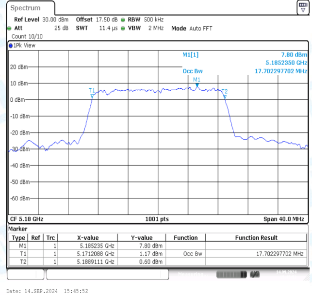
11N20MIMO-Ant2-5180
