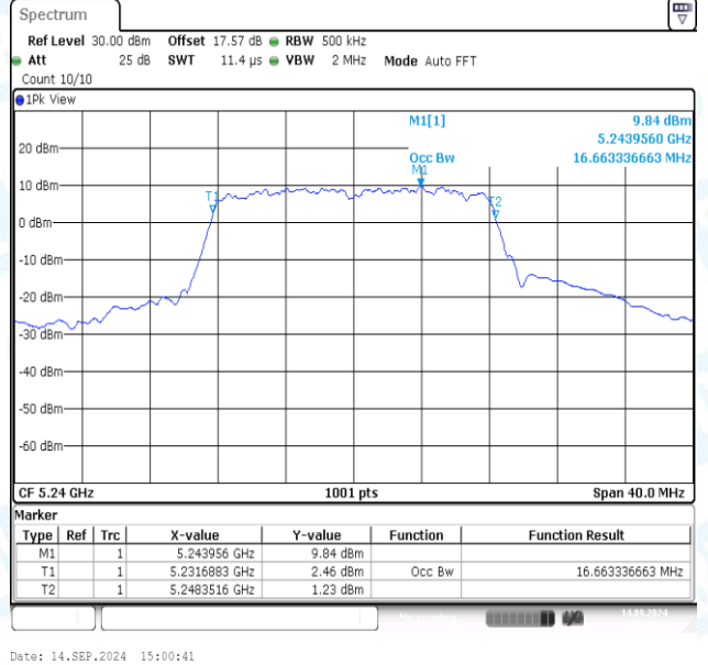
11A-Ant2-5240
