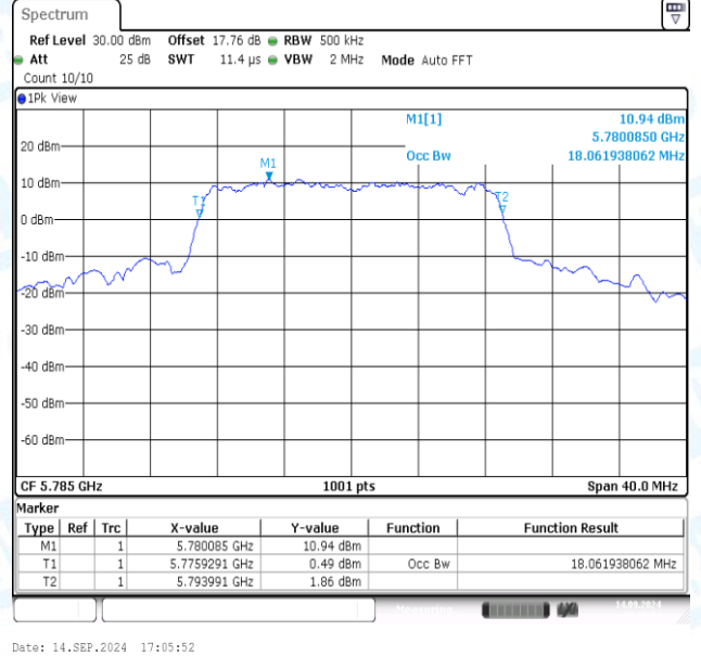
11N20MIMO-Ant2-5785
