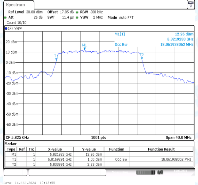
11N20MIMO-Ant2-5825
