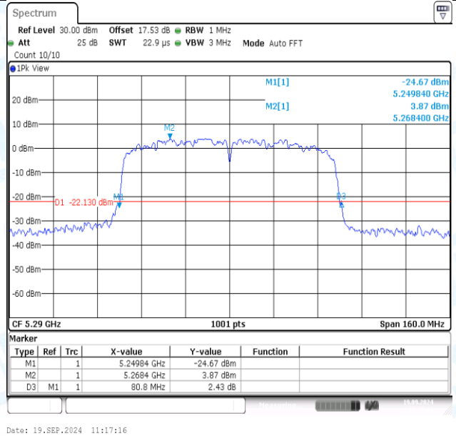
11AC80MIMO-Ant2-5290
