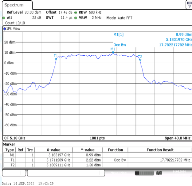
11N20MIMO-Ant1-5180
