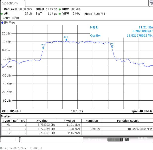
11N20MIMO-Ant1-5785
