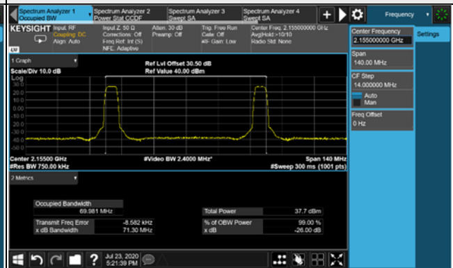
Chain 3 / 16QAM
