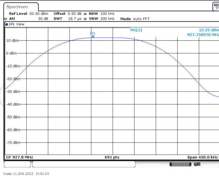
Ant1_927.8_0~Reference
