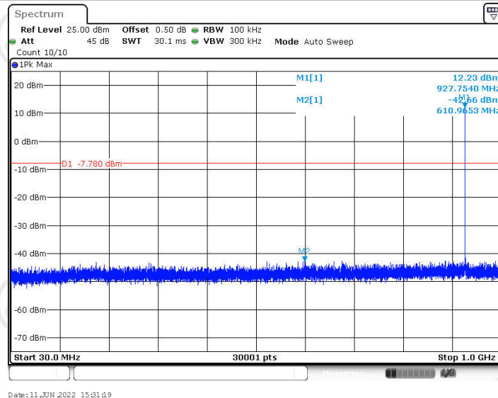
Ant1_927.8_30~1000
