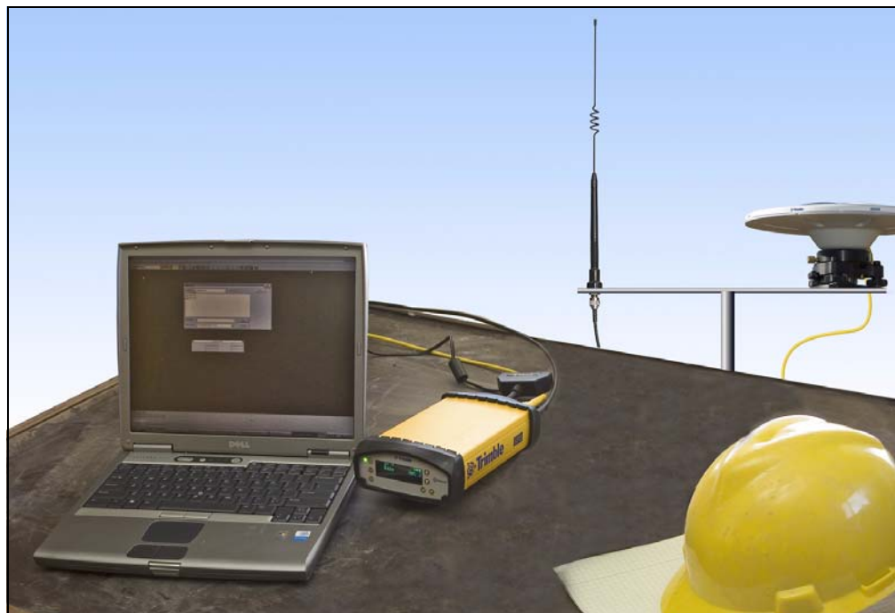
Figure 5.1 SPSx50 receiver permanent installation
