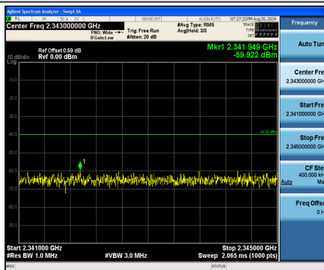
Band40-10MHz-16QAM-39200-1RB#0-Range5:2360~2365MHz
