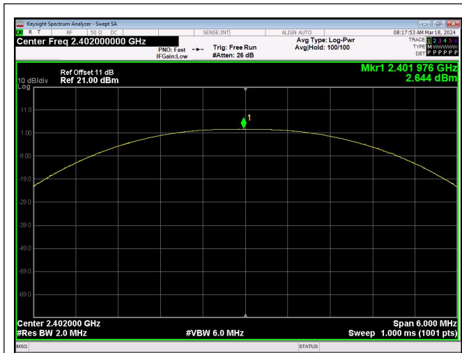
Peak Output Power 1Mbps_Channel 0
