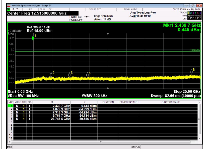
Spurious Emissions 1Mbps_Channel 19
