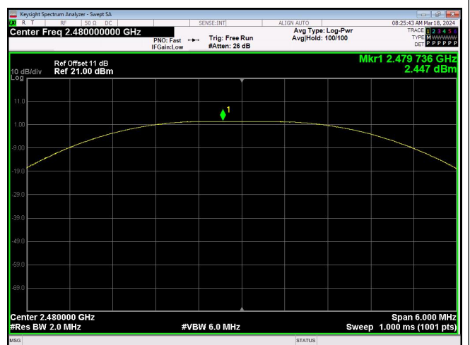
Peak Output Power 2Mbps_Channel 39
