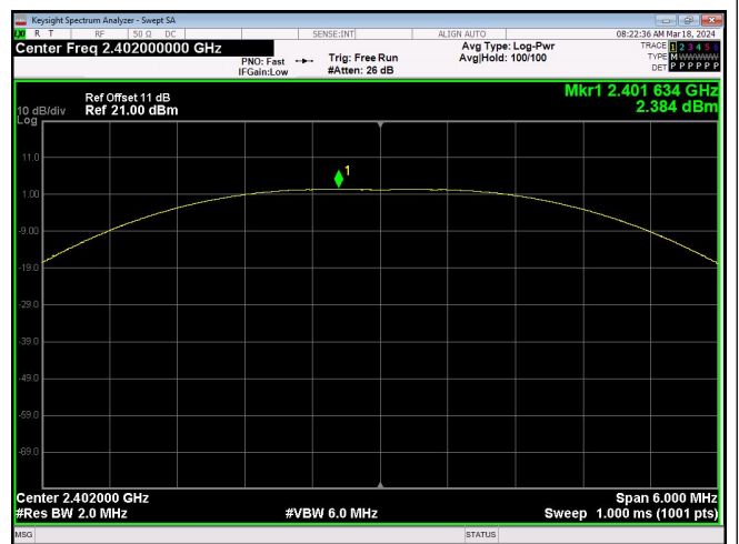
Peak Output Power 2Mbps_Channel 0
