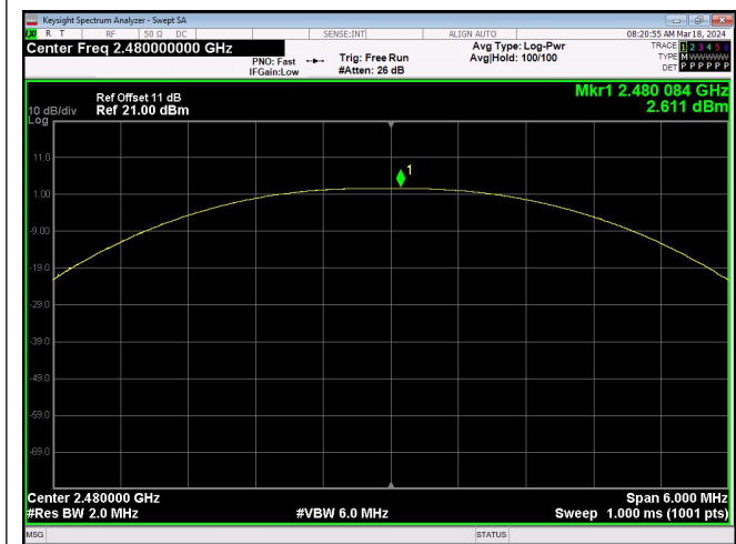
Peak Output Power 1Mbps_Channel 39
