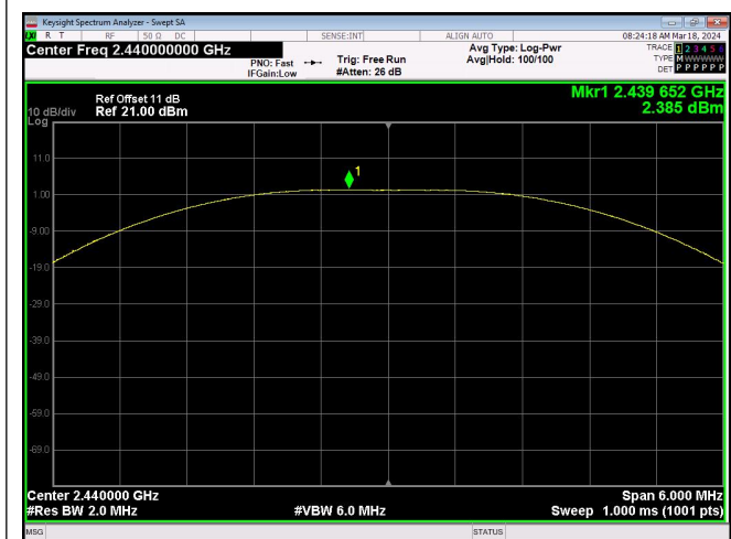
Peak Output Power 2Mbps_Channel 19
