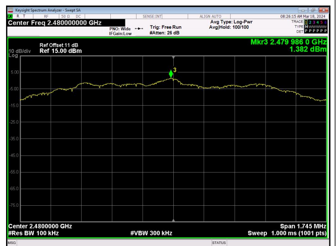
In-Band Reference 1Mbpsvel 2Mbps_Channel 39
