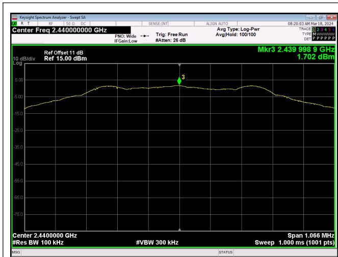
In-Band Reference 1Mbpsvel 1Mbps_Channel 19
