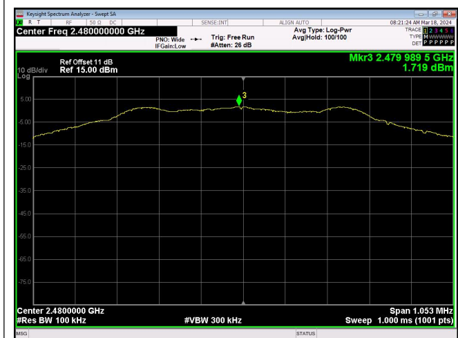
In-Band Reference 1Mbpsvel 1Mbps_Channel 39
