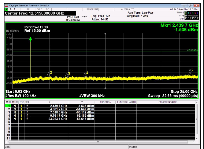
Spurious Emissions 2Mbps_Channel 19
