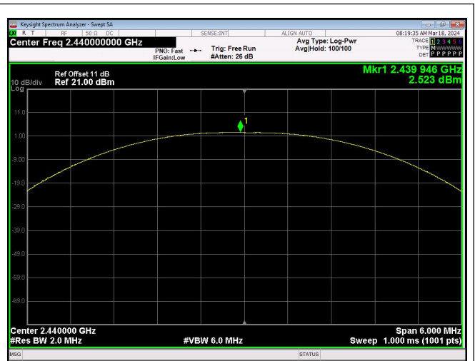
Peak Output Power 1Mbps_Channel 19
