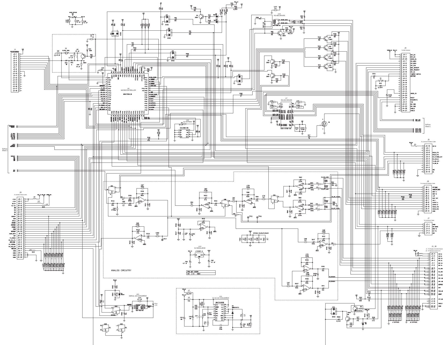
LOGIC BOARD (REV. 2) SCHEMATIC (PART 1 OF 2)
