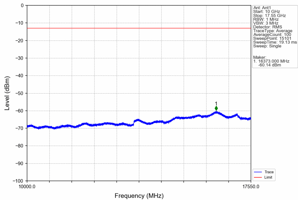
Band4_5MHz_16QAM_LCH_1712.5MHz_RB_1_0_NTNV
