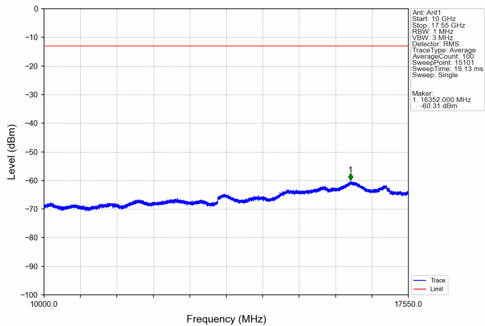
Band4_3MHz_16QAM_LCH_1711.5MHz_RB_1_0_NTNV
