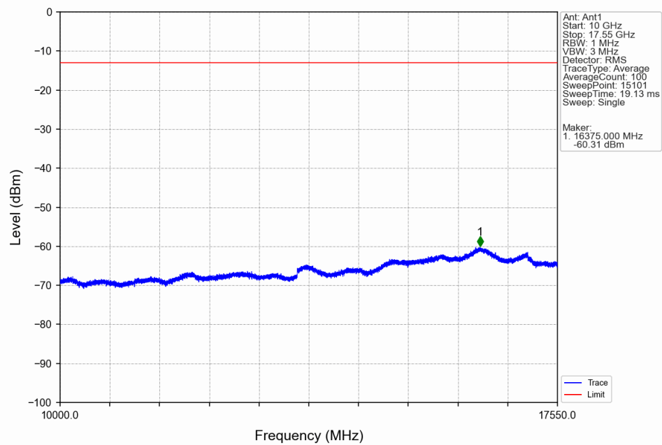
Band4_10MHz_16QAM_LCH_1715MHz_RB_1_0_NTNV
