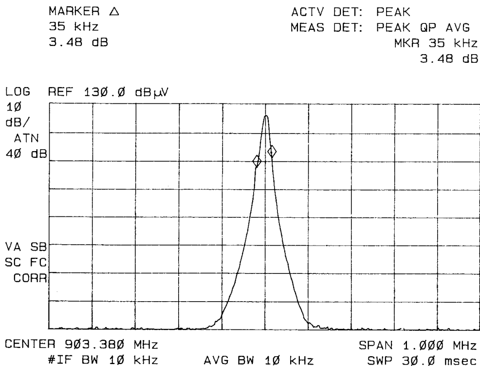
Figure 8 Antenna Conducted Emissions
