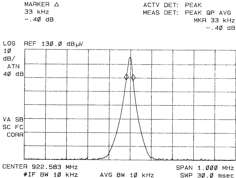
Figure 9 Antenna Conducted Emissions
