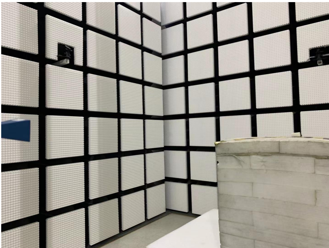
Radiated Emission Above 26.5-40GHz View
