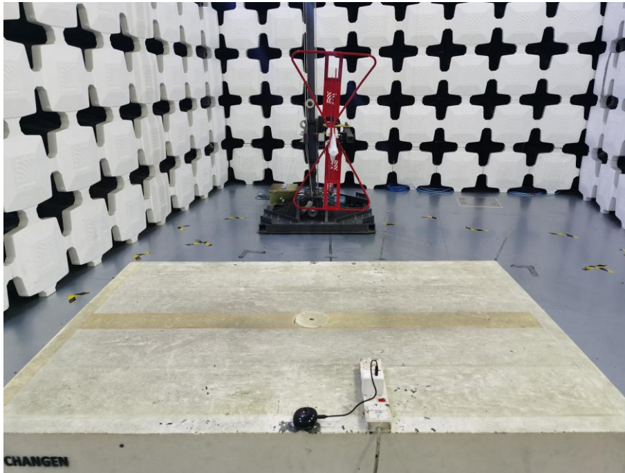
1. Radiated Emissions (Part 15B, Charging Mode, 30MHz-1GHz)
