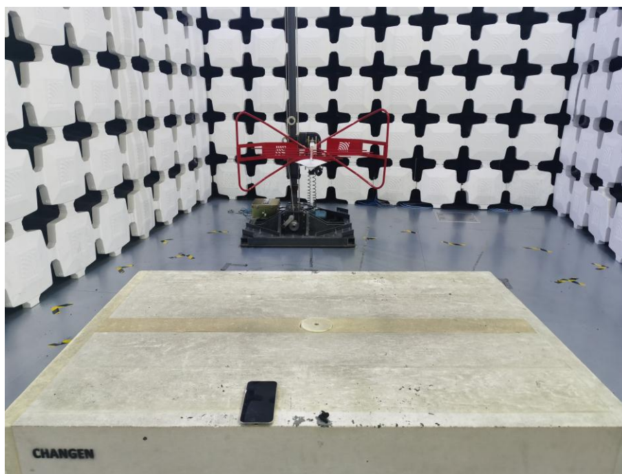
3. Radiated Emissions (Part 15B, Normal Working, 30MHz-1GHz)
