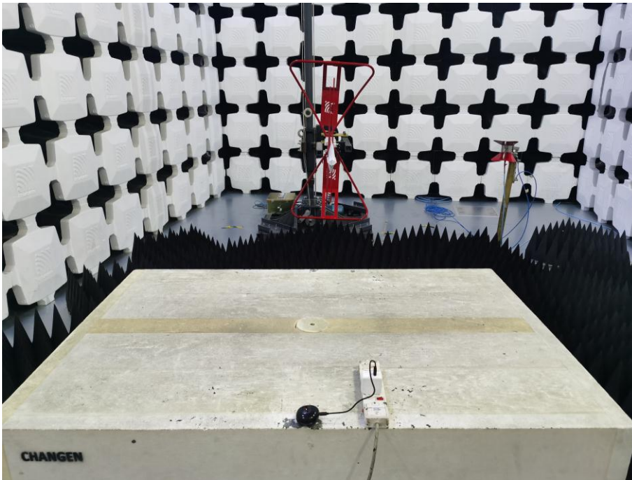
2. Radiated Emissions (Part 15B, Charging Mode 1GHz-18GHz)
