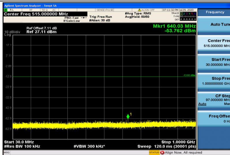
Band4-1.4MHz-16QAM-20175-1RB#0-30~1000MHz
