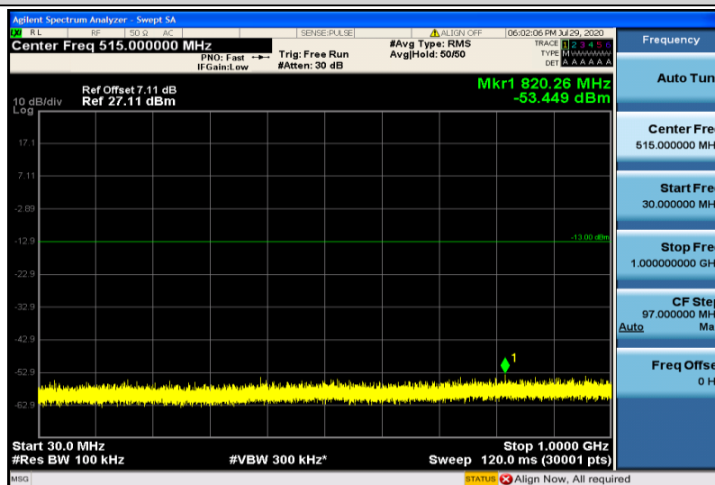
Band2-10MHz-QPSK-18900-1RB#0-30~1000MHz
