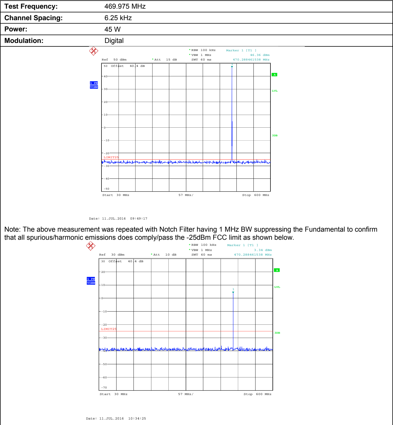
Plot 5.9.4.3.1. Conducted Transmitter Spurious Emissions for 469.975 MHz, High Power, 30 MHz - 600 MHz
