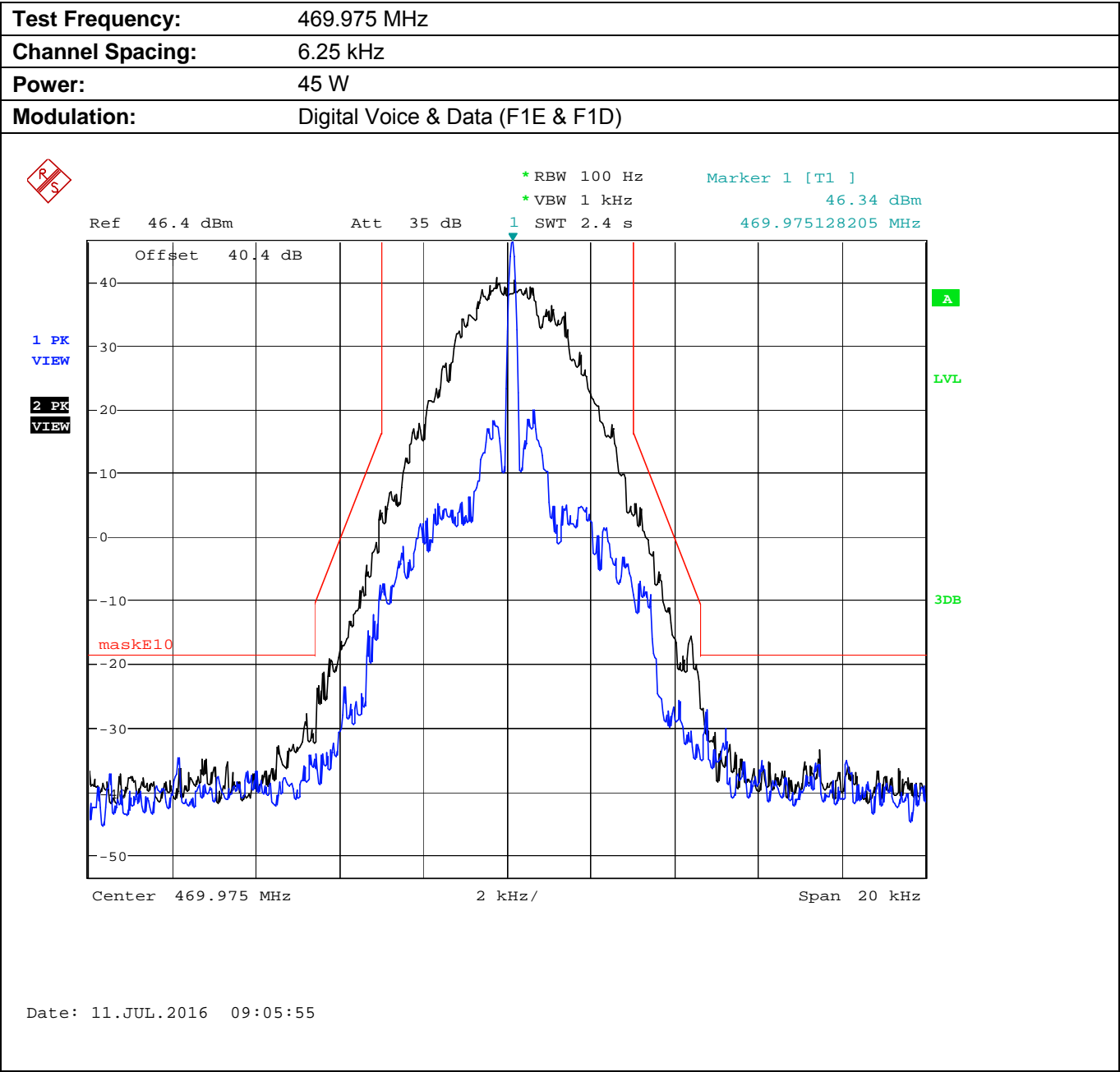
Plot 5.8.4.4.3. Emission Mask E, High Power
