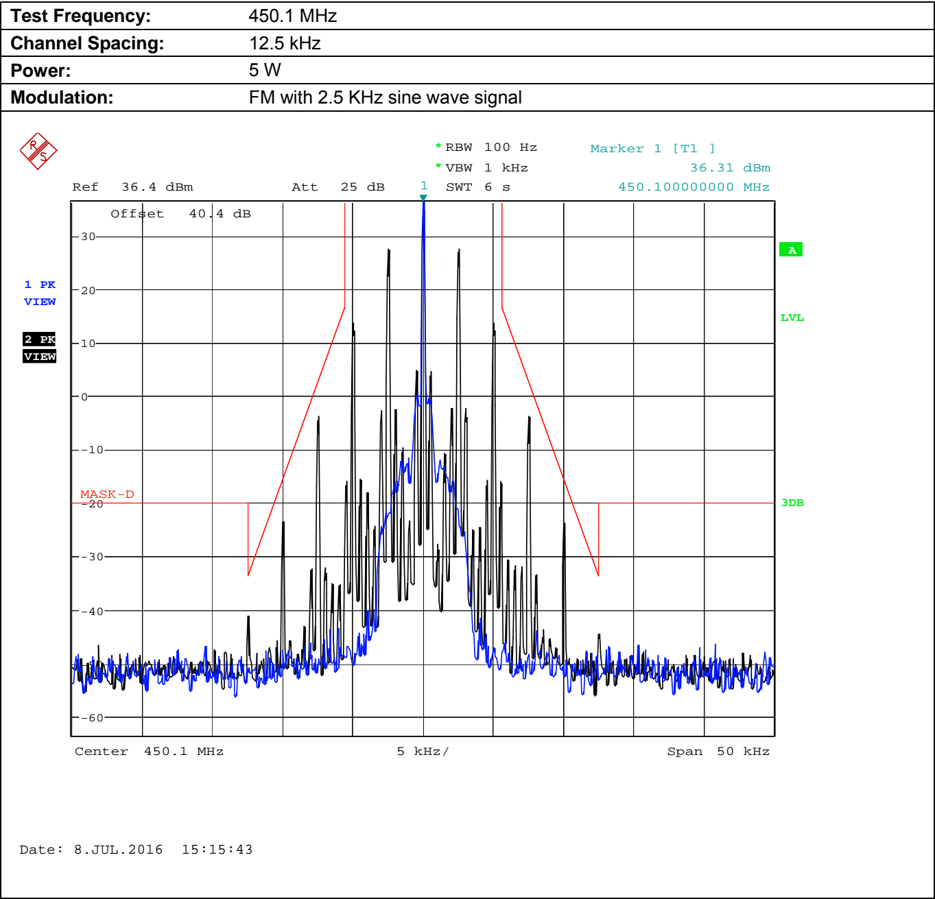
Plot 5.8.4.2.5. Emission Mask D, Low Power
