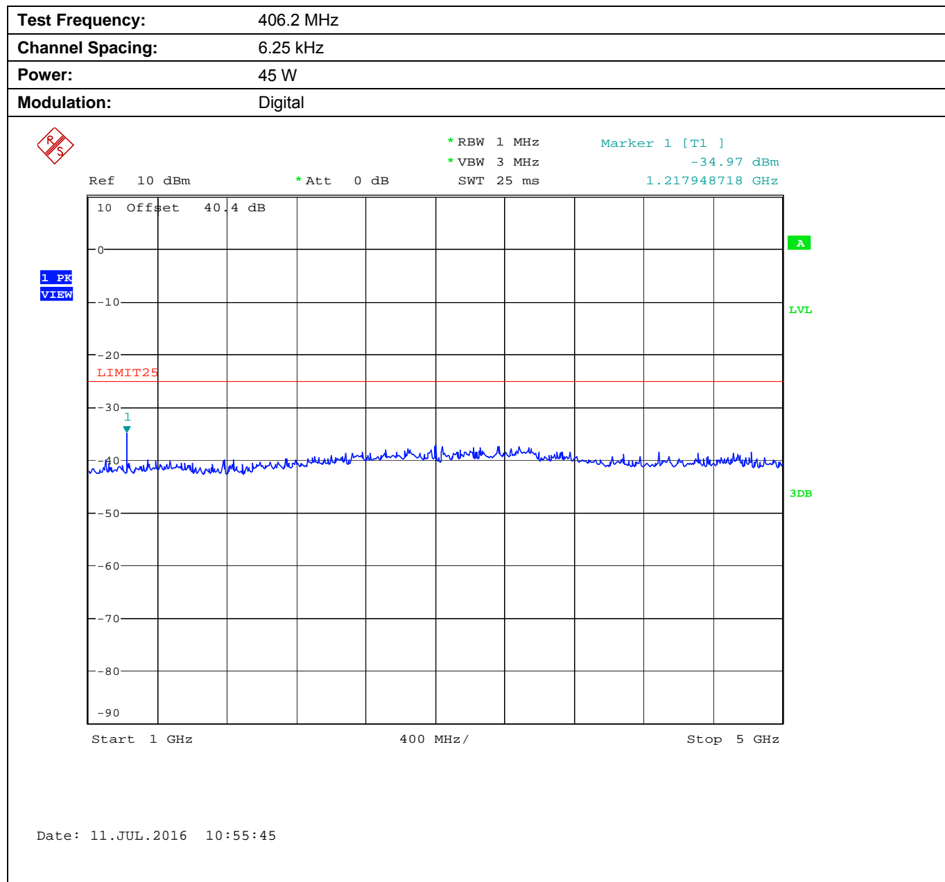
Plot 5.9.4.1.3. Conducted Transmitter Spurious Emissions for 406.2 MHz, High Power, 1 – 5 GHz
