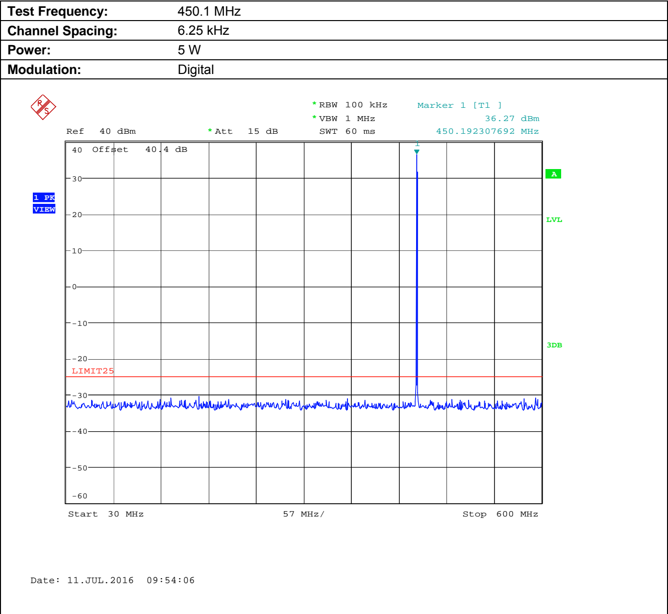
Plot 5.9.4.2.4. Conducted Transmitter Spurious Emissions for 450.1 MHz, Low Power, 30 MHz - 600 MHz
