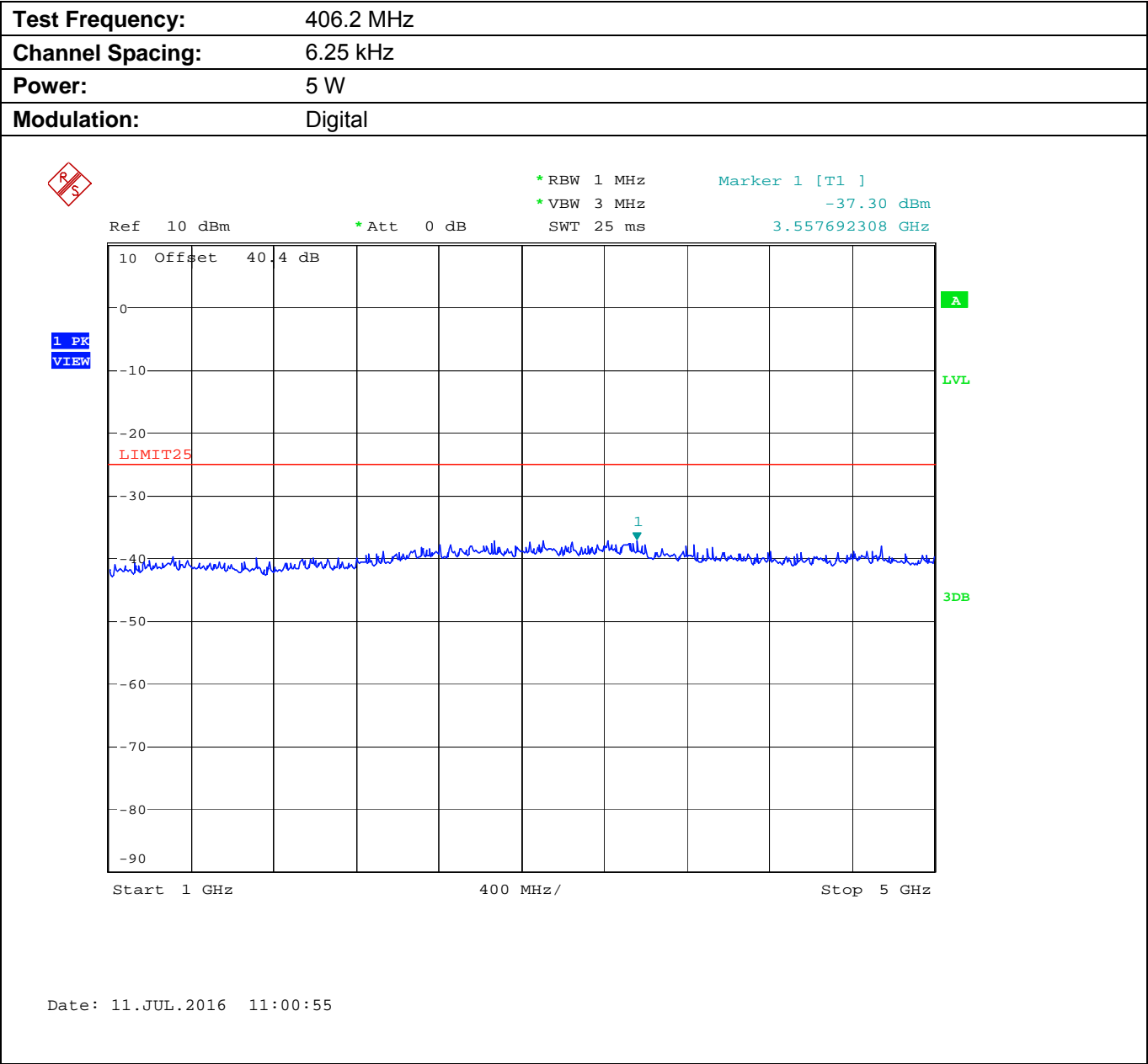
Plot 5.9.4.1.6. Conducted Transmitter Spurious Emissions for 406.2 MHz, Low Power, 1 - 5 GHz
