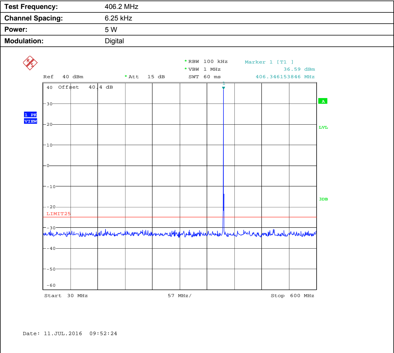
Plot 5.9.4.1.4. Conducted Transmitter Spurious Emissions for 406.2 MHz, Low Power, 30 MHz - 600 MHz
