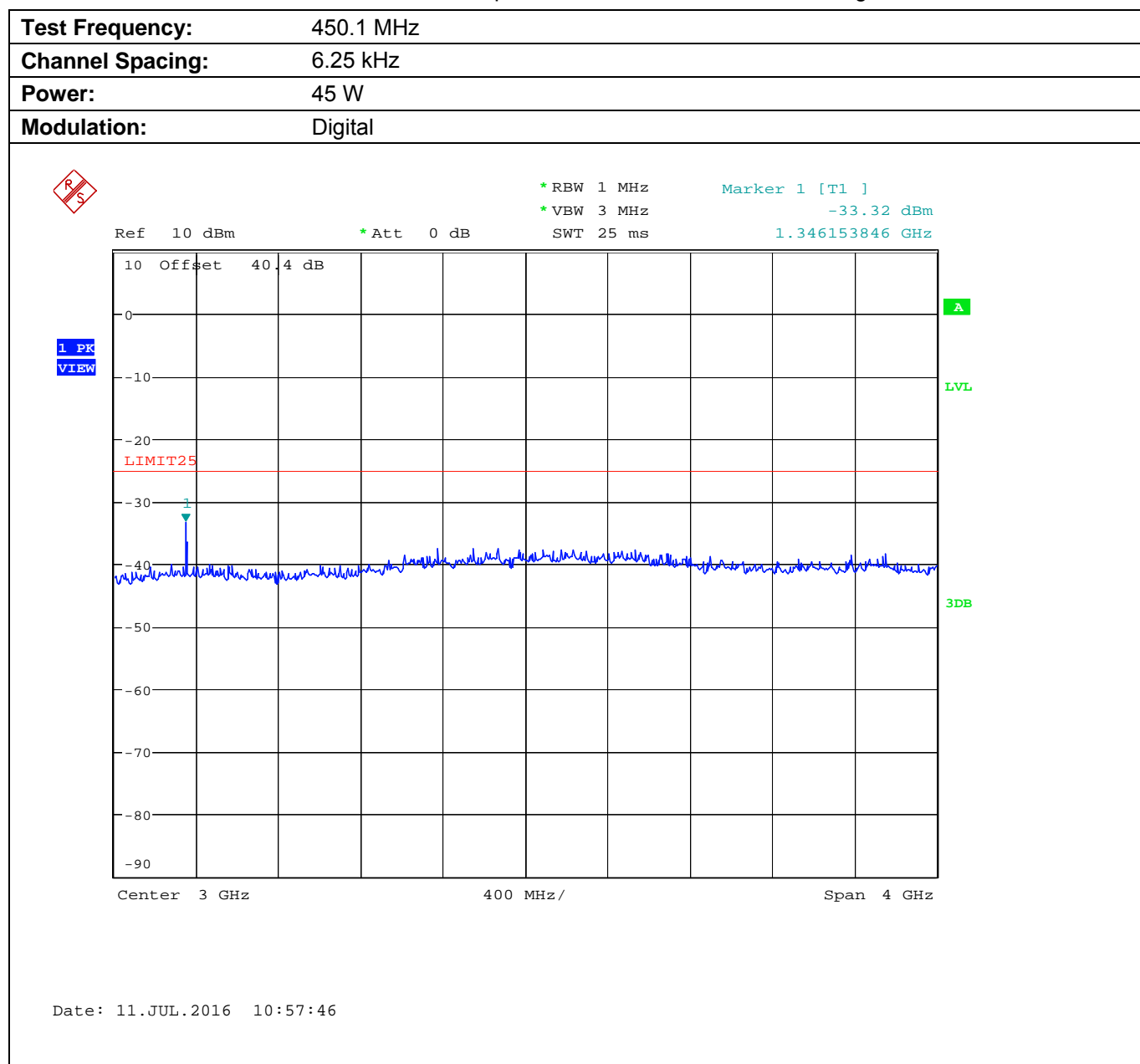
Plot 5.9.4.2.3. Conducted Transmitter Spurious Emissions for 450.1 MHz, High Power, 1 - 5 GHz
