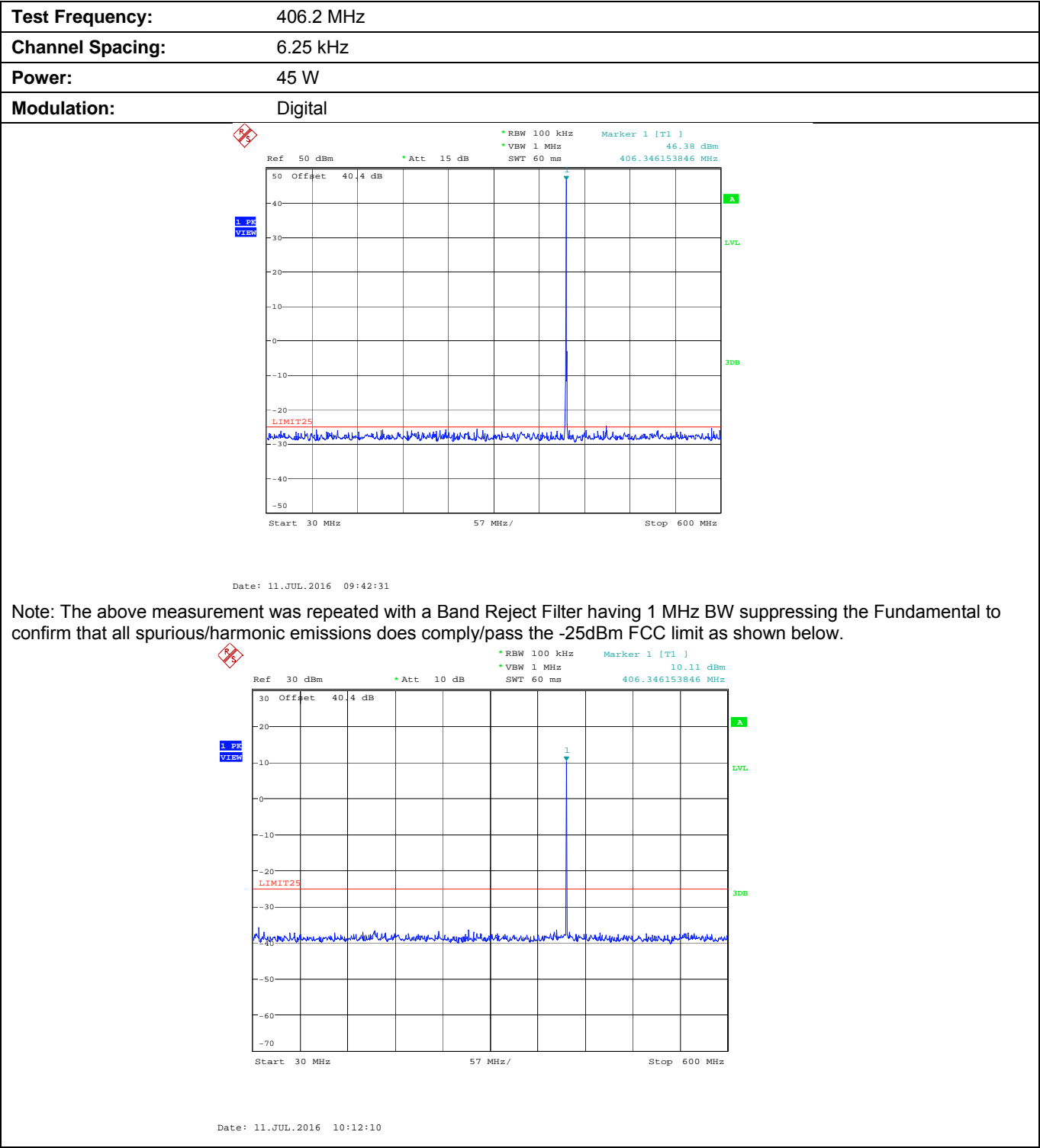
Plot 5.9.4.1.1. Conducted Transmitter Spurious Emissions for 406.2 MHz, High Power, 30 MHz - 600 MHz
