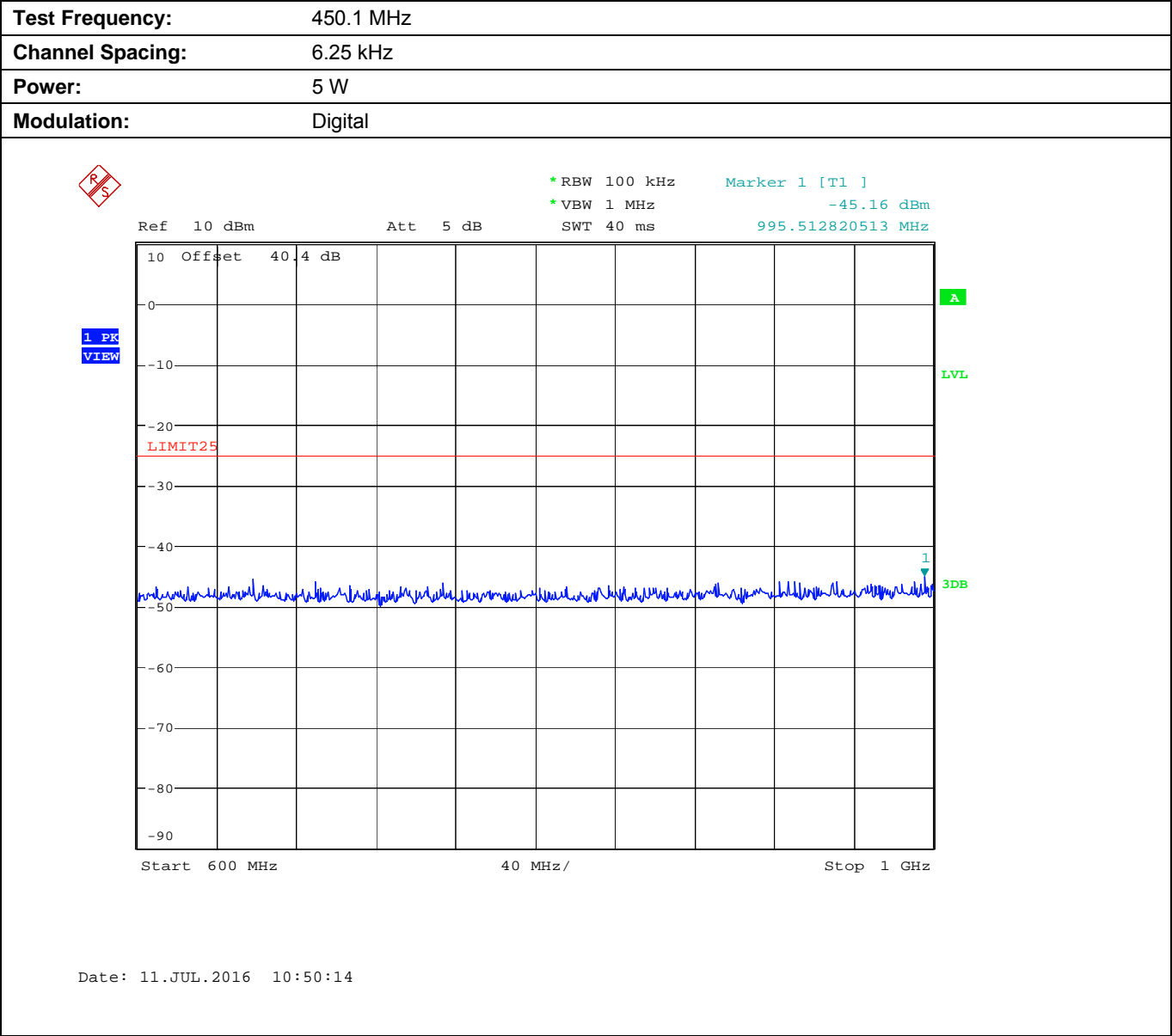
Plot 5.9.4.2.5. Conducted Transmitter Spurious Emissions for 450.1 MHz, Low Power, 600 MHz - 1 GHz
