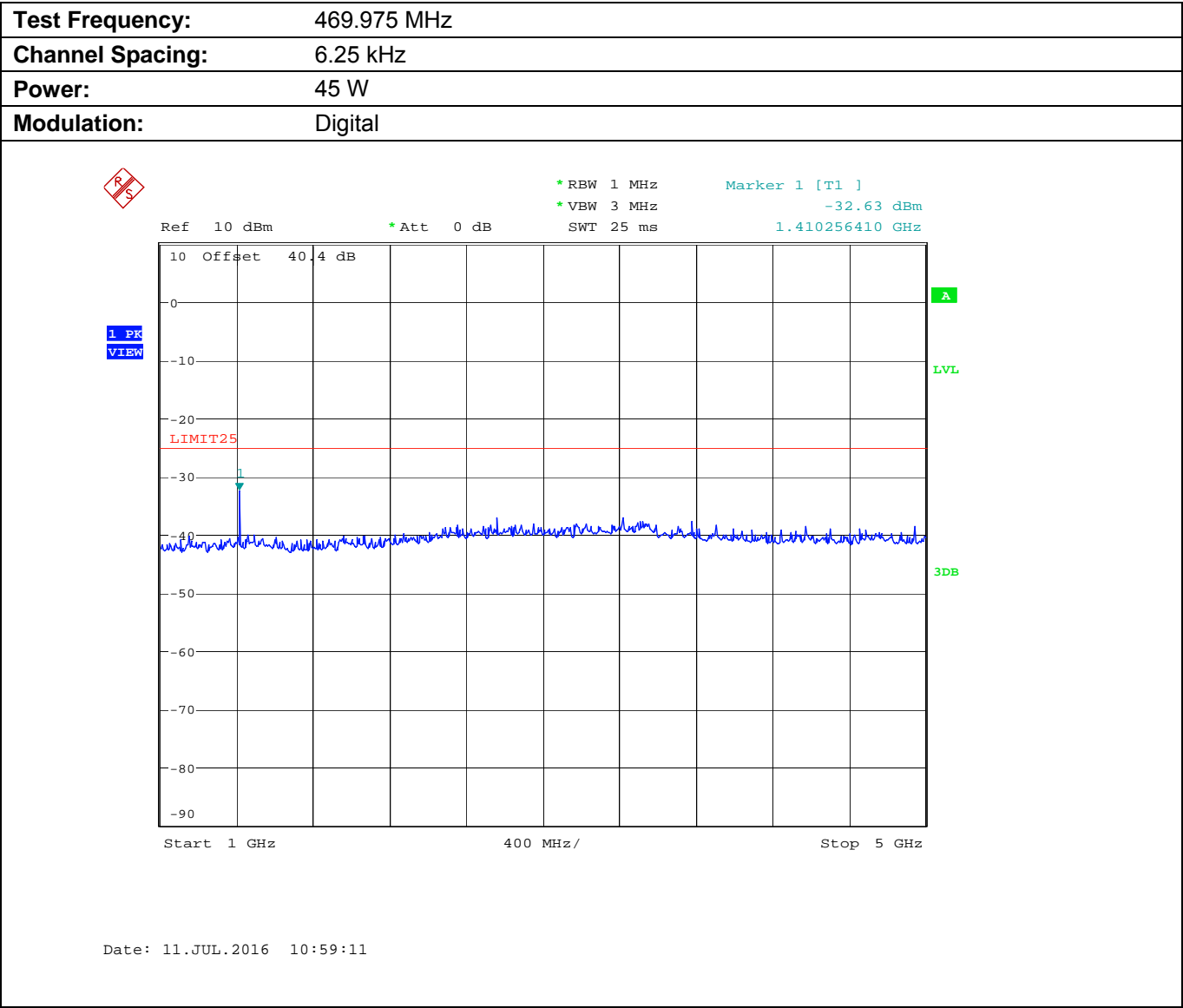
Plot 5.9.4.3.3. Conducted Transmitter Spurious Emissions for 469.975 MHz, High Power, 1 - 5 GHz
