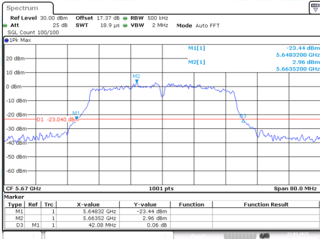
11AC40MIMO-Ant1-5670
