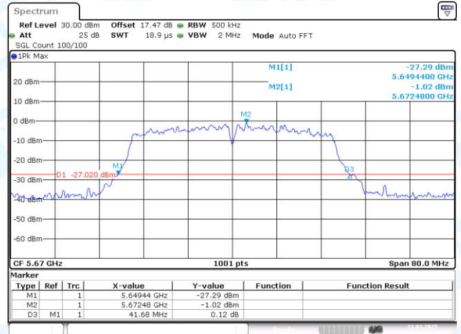
11AC40MIMO-Ant2-5670
