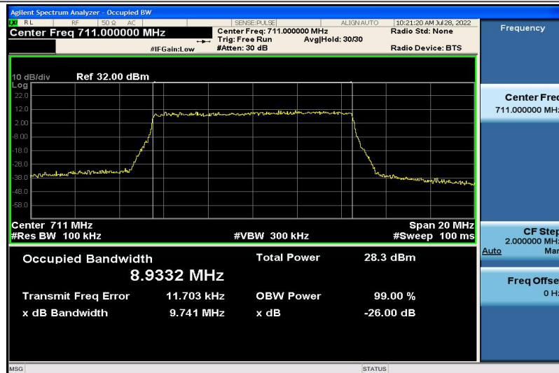
Band17-10MHz-16QAM-23800-50RB#0-8.9332
