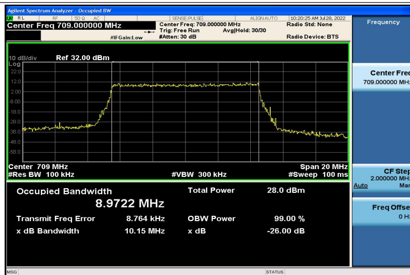
Band17-10MHz-QPSK-23780-50RB#0-8.9722
