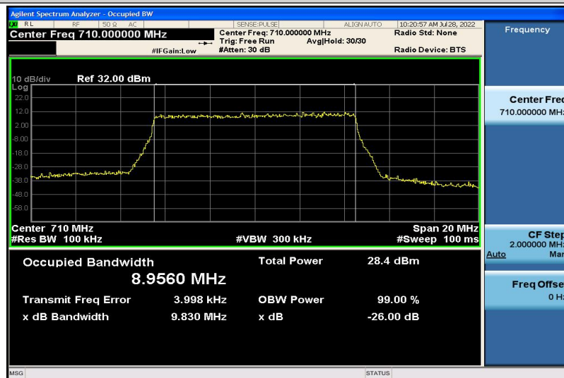
Band17-10MHz-16QAM-23790-50RB#0-8.9560
