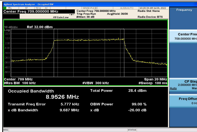
Band17-10MHz-16QAM-23780-50RB#0-8.9526
