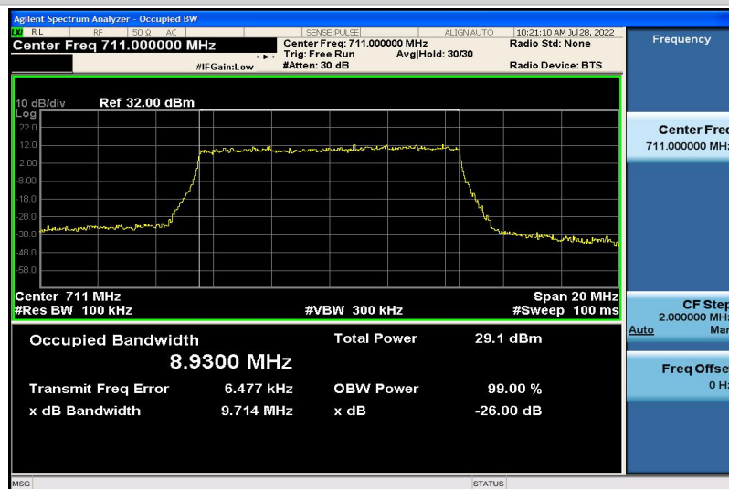
Band17-10MHz-QPSK-23800-50RB#0-8.9300
