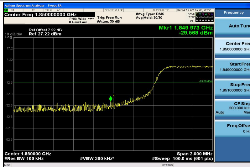
Band2-10MHz-16QAM-18650-50RB#0
