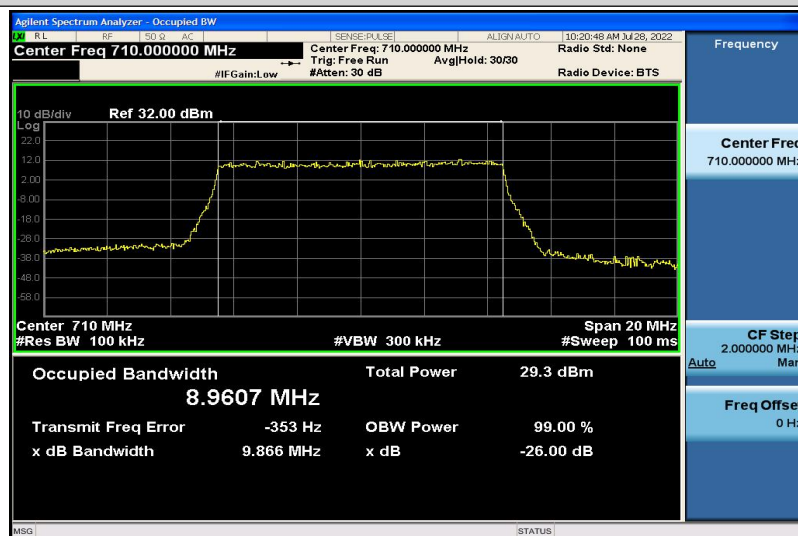
Band17-10MHz-QPSK-23790-50RB#0-8.9607
