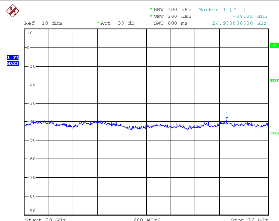
Plot 6 (20÷26GHz)
