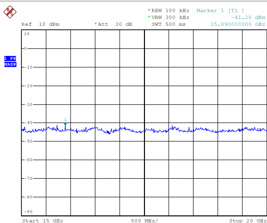
Plot 5 (15÷20GHz)
