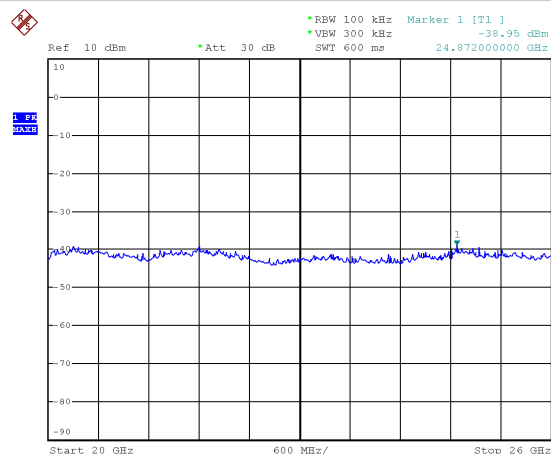
Plot 6 (20÷26GHz)
