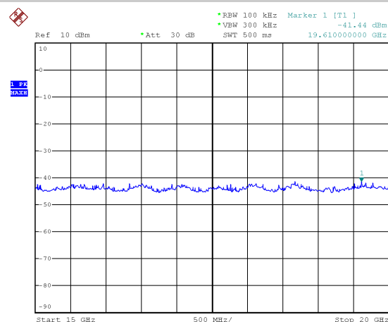
Plot 5 (15÷20GHz)
